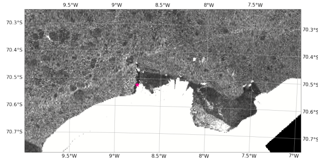
Figure A2. Sentinel-1 SAR image of the Ekström Ice Shelf and polynya on 12.01.2015 (PS89), zoomed in (ESA, 2021). The pink star indicates the sampling location for the PS89 tidal observation.
