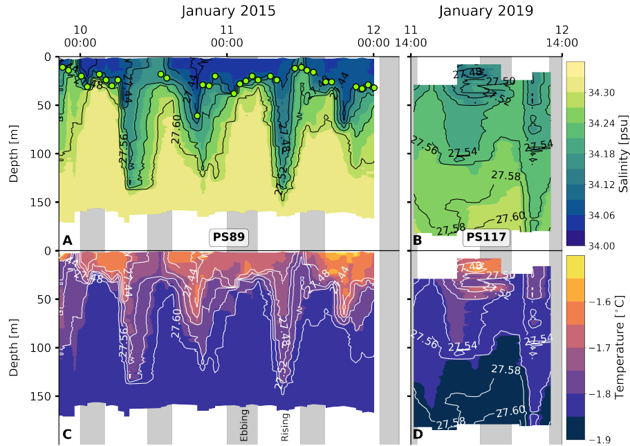
Figure 3. A and B show the salinity for PS89 and PS117, respectively. Green markers in A indicate the mixed layer depth (MLD) for casts where a mixed layer could clearly be identified according to a strong density gradient. MLD is identified as the depth at which the density difference with the average density values of the top 10 m is 0.03 \text{ kg m}^{-3} . Temperature profiles are shown in C (PS89) and D (PS117). White contour lines represent isopycnals in \text{kg m}^{-3} . Vertical grey shaded areas indicate times of ebbing tide.
