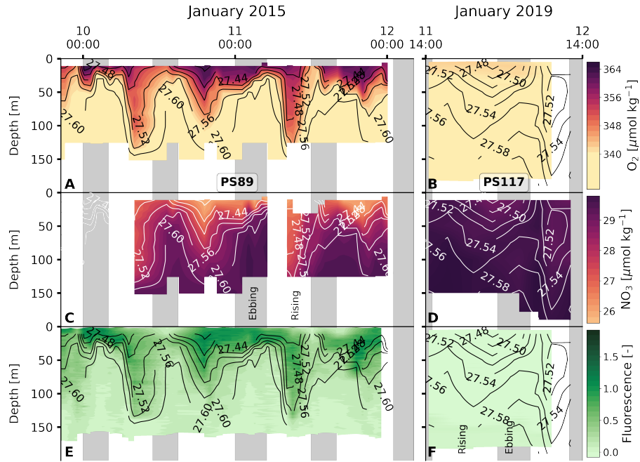
Figure 6. Same as Fig. 3, but for dissolved O_2 (A and B), NO_3^- (C and D), and fluorescence (E and F). Fluorescence during PS117 varied at values < 0.09 .
