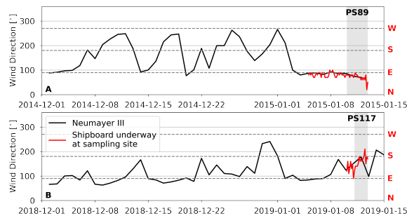
Figure H2. A) Wind direction measured at Neumayer III Research Station in the time prior and during the PS89 tidal observation (black), as well as the ship-board wind direction measurements during the PS89 tidal observation (red). B) Wind direction measured at Neumayer III Research Station in the time prior and during the PS117 tidal observation (black), as well as the ship-board wind direction measurements during the PS117 tidal observation (red). Grey areas indicate the duration of the tidal observations. Horizontal dashed lines indicate 90^\circ , 180^\circ , and 270^\circ . North, East, South, and West directions are indicated by the red initials at the right side of the plots.
