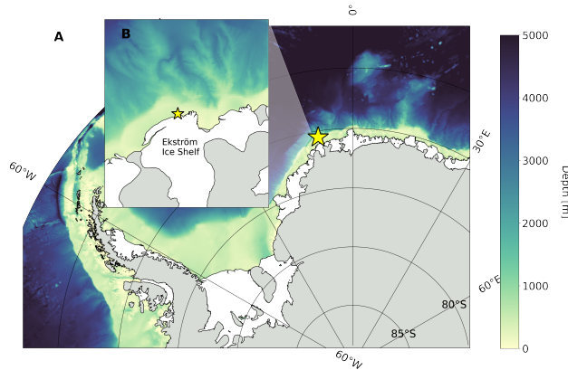
Figure 1. Map of study site: A) Weddell Sea with bathymetry: IBSCO Version 1.0 (Arndt et al., 2013). Grey regions represent the Antarctic continent and land-fast ice, white regions represent ice shelves. B) Enlarged map of coastal study site along the Ekström Ice Shelf. Yellow star shows location of tidal measurements. See Table 1 for coordinates.
