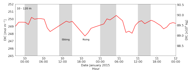
Figure G3. Left y axis: total water column DIC content between 10 and 120 m during the PS89 tidal observation. Right y axis: total DIC content between 10 and 120 m for the entire PS89 polynya, using the estimated dimensions in the text and assuming an ellipsoidal area.
