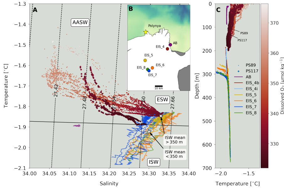
Figure 7. A) Temperature-salinity diagram for PS89 (circles) and PS117 (diamonds) tidal observation periods, which are coloured according to dissolved oxygen concentrations. CTD profiles of the ice shelf's cavity water were collected and made available by Smith et al. (2020a) (coloured lines). The cavity CTD profiles were taken by hot water drilling through the ice at various locations on the ice shelf, which are shown on the map in (B) in corresponding colours to the profiles in (A). AASW = Antarctic Surface Water, ESW = Eastern Shelf Water, ISW = Ice Shelf Water. The average temperature and salinity of water deeper and shallower than 350 m underneath the ice shelf are plotted as single white crosses. Contour lines indicate sigma-t in \text{kg m}^{-3} . Black line indicates freezing point at mean atmospheric pressure. B) Map of measurement locations of the Ekström Ice Shelf cavity CTD profiles by Smith et al. (2020a) denoted by "EIS_", a measurement location in Atka Bay by Smith et al. (2020a) denoted with "AB", and the sampling location of the tidal observations indicated by the yellow star. C) Temperature profiles for PS89 (circles) and PS117 (diamonds) tidal observation periods, coloured according to oxygen concentrations, and for the hot water drill CTD profiles underneath the ice shelf from Smith et al. (2020a).
