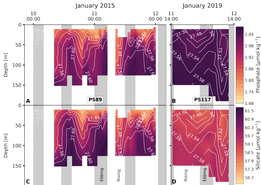
Figure G2. As for Fig. G1, but instead for phosphate and silicate content and not including the pH and calcite saturation contours that are shown in Fig. G1.
