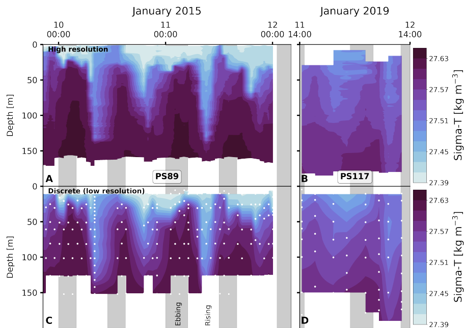
Figure E1. A) High vertical resolution profile of sigma-t for PS89. B) High vertical resolution profile of sigma-t for PS117. C) Discrete (low vertical resolution) profile measurements at bottle sampling depth for PS89. D) Discrete (low vertical resolution) profile measurements at bottle sampling depth for PS117. Sampling depths are shown in white markers in C and D.
