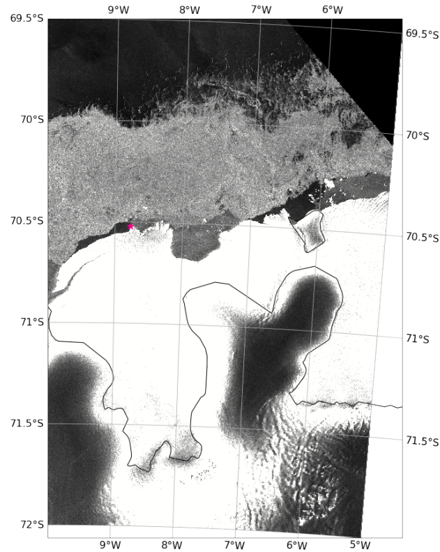
Figure A3. Sentinel-1 SAR image of the Ekström Ice Shelf and polynya on 10.01.2019 (PS117) (ESA, 2021). The pink star indicates the sampling location for the PS117 tidal observation.
