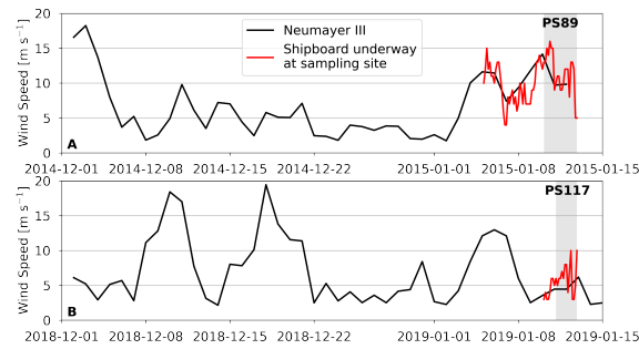
Figure H1. A) Wind speed measured at Neumayer III Research Station (black) in the time prior and during the PS89 tidal observation, as well as the ship-board wind speed measurements during the PS89 tidal observation (red). B) Wind speed measured at Neumayer III Research Station in the time prior and during the PS117 tidal observation (black), as well as the ship-board wind speed measurements during the PS117 tidal observation (red). Grey areas indicate the duration of the tidal observations.
