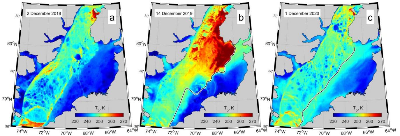
Figure 10: MODIS near -clear-sky brightness temperatures on (a) 02 December 2018, (b) 14 December 2019 and (c) 01 December 2020. Images (b) and (c) show T_b several days prior to ice bridge formations in both years.
