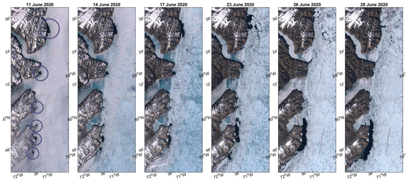
Figure 1211: The series of Sentinel-2 images showing the evolution of polynyas along western coast of Kane Basin from the first appearance until the start of bridge collapse in June 2020. The circles in the left panel indicates the regions where open water polynyas first appear.
