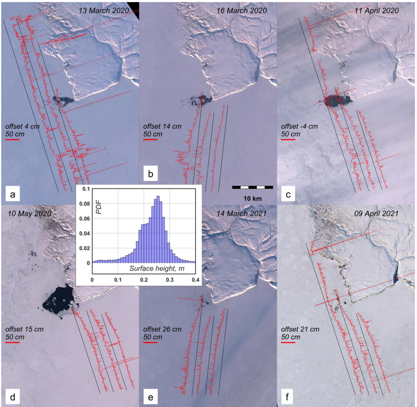
Figure 3: The ATL07 elevations (red lines) heights from 3 strong beams overlaid on the Sentinel-2 images of the polynya in March-May 2020 and in March-April 2021. The elevations are adjusted to the sea level in the polynya and plotted as absolute deviations from the ground tracks (black lines) in direction normal to the tracks. The open water was used as a reference level to calculate the corresponding offsets for each subset. The red scale bar in each panel corresponds to 50 cm elevation. The inset histogram demonstrates the probability distribution of all heights shown in the panels a-f.
