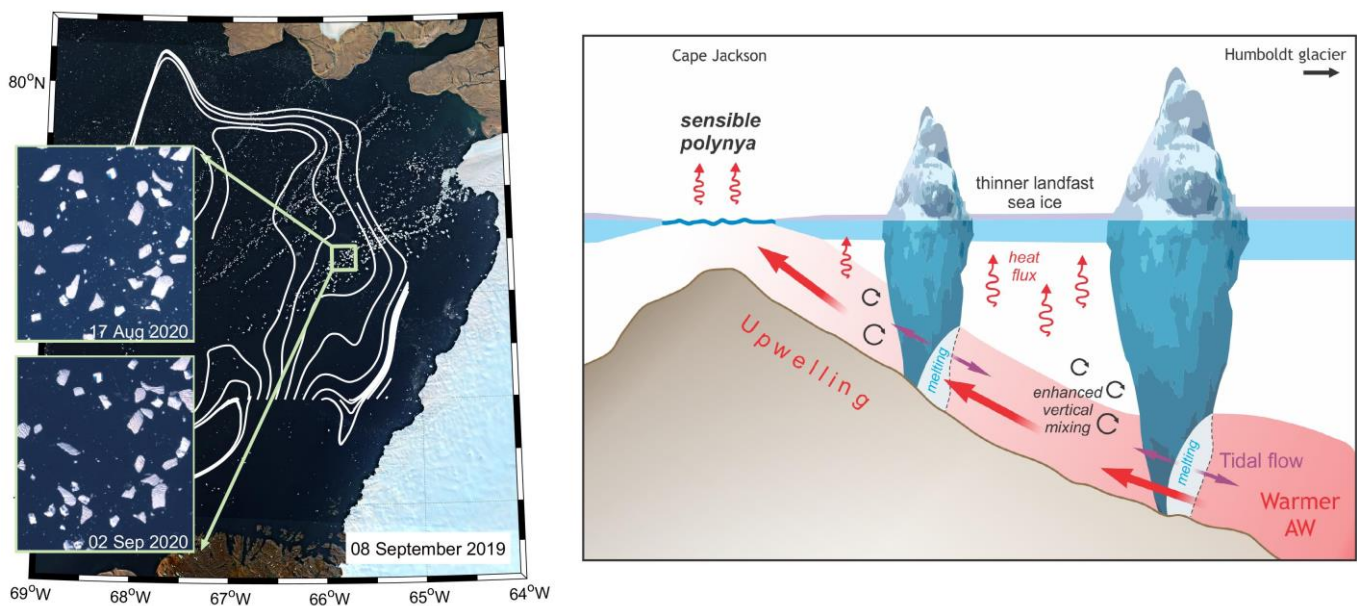
525 Figure 11: (left) The grounded icebergs in Peabody Bay. The white trajectories represent the mean November-June ocean circulation at 80 m depth from FESOM model. (right) The principle scheme of interaction of AW with a slope and grounded icebergs.
