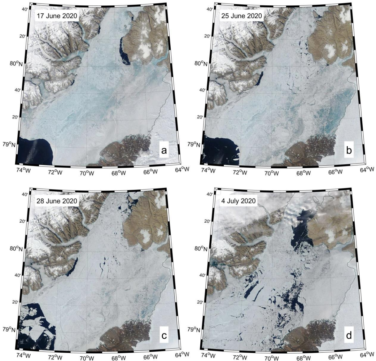
Figure 1413: The process of the ice bridge break-up in June 2020 in MODIS true-color imagery.
