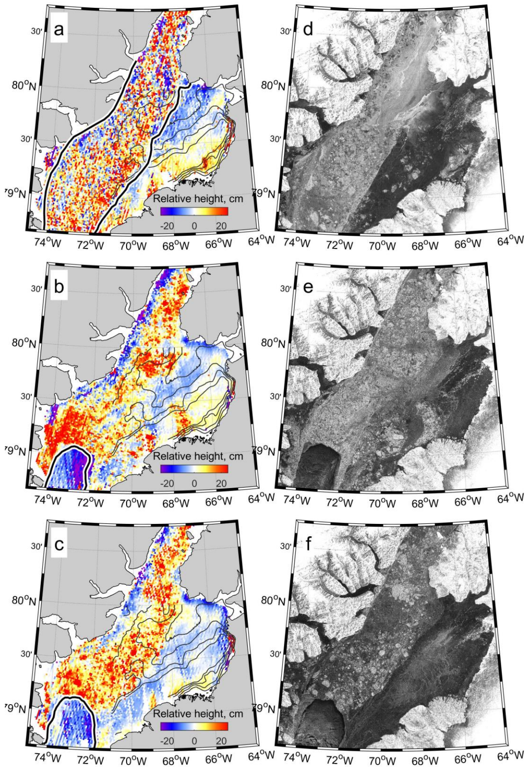
Figure 4: (a-c) The along-track anomalies of ATL07 heights-elevations averaged over 1.5x1.5 km cells in January-April 2019 (a), 2020 (b) and 2021 (c). The thick black lines correspond to approximate positions of landfast ice edge during these winters. (d-e) Sentinel-1 SAR images from January 16 in the corresponding years.
