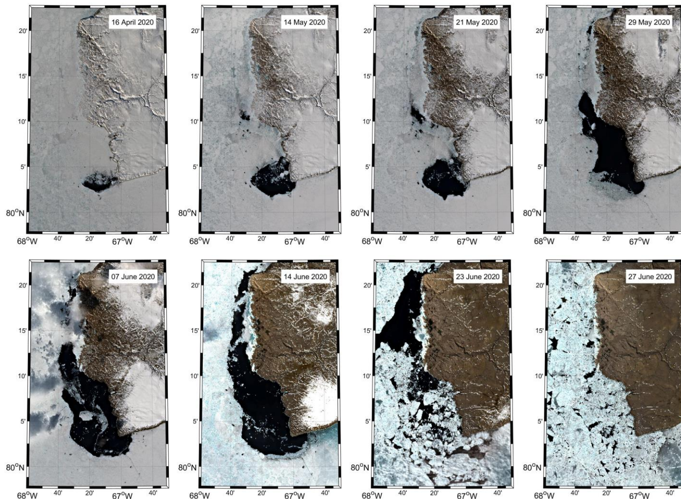
645 Figure 1312: The evolution of polynya at Cape Jackson from April to June 2020 from Sentinel-2 data.
