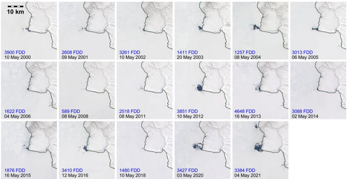
240 Figure 2: The presence of sensible heat polynya at Cape Jackson during winters when ice bridge in Nares Strait formed between 2000 and 2021 in MODIS imagery. Blue numbers correspond to the sum of freezing degree days (FDD) from a corresponding date of bridge formation (see Kirillov et al., 2021) to 30 April. Each panel is 37.5 x 37.5 km.
