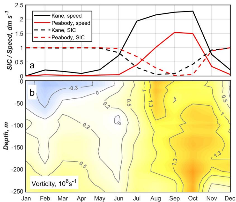
425 Figure 8: (a) The mean monthly SIC (dashed lines) and drift speeds (solid lines) within the main channel of Kane Basin (black) and in Peabody Bay (red). (b) The seasonal evolution of mean 2006-2010 vorticity within Peabody Bay. Both datasets are calculated from FESOM data.
