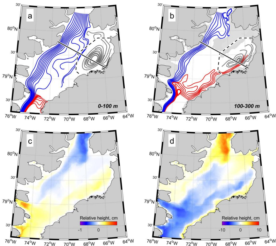
400 Figure 7: (a-b) The trajectories of water parcels calculated from the mean 2006-2010 model current velocities averaged within 0-100 m and 100-300 m, respectively. The blue, red and green-grey lines correspond to three main circulation patterns in the region (see more details in the text). The black dashed line envelopes the region used for vorticity calculation (Figure 8) and the solid line shows the position of transect presented in Figure 9. The shaded area in panel (b) corresponds to the regions shallower than 150 m. The spatial distribution of the mean winter (November-June) thermo- and halosteric sea-level anomalies is shown in (c) and (d), respectively.
