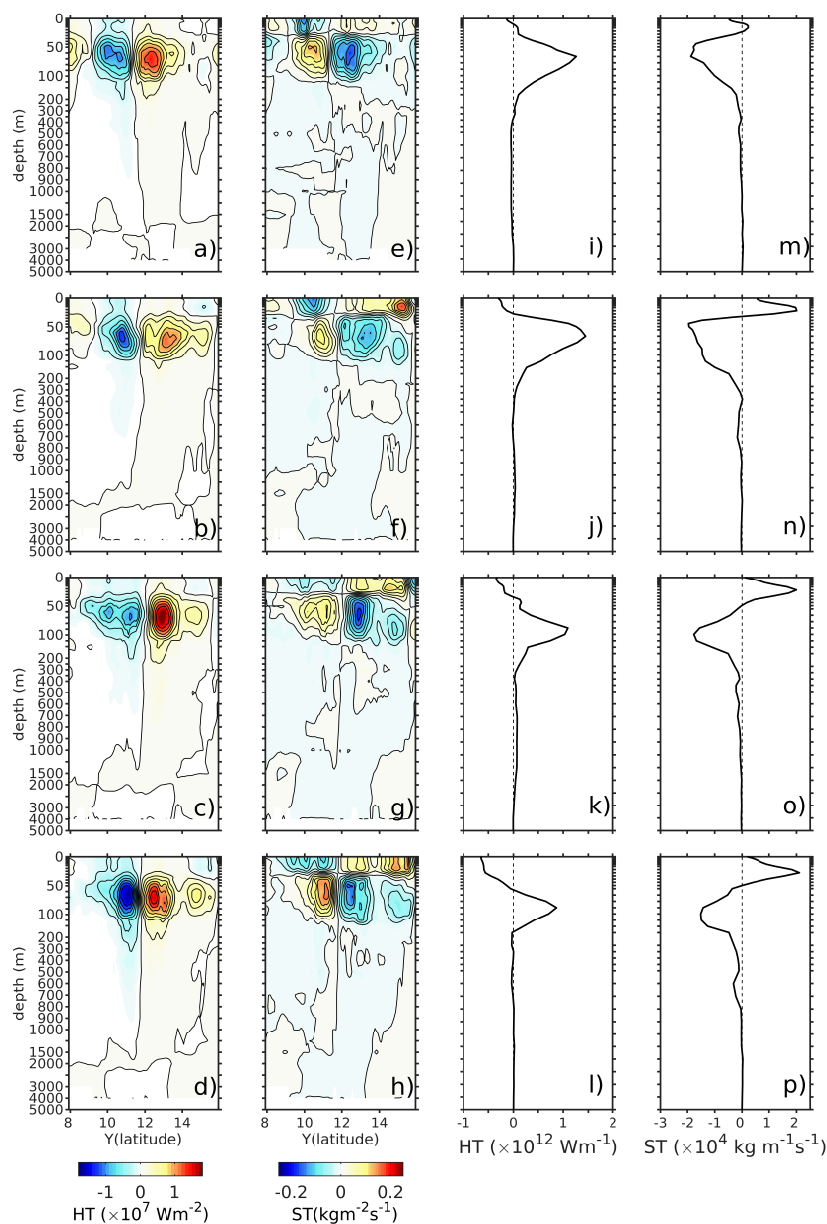
Figure 12. Vertical sections of heat flux a) to d) and salinity flux e) to h). Vertical profiles of heat transport integrated across the eddy area i) to l) and vertical profile of salinity transport m) to p). Each row from top to bottom show the transects in 03 April, 27 April, 11 May and 16 May 2019 respectively.
