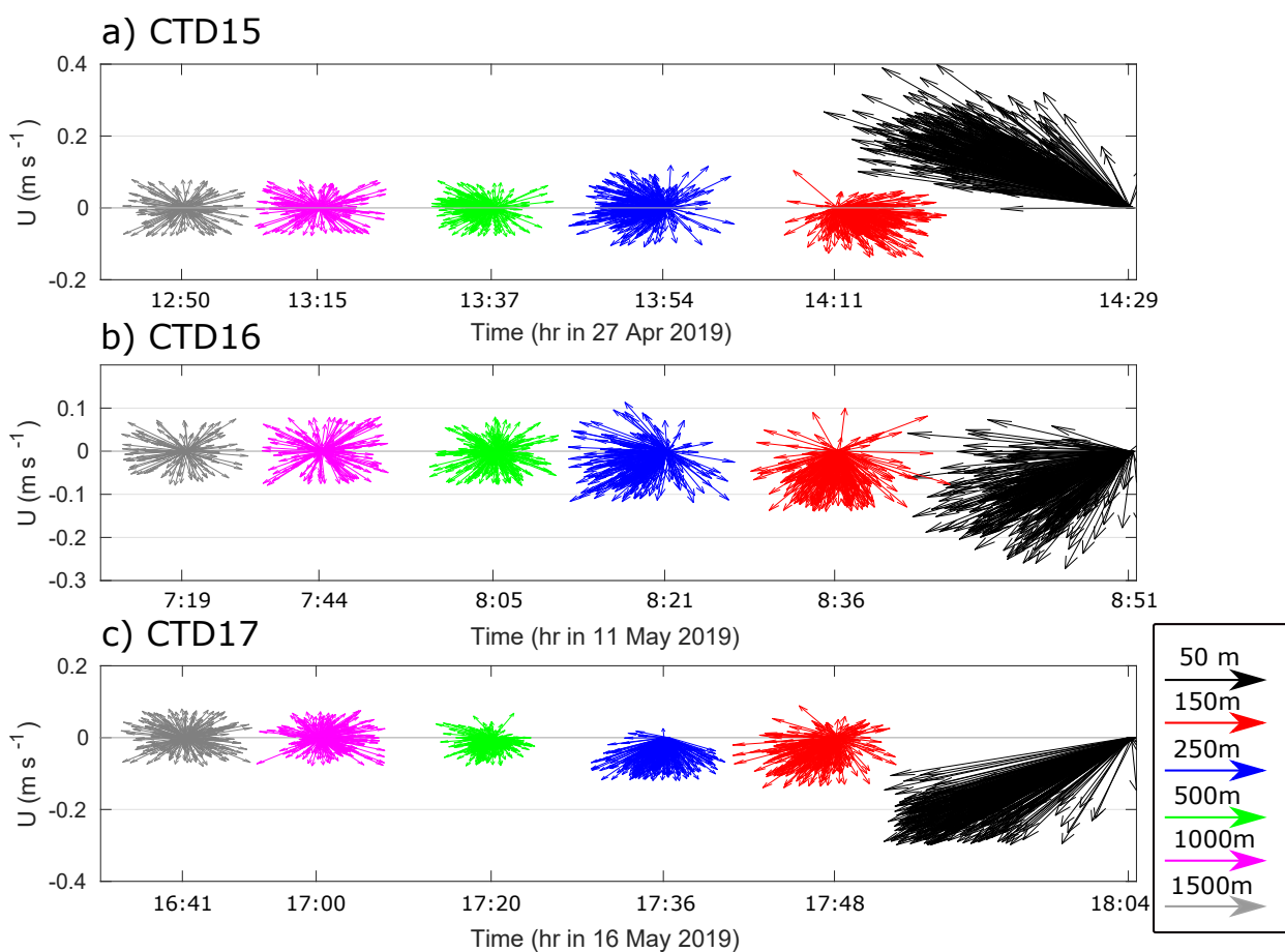
Figure 9. Current velocity obtained at the western rim, eddy center and eastern rim of the taken at different depths from an Aquadoppe attached to the CTD at a) 27 April 2019, b) 11 May 2019 and c) 16 May 2019. Different colors correspond to the measurements at distinct depths.
