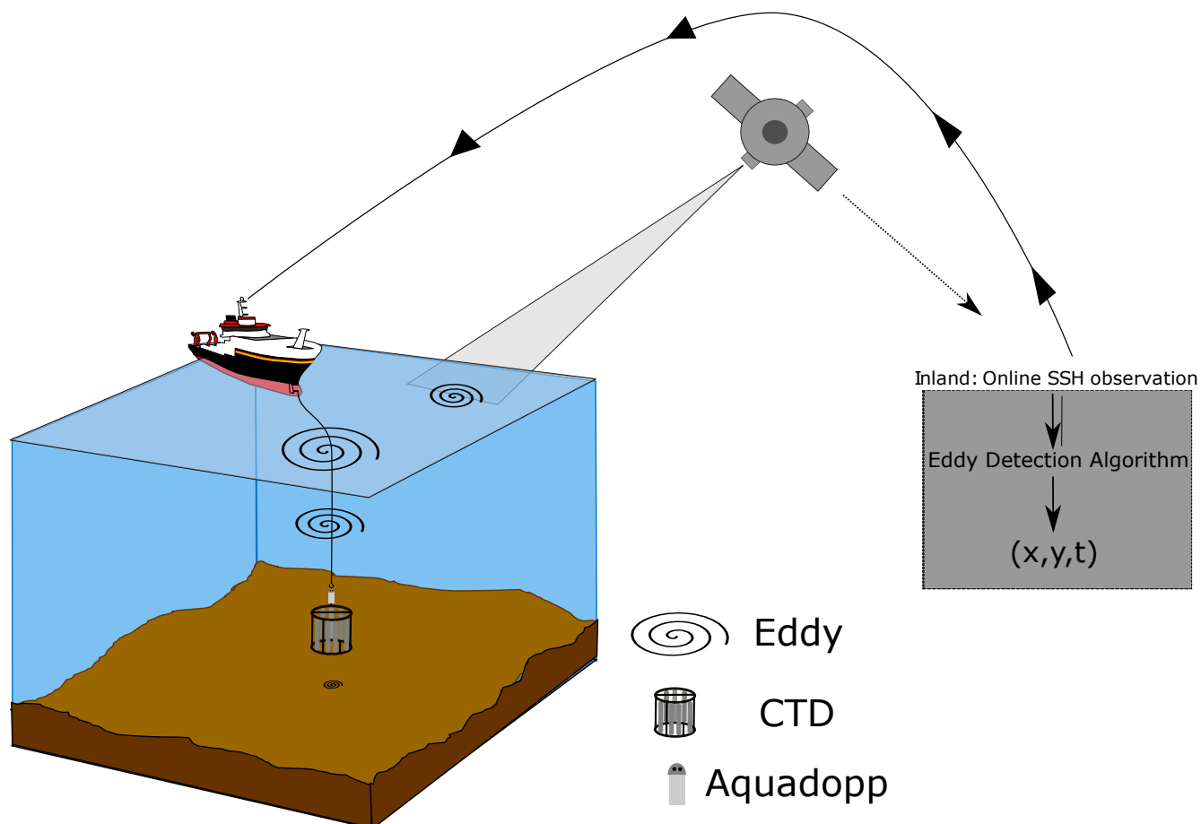
Figure 2. The concept of online communication between the research vessel in the NETP and the shore-based eddy detection group using online satellite data for determining the positions for hydrographic measurements. Figure is not to scale. Eddy, CTD and Aquadopp are shown.
