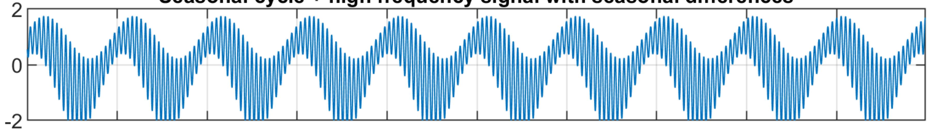
Seasonal cycle + high frequency signal with seasonal differences
