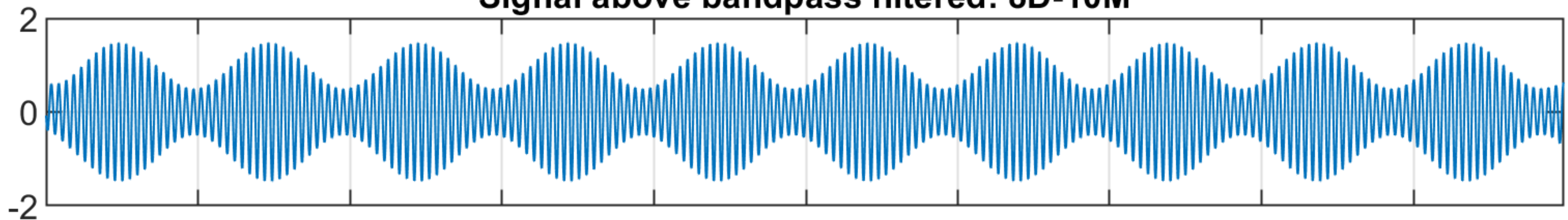
Signal above bandpass filtered: 8D-10M
