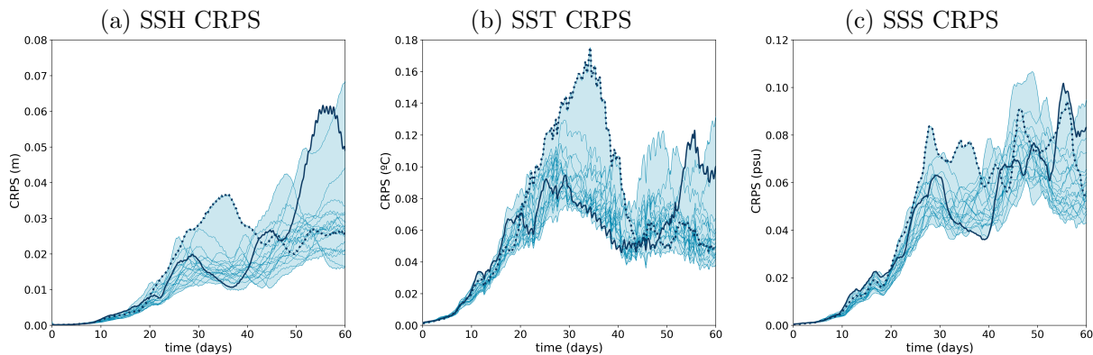
Figure 8. Time evolution of the CRPS score (y-axis) for SSH (meters), SST (degree Celsius) and SSS (psu) from experiment ENS-CI. The score is computed for each of the 20 permuted cases (thin lines) taking an ensemble member as the reference truth and the rest of the members as the ensemble forecast. The blue shading represents the min-to-max envelop of the 20 scores computed for the experiments. Two example lines are plotted thicker (solid and dotted lines) in each panel to illustrate how individual scores can evolve with time.
