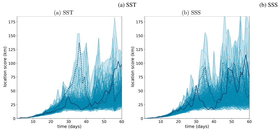
Figure 14. Time evolution of the location score (y-axis, in km) for (a) SST and (b) SSS in experiment ENS-CI. The score is computed for each of the 20x19 permuted pairs (blue lines) considering one ensemble member as the reference truth and each of the 19 remaining ensemble members as a forecast. The blue shading represents the min-to-max envelop of all the 20x19 scores computed for the experiment. Two example lines are plotted thicker (solid and dotted lines) in each panel to illustrate how individual scores can evolve with time.
