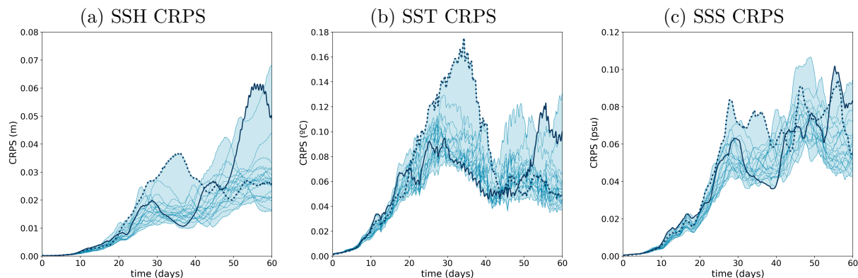
Figure 8. Time evolution of the CRPS score ( y -axis) for SSH (meters), SST (degree Celsius) and SSS (psu) from experiment ENS-CI. The score is computed for each of the 20 permuted cases (thin lines) taking an ensemble member as the reference truth and the rest of the members as the ensemble forecast. The blue shading represents the min-to-max envelop of the 20 scores computed for the experiments. Two example lines are plotted thicker (solid and dotted lines) in each panel to illustrate how individual scores can evolve with time.
