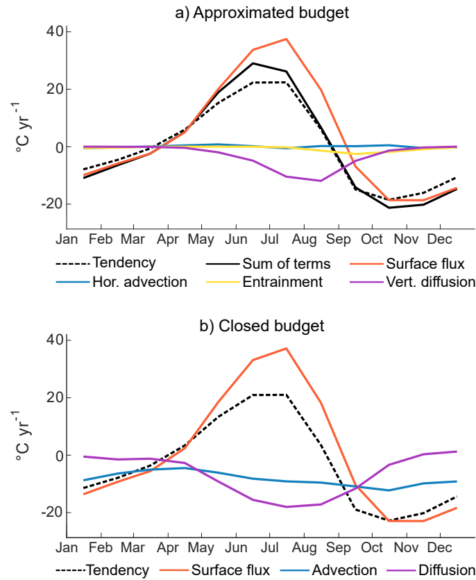
Figure 5. The average seasonal cycle of the dominant mixed layer temperature budget terms ( ^{\circ}\text{C yr}^{-1} ) averaged over the cold blob region for ECCOv4-r4, where positive values represent an increase in the rate of change in the temperature of the mixed layer. a) The approximated budget computed using Equation 1, where the black dashed line is the actual temperature tendency in the model, and the solid line is the sum of the budget terms driving that temperature change. The remaining lines represent the temperature change due to each individual process: surface heat fluxes (orange), horizontal advection (blue), vertical entrainment (yellow), and vertical diffusion (purple). Horizontal diffusion and lateral induction are not shown as the effects of both are negligible. b) The closed budget computed online for comparison, where the dashed line is the tendency, which is equal to the sum of surface fluxes (orange), advection (blue), and diffusion (purple).
