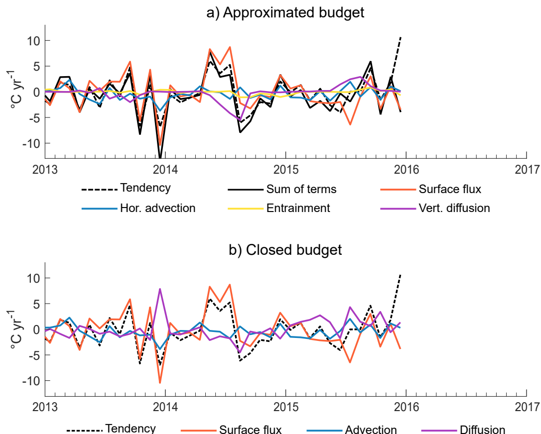
Figure B4. Anomalies in the dominant terms of the mixed layer temperature budget, relative to the 1992–2015 monthly climatology ( ^{\circ}\text{C yr}^{-1} ), averaged over the cold blob region. a) Anomalies in the approximated budget, where the dashed black line shows anomalies in the model temperature tendency, and the solid black line shows anomalies in the sum of the temperature budget terms driving the temperature change. The remaining lines represent those individual processes: the surface heat flux (orange), horizontal advection (blue), vertical entrainment (yellow), and vertical diffusion (purple). Lateral induction and horizontal diffusion are not shown because anomalies in both are negligible. b) Anomalies in the closed budget.
