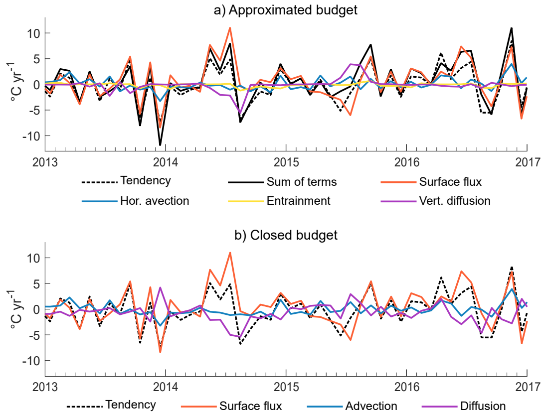
Figure 6. a) Anomalies in the dominant terms of the mixed layer temperature budget, relative to the 1992-2015 monthly climatology ( ^{\circ}\text{C yr}^{-1} ), averaged over the cold blob region. a) The approximated budget computed via Equation 1, where the dashed black line shows anomalies in the model temperature tendency and the solid black line shows anomalies in the sum of the temperature budget terms driving the temperature change. The remaining lines represent those individual processes: the surface heat flux (orange), horizontal advection (blue), vertical entrainment (yellow), and vertical diffusion (purple). The budget is also shown in Fig. A1, prior to the removal of the seasonal cycle. b) Anomalies in the closed budget for comparison.
