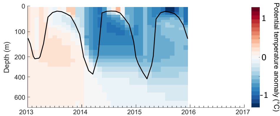
Figure B2. The potential temperature anomaly over depth relative to the 1992-2015 monthly climatology (color; °C), averaged over the cold blob region in ECCOv4-r3. The MLD is also shown (black line, m). Note the non-uniform spacing of the vertical axes.
