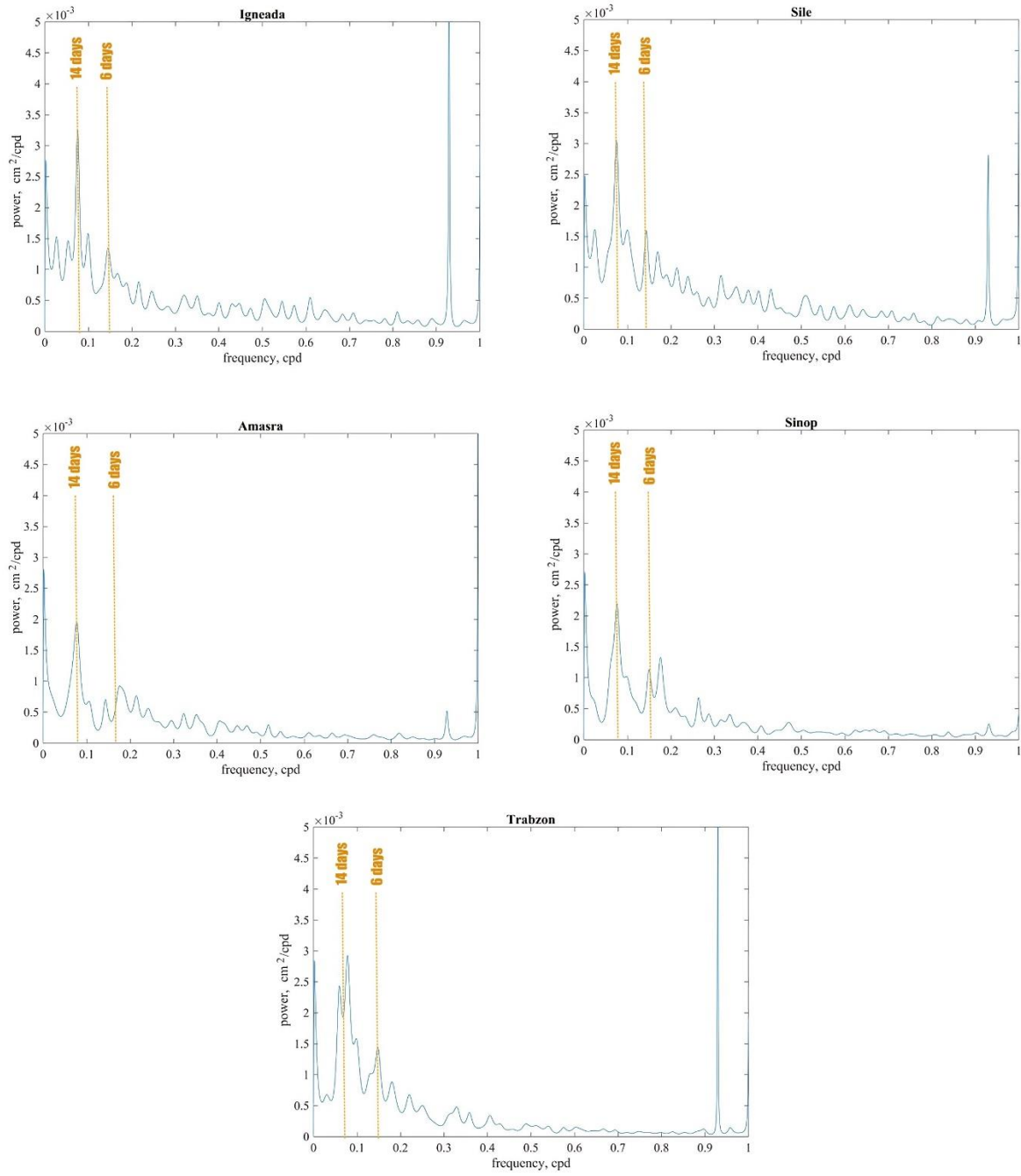
330 Figure 3. Variance preserving spectra of the sea level for İğneada, Şile, Amasra, Sinop and Trabzon; frequencies in cycles per day (cpd).
