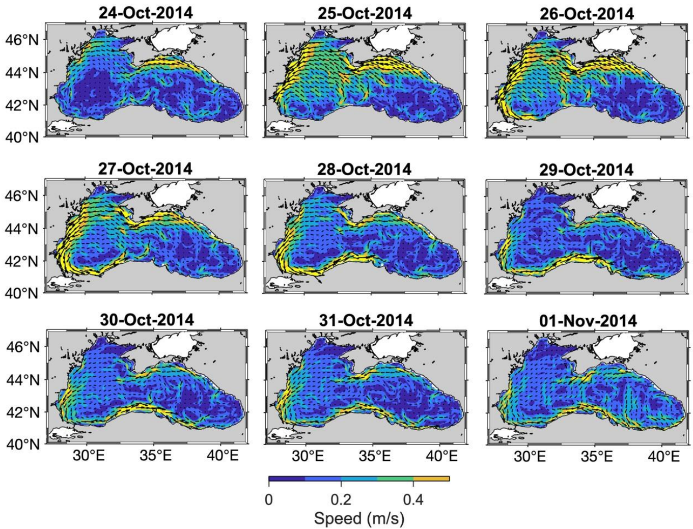
Figure 10. Sequence of daily mean horizontal velocity distributions at 2.5 m from 24 October to 01 November 2014 obtained from Black Sea reanalysis product of CMEMS. For clarity in presentation, just 1 of every 10 vectors is plotted.
