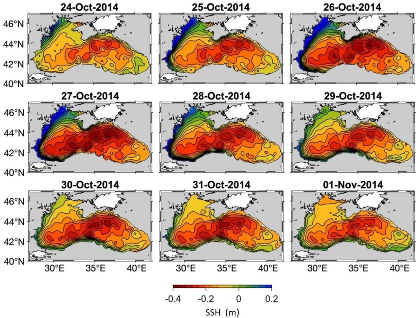
375 Figure 9. Sequence of daily mean Sea Surface Height (SSH) from 24 October to 01 November 2014 obtained from Black Sea reanalysis product of CMEMS.
