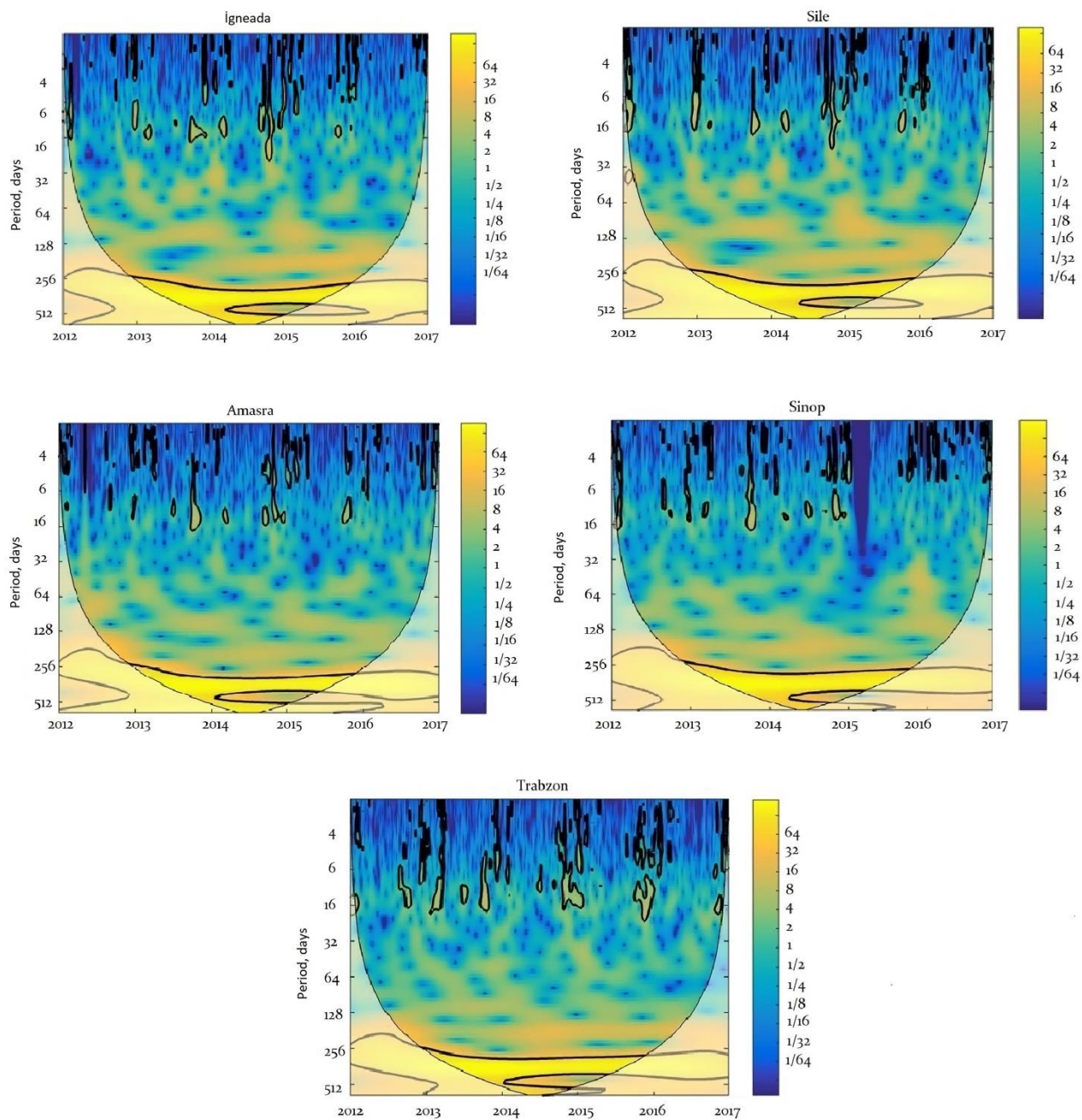
335 Figure 4. Wavelet power spectrum of the sea level for İğneada, Şile, Amasra, Sinop and Trabzon, using the Morlet wavelet. Time is indicated on the x-axis (years) and the timescale (period) on the y-axis. The colour scale of the variance (power) on the z-axis represents an increasing power (variance) from blue to yellow. The areas enclosed by the black contour lines indicate the periods with significance above 95%.
