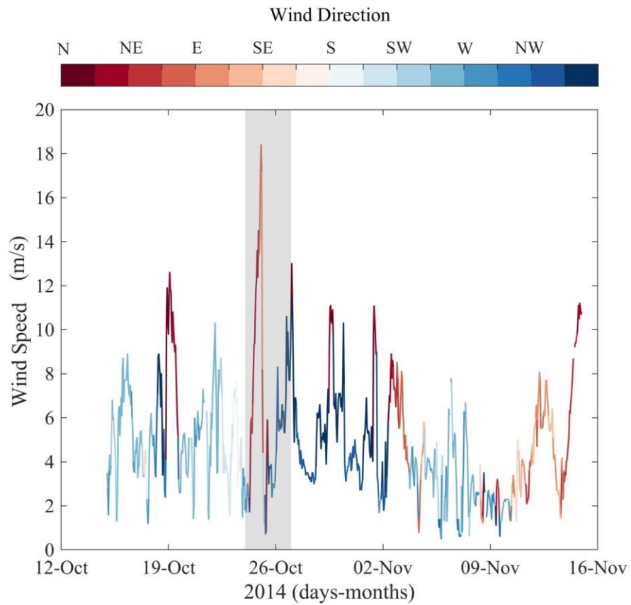
Figure 7. Wind speed and direction at Īgneada for the October 2014 event. Area shaded highlights the excitation of the CTWs period.
