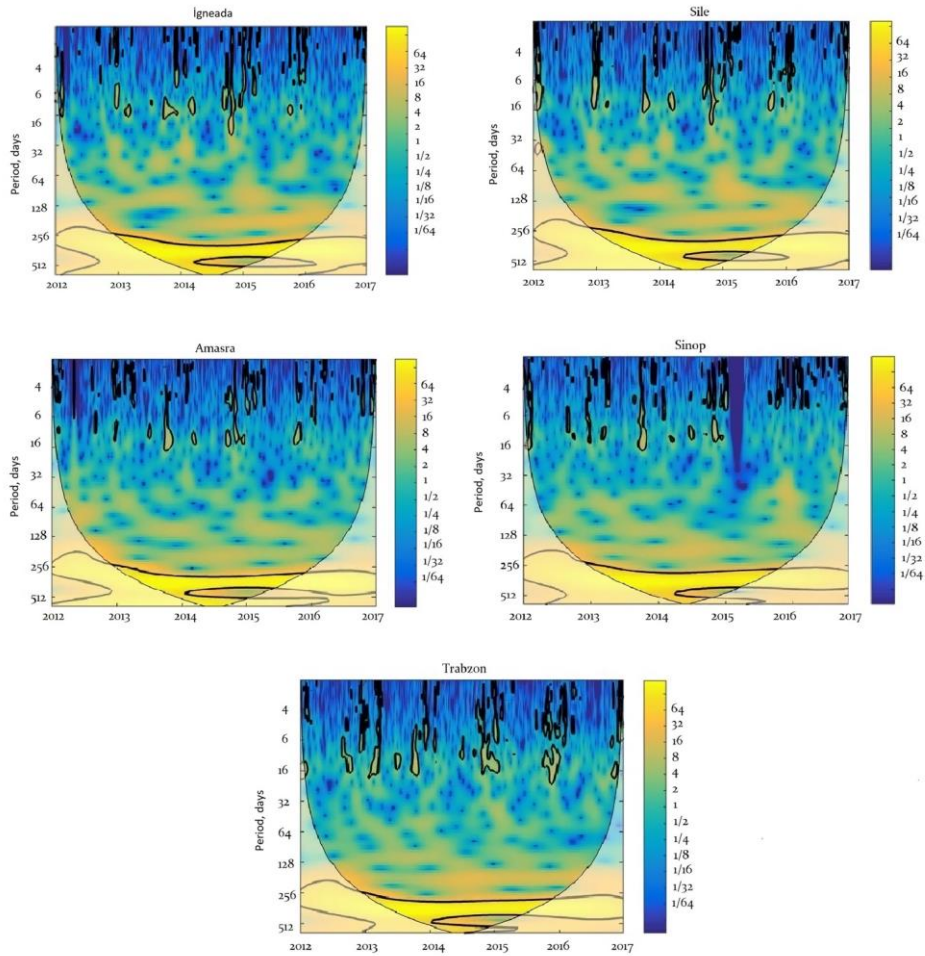
Figure 4. Wavelet power spectrum of the sea level for İğneada, Şile, Amasra, Sinop and Trabzon, using the Morlet wavelet. Time is indicated on the x-axis (years) and the timescale (period) on the y-axis. The colour scale of the variance (power) on the z-axis represents an increasing power (variance) from blue to yellow. The areas enclosed by the black contour lines indicate the periods with significance above 95%.
