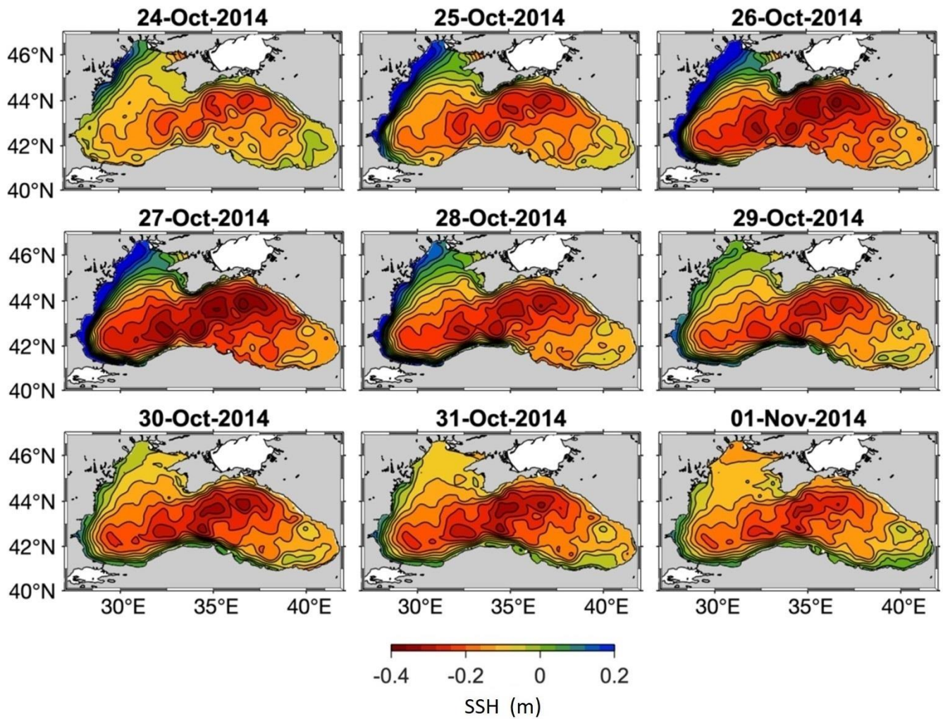
380 Figure 9. Sequence of daily mean Sea Surface Height (SSH) from 24 October to 01 November 2014 obtained from Black Sea reanalysis product of CMEMS.
