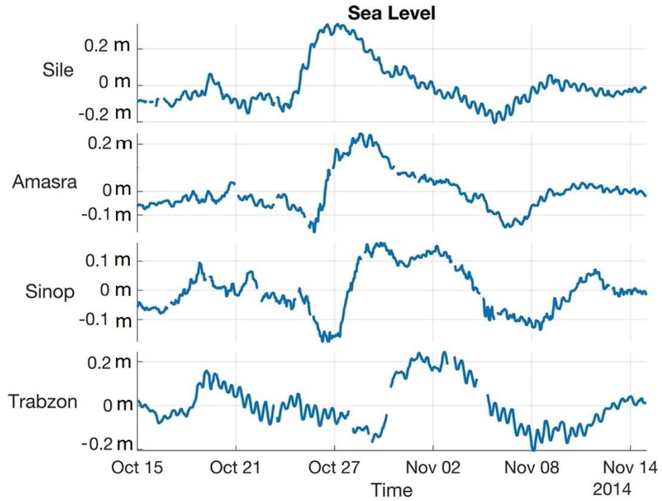
Figure 5. Time series of the sea level variations from 15 October 2014 to 15 November 2014. The data is subsampled from Fig. 2. The data is smoothed using robust linear regression method of MATLAB smoothdata function with rlowess option.
