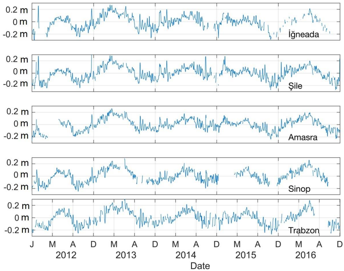
330 Figure 2. Time series of hourly sea level in meters from İğneada, Şile, Amasra, Sinop and Trabzon from 2012 to 2017. The data is smoothed using robust linear regression method of MATLAB smoothdata function with rlowess option.
