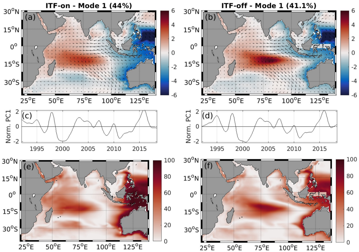
760 Figure 6: Regression of monthly SLA (color) and wind stress (arrow) on the standardized principal component of the first EOF mode (PC1) from 1992 to 2018, for the ITF-on (a) and ITF-off (b) simulations, expressed in centimeters per 1 STD change of the respective PC1. (c, d) Time evolution of the associated PC1 normalized by their standard deviations. (e, f) Explained variance between the modeled and the reconstructed SLA.
