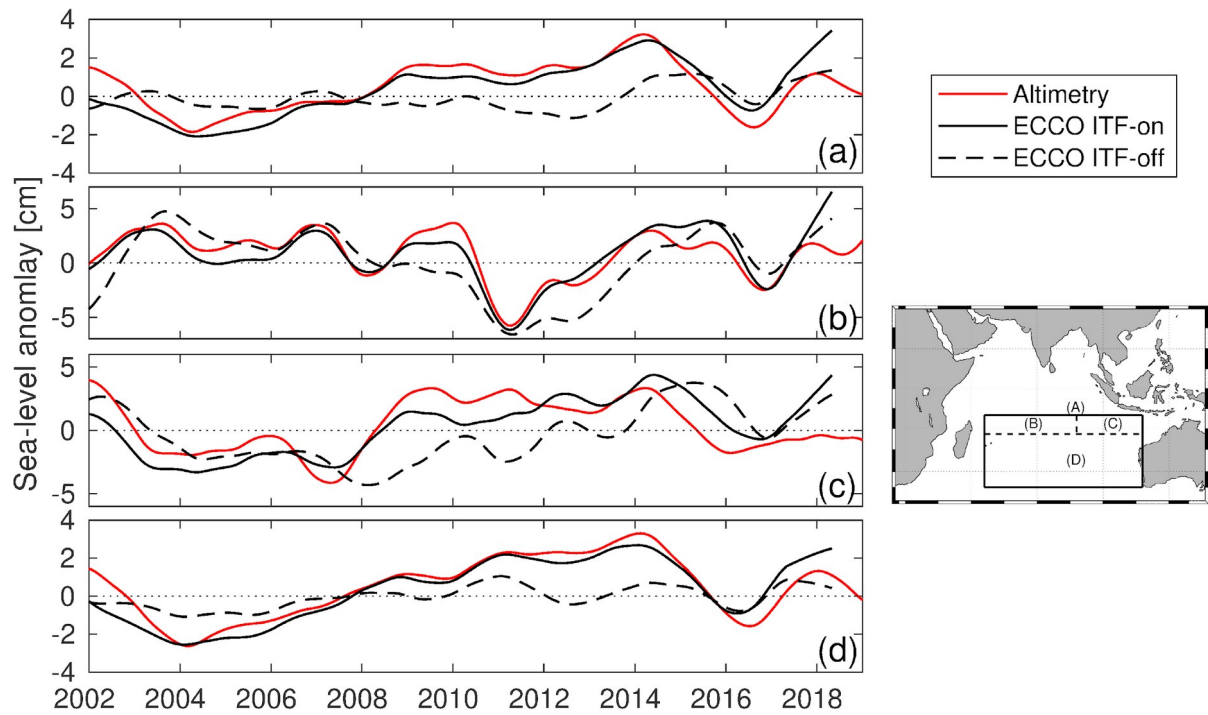
Figure 4: Time series of the sea-level anomaly (SLA) from altimetry (red line), and from numerical simulations (ITF-on: black line; ITF-off: black dashed line). The SLA (a, b, c, d) are averaged, respectively, in four areas (A, B, C, D) represented in the map on the right panel. All the time series are low pass filtered with a cutoff period of 1 year.
