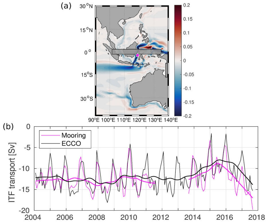
745 Figure 2: (a) Difference between the time-mean absolute ocean current velocities ( \text{m s}^{-1} ) averaged over the upper 100 m in the ITF-off and the ITF-on numerical simulations. (b) Monthly ITF transport in the upper 760 m from the ITF-on numerical simulation (black line) and in situ velocity measurements (magenta line) from subsurface moorings across the Makassar Strait (magenta star in fig. a). The bold lines represent the low pass filtered time series with a cutoff period of 1 year.
