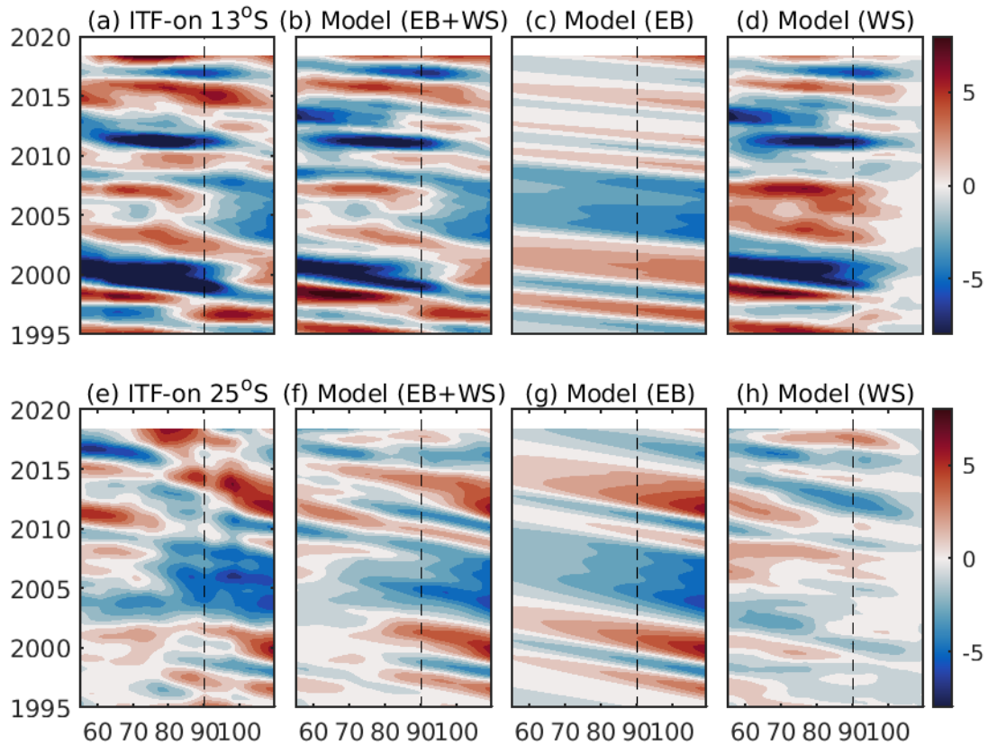
770 Figure 8: Hovmöller diagrams of (a,e) the ECCO modeled SLA at 13°S and 25°S from the ITF-on simulation; (b,f) the RG modeled SLA using both the eastern boundary and the local wind stress curl forcing; (c,g) the RG modeled SLA obtained using the eastern boundary forcing only, and (d,h) the RG modeled SLA obtained using the local wind stress curl forcing only. The results from the ITF-on simulation at 13°S are shown in the top panels, and at 25°S in the bottom panels.
