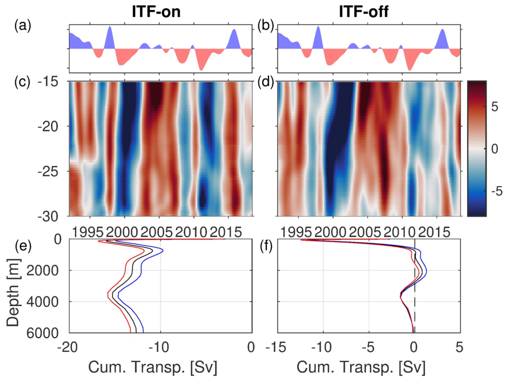
Figure 12: (a,b) Time series of the standardized MEI (El Niño/La Niña are shown by blue/red shading). (c, d) Zonal differences of SLA (cm) computed between 50°-55°E and 110°-115°E ( SLA_{west} - SLA_{east} ) as a function of latitude and time in the ITF-on and ITF-off experiments. (e,f) Time-mean stream function of the meridional flows across 15°S (black line), and the composite of the stream function associated with El Niño (blue line) and La Niña (red line) in the ITF-on and ITF-off experiments.
