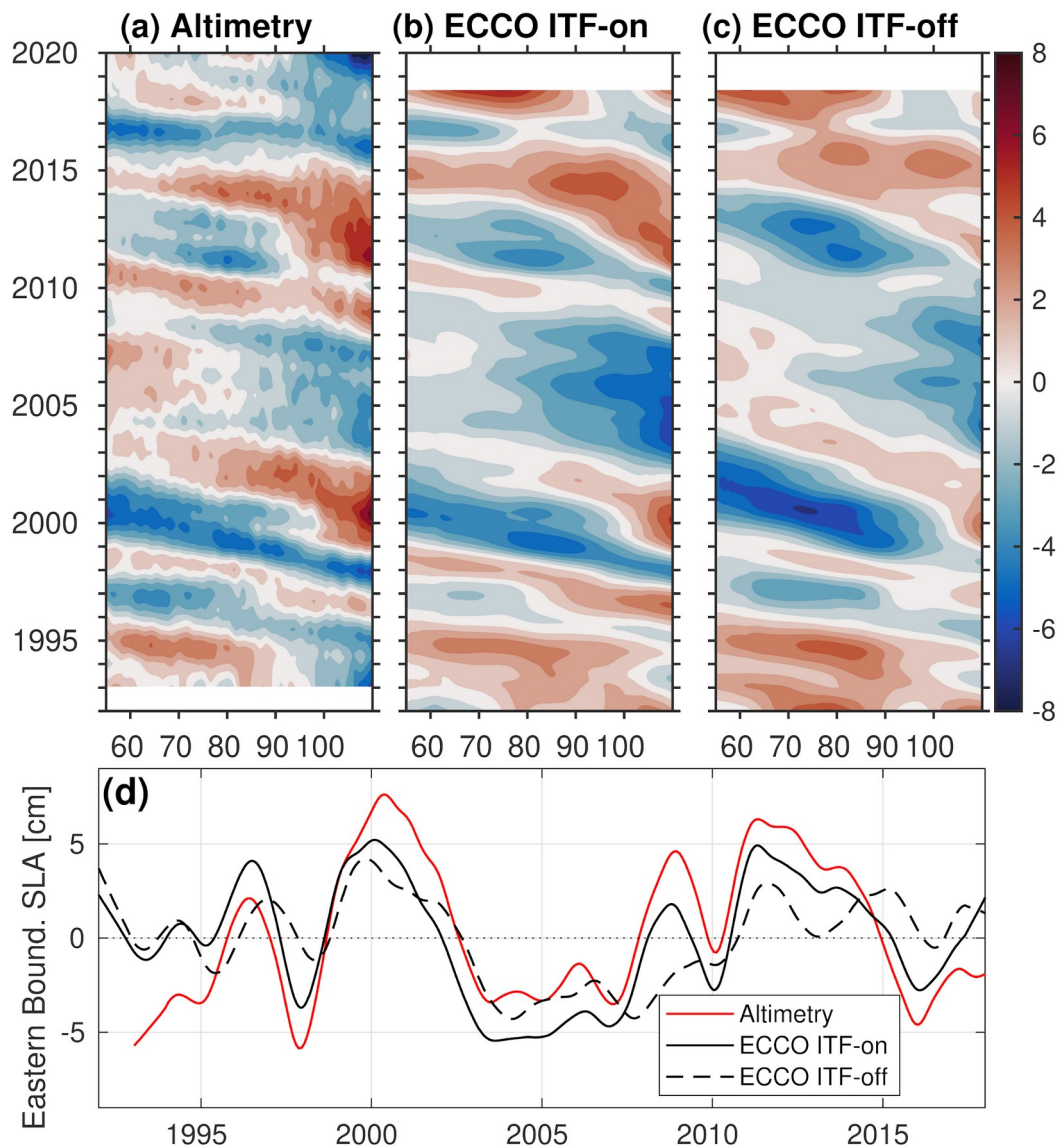
755 Figure 5: Hovmöller diagrams of (a) the observed SLA; (b) the ECCO modeled SLA from the ITF-on simulation; (c) the ECCO modeled SLA from the ITF-off simulation, averaged between 10°S and 30°S. (d) Time series of SLA from altimetry (red line) and from numerical simulations (ITF-on: black line; ITF-off: black dashed line) averaged between 10°S and 30°S at 110°E. All the time series are detrended and low pass filtered (with a cutoff period of 1 year).
