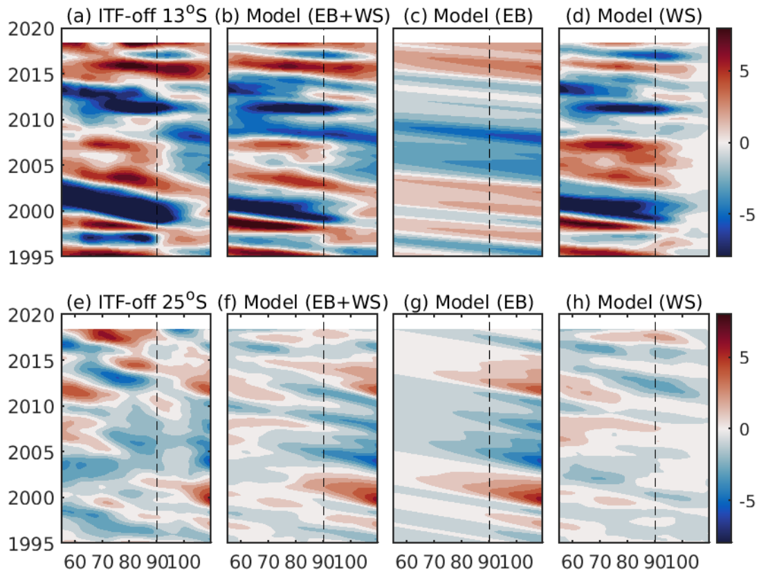
Figure 10: Hovmöller diagrams of (a,e) the ECCO modeled SLA at 13°S and 25°S from the ITF-off simulation; (b,f) the RG modeled SLA using both the eastern boundary and the local wind stress curl forcing; (c,g) the RG modeled SLA obtained using the eastern boundary forcing only, and (d,h) the RG modeled SLA obtained using the local wind stress curl forcing only. The results from the ITF-off simulation at 13°S are shown in the top panels, and at 25°S in the bottom panels.
