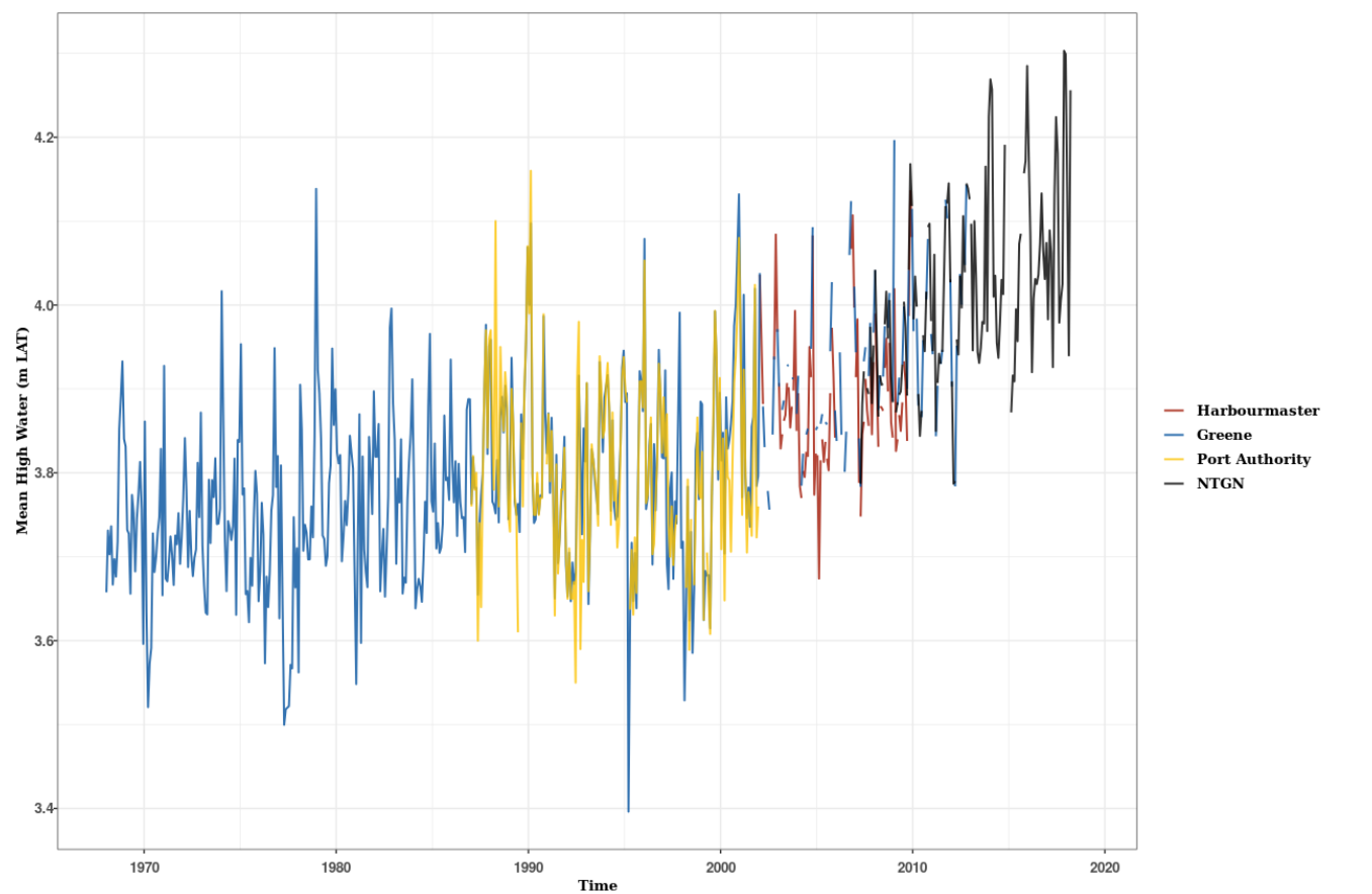
Figure 1. Monthly MHW in Dublin from the Port Authority, Greene, Harbourmaster, and NTGN datasets. A high level of agreement is found between the records indicating consistent datum definition, with only a small adjustment of 0.008 m to the Greene dataset for complete reconciliation.
