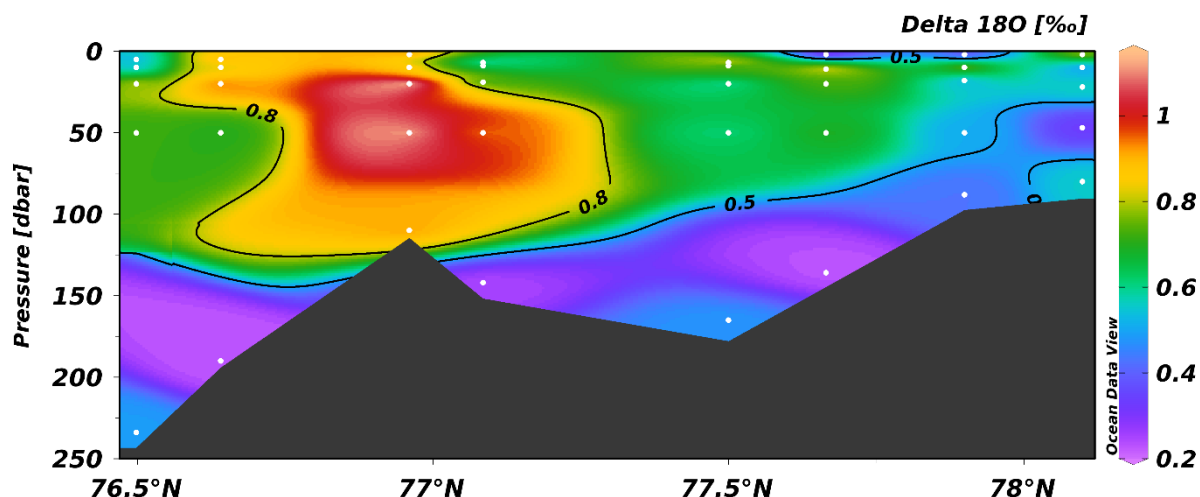
Figure 4 - Oxygen isotope ratio ( \delta^{18}\text{O} ) from water samples, sample location indicated with white dots. Bathymetry is based on echo depth at the CTD stations. Plots are made with Ocean Data View (Schlitzer, Reiner, Ocean Data View, adv.awi.de , 2021).
