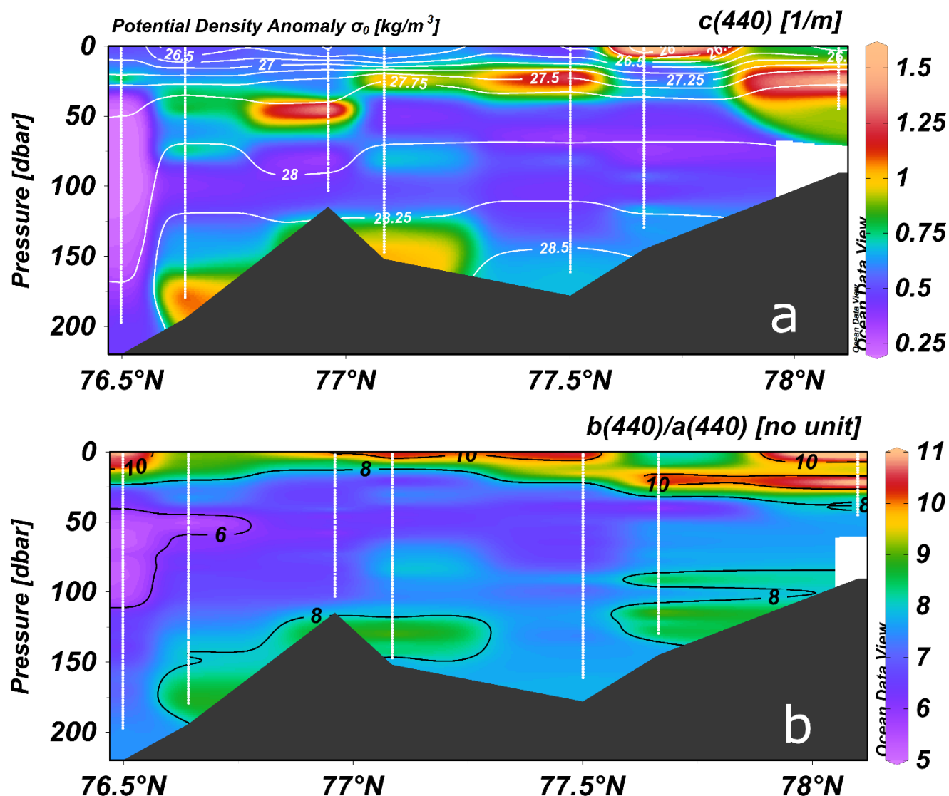
Figure 6 - Total attenuation coefficient ( c ) with white contours of potential density anomaly (panel a) and ratio of scattering (b) to absorption (a) at 440 nm (panel b) from in situ ac-s data for the South–North transect (see Figure 1). Plots are made with Ocean Data View (Schlitzer, Reiner, Ocean Data View, odv.awi.de , 2021).
