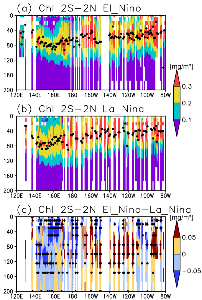
515 Figure 11. (a-c) Cross-sections of the chlorophyll a (Chl-a) concentrations in the equatorial Pacific (2°S to 2°N) during El Niño and La Niña, and the difference between them. The black dots denote the depth of the Chl-a maximum in panels (a) and (b), and the significant difference at 5% in panel (c).
