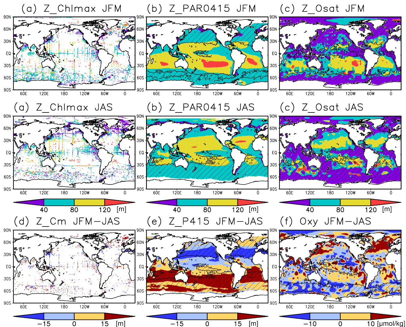
485 Figure 7. (a–c) Depths of the chlorophyll a (Chl-a) maximum, photosynthetically active layer ( >0.415 einstein/m 2 /day of photosynthetically available radiation), and oxygen-oversaturated layer in January–March (JFM) (top) and July–September (JAS) (middle), respectively. (d–f) Differences between the Chl-a maximum depth, photosynthetically active layer depth, and dissolved oxygen concentrations at 50–150 m during JFM compared to those in JAS. The hatched areas indicate a mixed layer deeper than the photosynthetically active layer in panel (b), the oxygen saturation layer in panel (c), the photosynthetically active layer in winter in panel (e), and 50 m in summer in panel (f). 490
