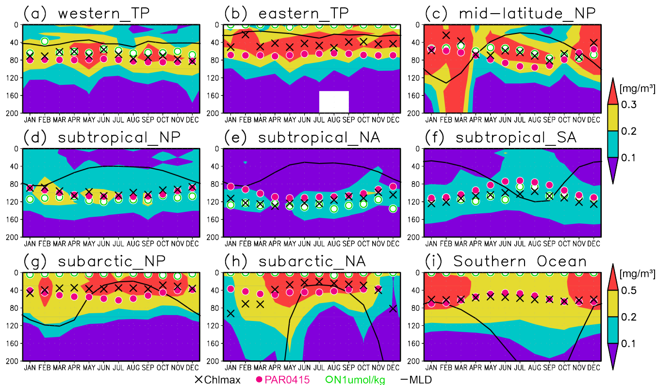
505 Figure 10. Seasonal evolution of chlorophyll a (Chl-a) concentrations with the Chl-a maximum (black crosses), 0.415 einstein/m 2 /day of photosynthetically available radiation (magenta dots), 1 \mu\text{mol/kg} of nitrate (green open circles), and mixed layer (black solid line) at (a) 2°S to 2°N, 120–170°E (western tropical Pacific), (b) 2°S to 2°N, 120–90°W (eastern tropical Pacific), (c) 30–40°N, 150–130°W (midlatitude North Pacific), (d) 10–30°N, 120°E to 120°W (subtropical North Pacific), (e) 15–30°N, 70– 510 30°W (subtropical North Atlantic), (f) 30–10°S, 50–0°W (subtropical South Atlantic), (g) 40–55°N, 160°E to 155°W (subarctic North Pacific), (h) 50–70°N, 30–0°W (subarctic North Atlantic), and (i) 60–45°S (Southern Ocean).
