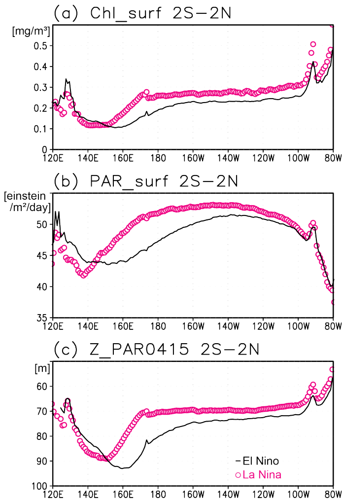
520 Figure 12. (a) Satellite-derived surface chlorophyll a concentrations, (b) surface photosynthetically available radiation (PAR), and (c) photosynthetically active layer (>0.415 einstein/m 2 /day of PAR) along the equatorial Pacific during El Niño (black solid lines) and La Niña (magenta open circles).
