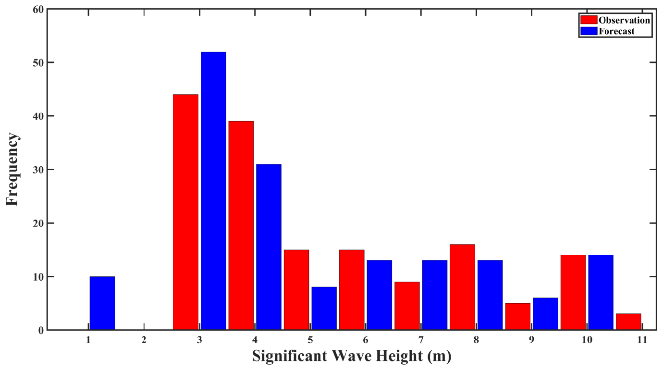
7 Figure S3. Same as Figure S1, but for Hurricane Igor.
