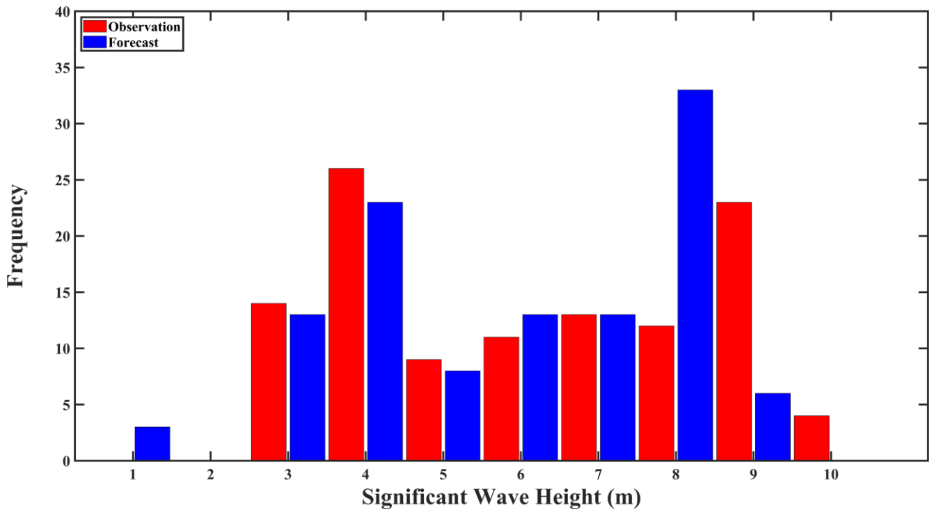
5 Figure S2. Same as Figure S1, but for Hurricane Sandy.
