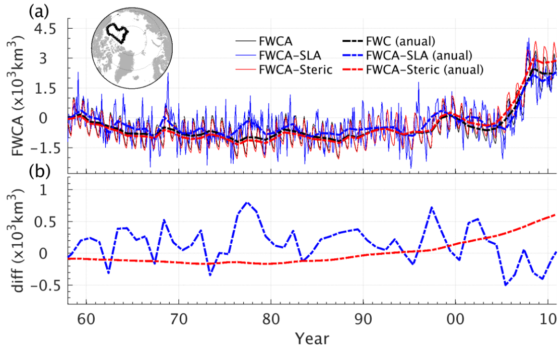
369 Figure 11. (a) Freshwater content anomalies ( 10^3 \text{ km}^3 ) and approximated based on Eq. (6) in blue and Eq. (7) in 370 red using the monthly output of ATLARC08km. The thick dashed lines are the annual mean values. (b) The 371 differences of the approximated annual mean freshwater content anomalies based on Eq. (6) in blue and Eq. (7) 372 in red to the annual mean freshwater content anomalies.
