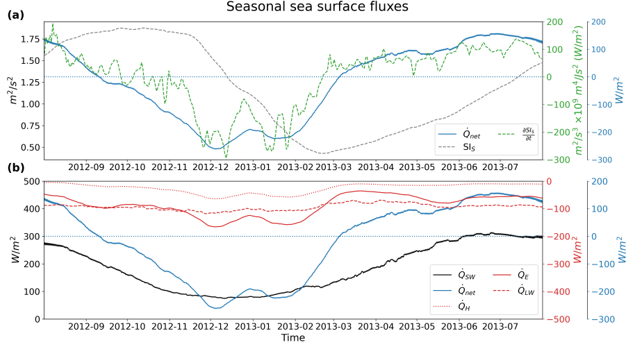
Figure 9. The smoothed (with Eq. (3)) seasonal surface heat fluxes over the point 42^\circ \text{ N } 5^\circ \text{ E} for the Seasonal simulation. (a) contains the seasonal stratification index, SI_S , and its derivative, \frac{\partial SI_S}{\partial t} , comparing it to the seasonal net heat flux, Q_{net} (the subscript S is dropped for convenience). (b) shows the net heat flux separated into its components: Q_E , Q_H , Q_{SW} , and Q_{LW} for latent heat, sensible heat, shortwave downward, and longwave downward fluxes, respectively (neglecting contributions from precipitation and snowfall). The different line colors correspond to the similarly colored axes.
