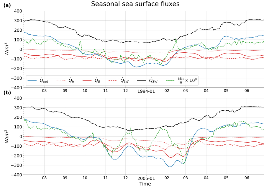
Figure 17. The smoothed seasonal sea surface fluxes spatially averaged over the 42 to 42.5 ° N and 4.25 to 5 ° E area, with the green dashed line denoting the estimated derivative w.r.t. time of the seasonal SI from the NEMO results, multiplied by 10^9 \text{ m}^4/\text{Js}^2 . A negative value means heat is leaving the ocean.
