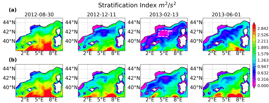
Figure 7. The Stratification Index across the Gulf of Lion-GOL (the area marked as NW Med. in Fig. 1 (b)) at different timestamps. Row (a) displays the values of SI for the Control simulation and row (b) displays the values of SI for the Seasonal simulation. The box denoted by DC indicates the area of deep convection in the Gulf of Lion-GOL that was not seen in the Seasonal simulation.
