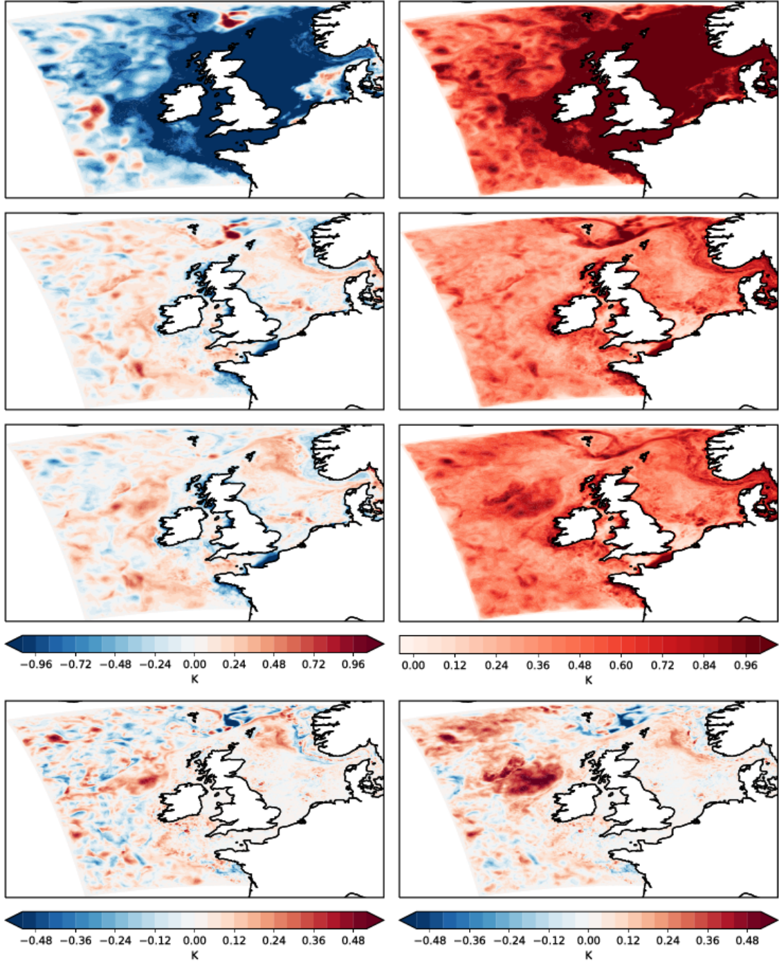
Figure 11. June 2018 vertically-averaged temperature bias (left) and RMSE (right) for Free Run (top), Control (second row) and LowErrSWOT experiments (third row). The difference (Control-LowErrSWOT) in the absolute bias and RMSE between the Control and LowErrSWOT experiments is also shown (bottom row) to highlight the impact of the additional SWOT observations.
