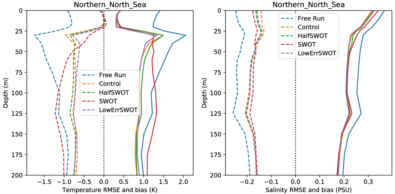
Figure 14. On-shelf Northern North Sea temperature and salinity RMSE (solid) and bias (dashed) averaged over June–October when the full year of the experiments temperature and salinity balanced changes due to SSH assimilation are applied.
