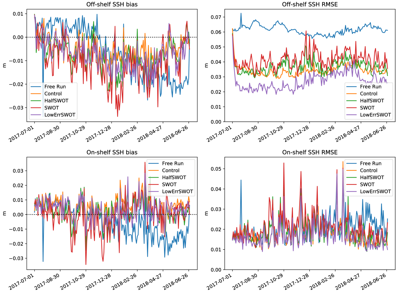
Figure 7. SSH bias (m, left) and RMSE (right) for the off-shelf (top) and on-shelf (bottom) regions.
