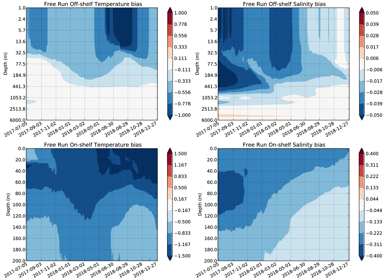
Figure 3. Free Run temperature (left) and salinity (right) biases relative to the Nature Run ( Free-Nature ) for the off-shelf (top) and on-shelf (bottom) regions. Note that the off-shelf plots are shown on a log depth scale.
