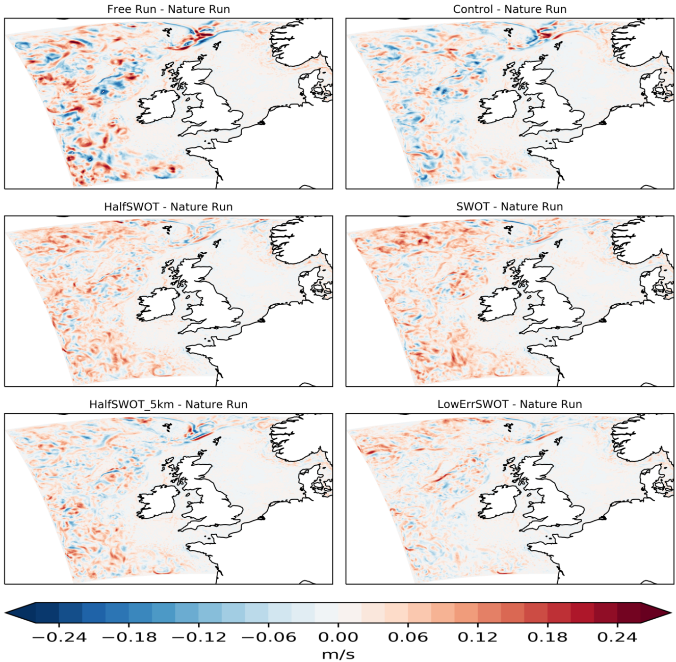
Figure 15. Monthly (June 2018) mean surface current speed error (compared to Nature Run) from the Free Run (top left), Control, HalfSWOT, SWOT , HalfSWOT_5km, SWOT and LowErrSWOT experiments (bottom).
