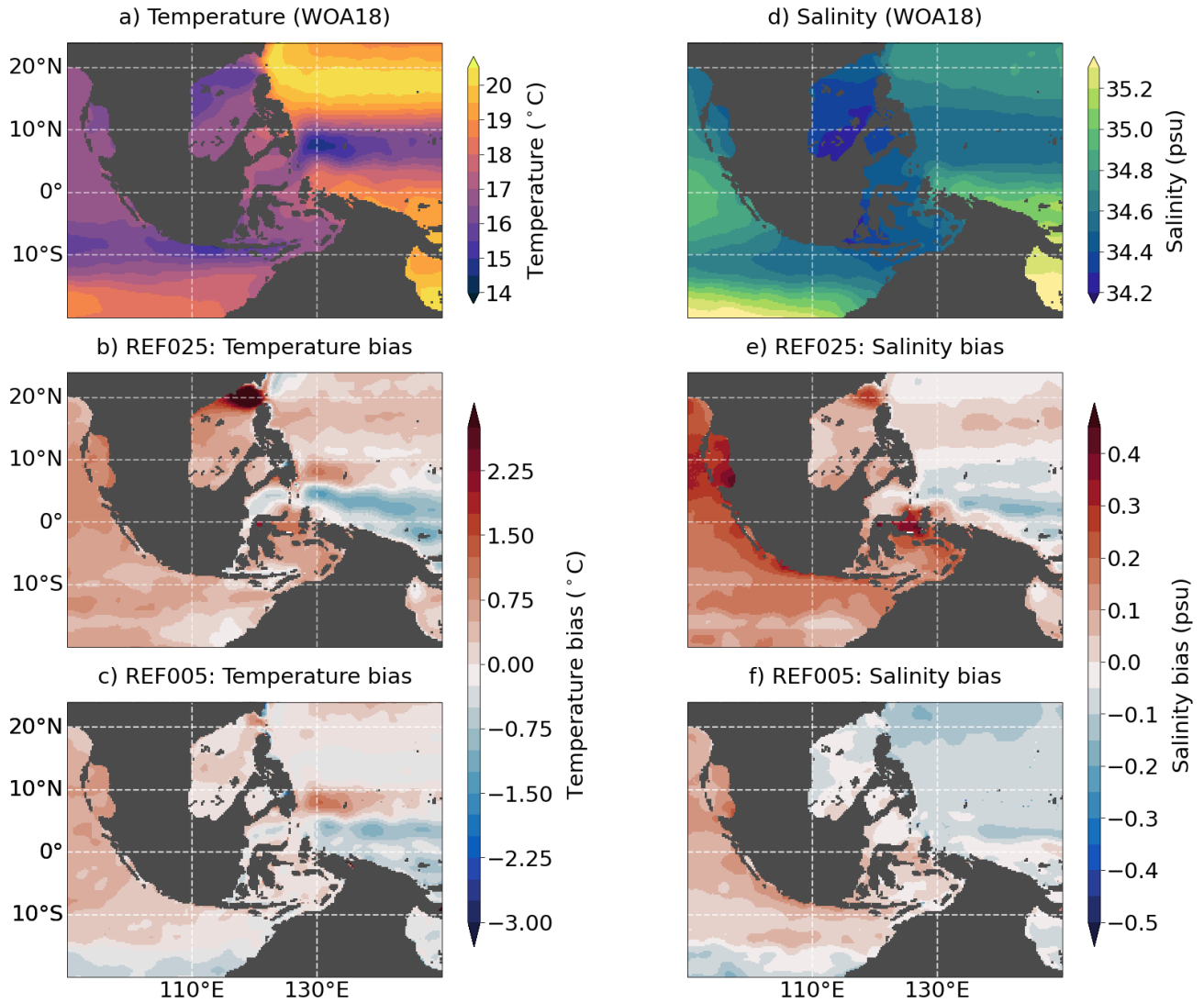
Figure 3. Mean fields (1955–2017; upper row) and model biases (1958–2016; middle and bottom row) averaged over the upper 400 m for (a-c) temperature and (d-f) salinity. Note that data is only shown where the water depth exceeds 400 m.
