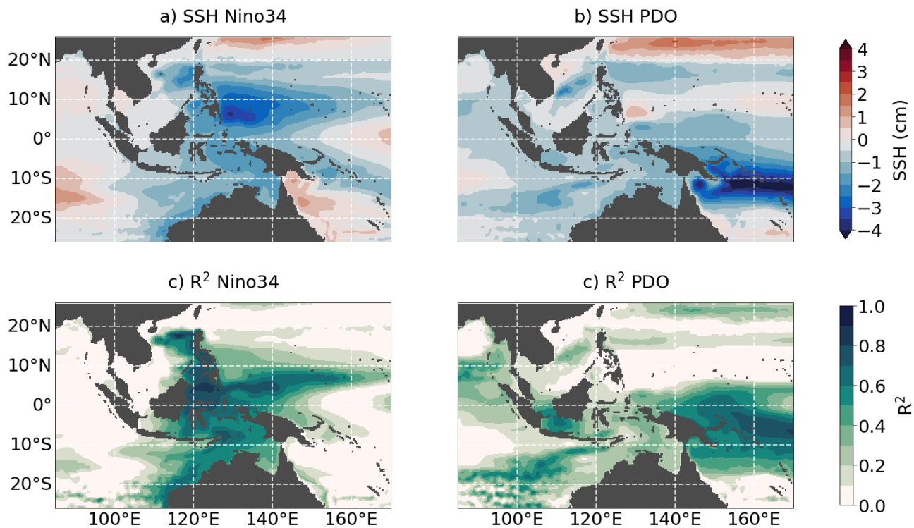
Figure A2. Linear regression of SSH from WIND on (a) Niño3.4 and (b) PDO index and (c, d) respective coefficients of determination. Both climate indices are derived from REF025. All data were filtered with an 8-year low-pass filter.
