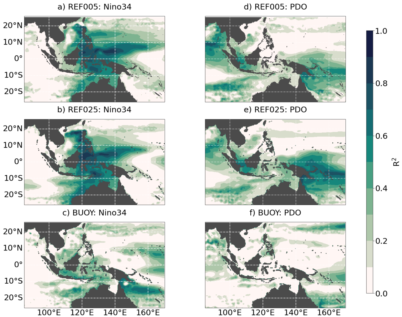
Figure 6. Coefficient of determination for the linear regression of SSH with (a-c) Niño3.4 index and (d-f) PDO index for two hindcast (REF025, REF005) and buoyancy forcing experiments (BUOY). Climate indices are derived from its base model in case of REF005 and from REF025 for the other two experiments. All data has been filtered with an 8-year low-pass filter.
