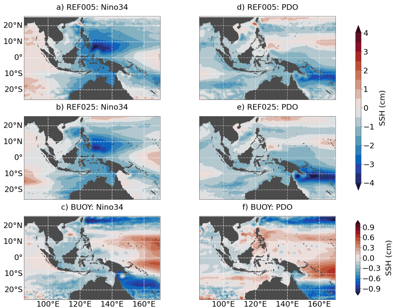
Figure 5. Linear regression of SSH with (a-c) Niño3.4 index and (d-f) PDO index for two hindcast (REF025, REF005) and buoyancy forcing experiments (BUOY). Climate indices are derived from its base model in case of REF005 and from REF025 for the other two experiments. All data has been filtered with an 8-year low-pass filter. Note the different colorbars.
