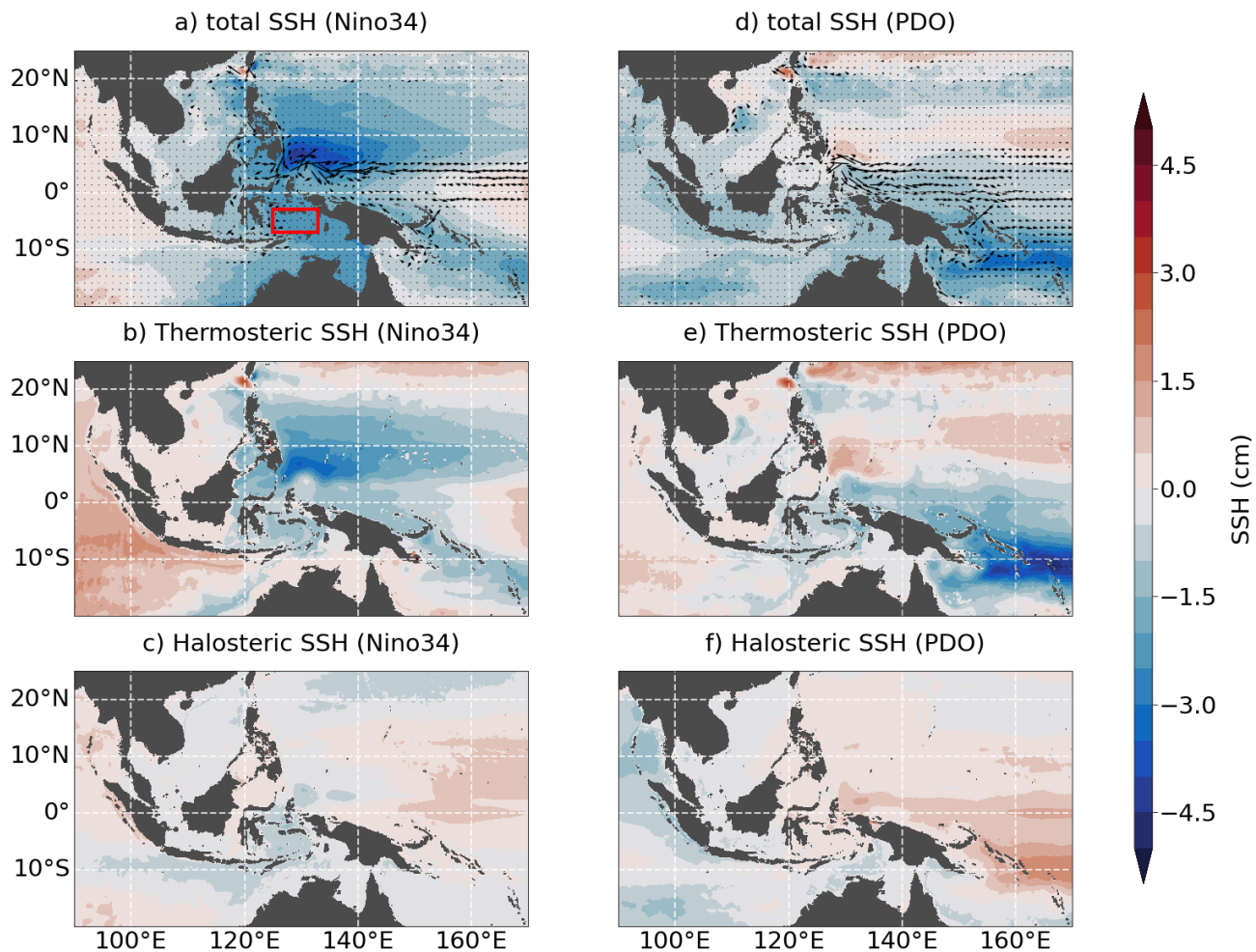
Figure 7. Linear regression with (a-c) Niño3.4 and (d-f) PDO index of upper ocean currents (arrows; 0–150 m), total, thermosteric and halosteric SSH. All data is taken from REF005 and were filtered with an 8-year low-pass filter. Note that the colour shading in panels a) and b) is the same as in Fig. 5a, b)
