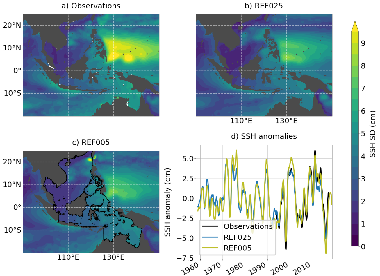
Figure 2. SD of SSH from (a) observations and two hindcast experiments (b) REF025 and (c) REF005 over the period 1993 to 2016. d) SSH anomalies averaged over the region marked by black contours in panel c). The global mean trends over the integration period have been subtracted, and all data were smoothed with a 12-month running mean window.
