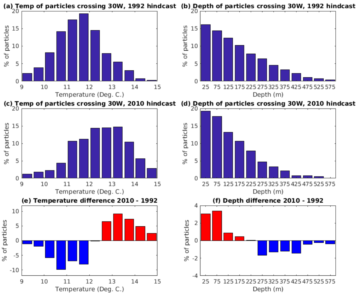
665 Figure 13: Histograms from the 1992 and 2010 hindcast, showing the temperature and depth of unique particles crossing 30 °W for the first time (any further crossings are ignored). (a) 1992 particle temperature; (b) 1992 particle depth; (c) 2010 particle temperature; (d) 2010 particle depth; (e) temperature difference; (f) depth difference. Positive difference = more particles in 2010. Data binned by 0.5 °C temperature and 50m depth.
