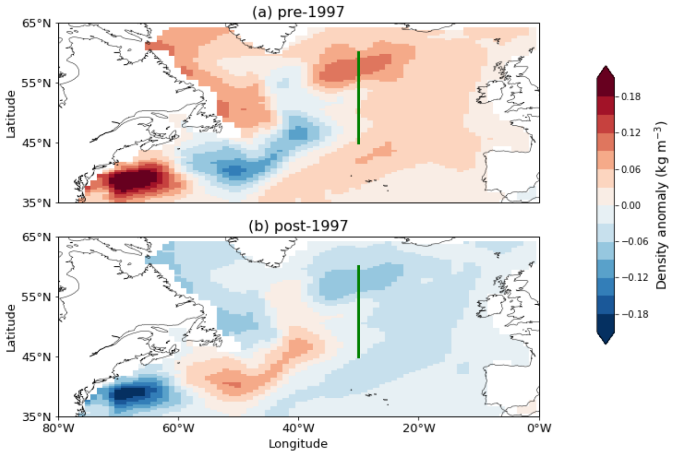
610 Figure 2: Mean anomaly maps of density at 205 m below the surface: (a) pre-1997; (b) post-1997. Data from GODAS. Anomalies calculated with respect to the 1980 – 2020 climatology. Green line at 30°W shows the meridional profile used for eastward transport calculations, between 45 °N and 60 °N
