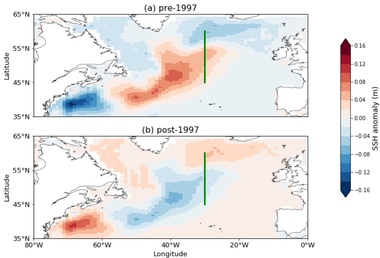
615 Figure 3: Mean anomaly maps of sea surface height (SSH): (a) pre-1997; (b) post-1997. Data from GODAS. Anomalies calculated with respect to the 1980 – 2020 climatology. Green line at 30 °W shows the meridional profile used for eastward transport calculations, between 45 °N and 60 °N.
