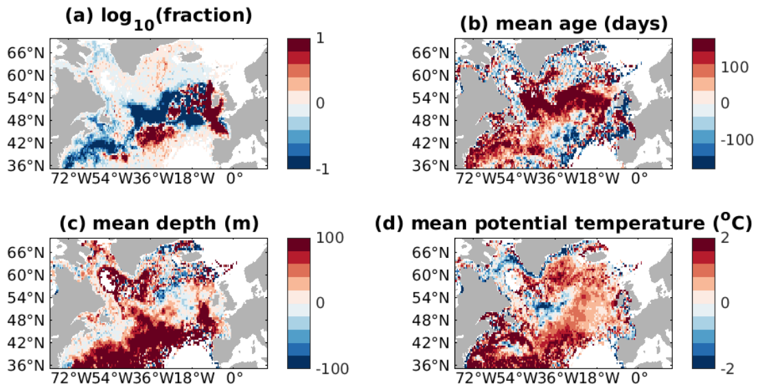
655 Figure 11: Difference between the ensemble mean statistical analyses of the ARIANE 4-year hindcasts: (a) 2010 mean – 1992 mean \log_{10} fraction of total particles; (b) 2010 mean – 1992 mean age in days; (c) 2010 mean – 1992 mean depth in metres, positive = shallower; (d) 2010 mean – 1992 mean potential temperature in ^{\circ}\text{C} .
