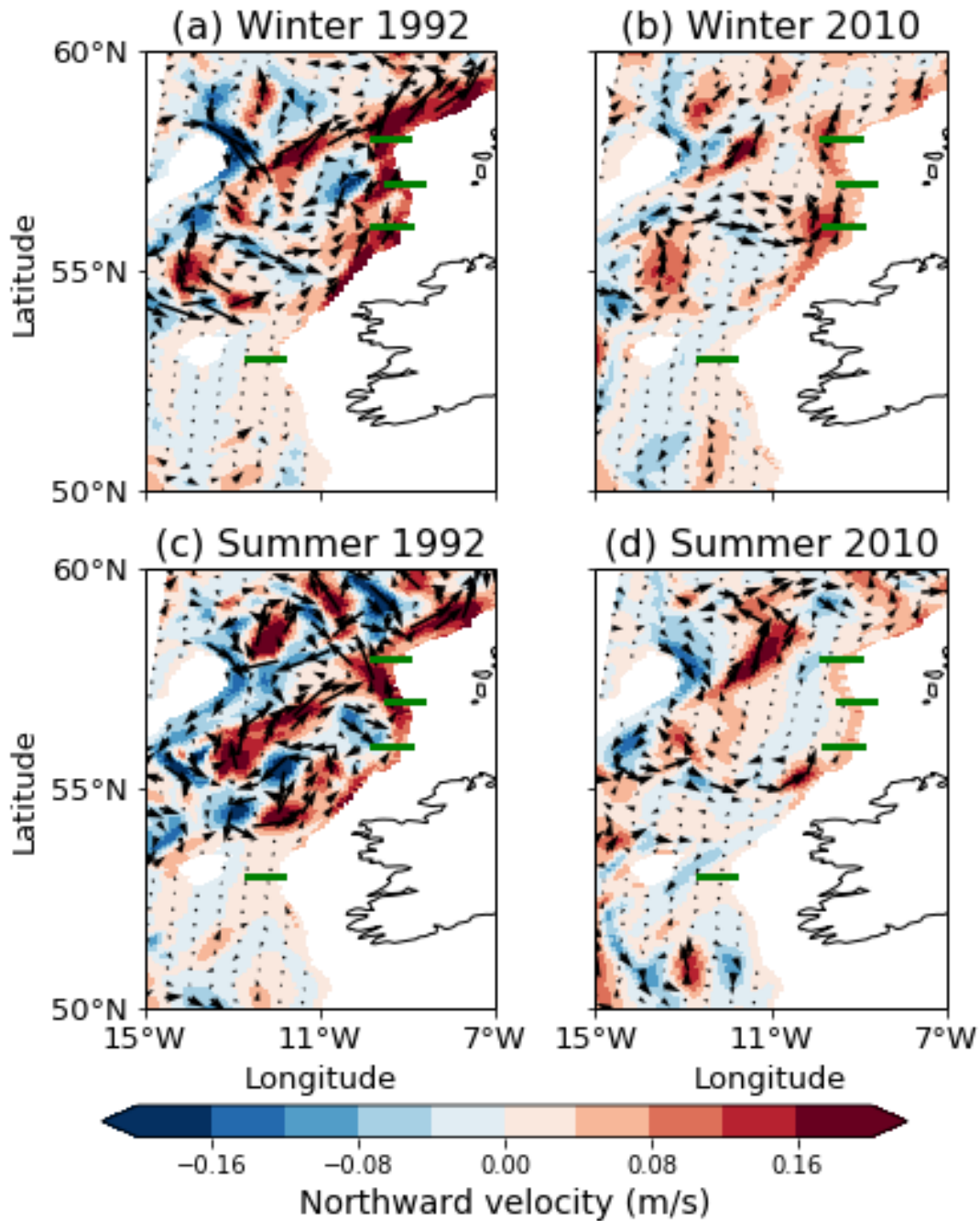
605 Figure 1: quiver plot, using ORCA12 data, indicating subsurface (245 m) velocity magnitude and direction of the water, comparing winter (January) and summer (July) releases: (a) winter 1992; (b) winter 2010; (c) summer 1992; (d) summer 2010. Background colour highlights the magnitude of the v component of velocity, positive northwards. Green lines indicate the zonal transects used for Figure 8.
