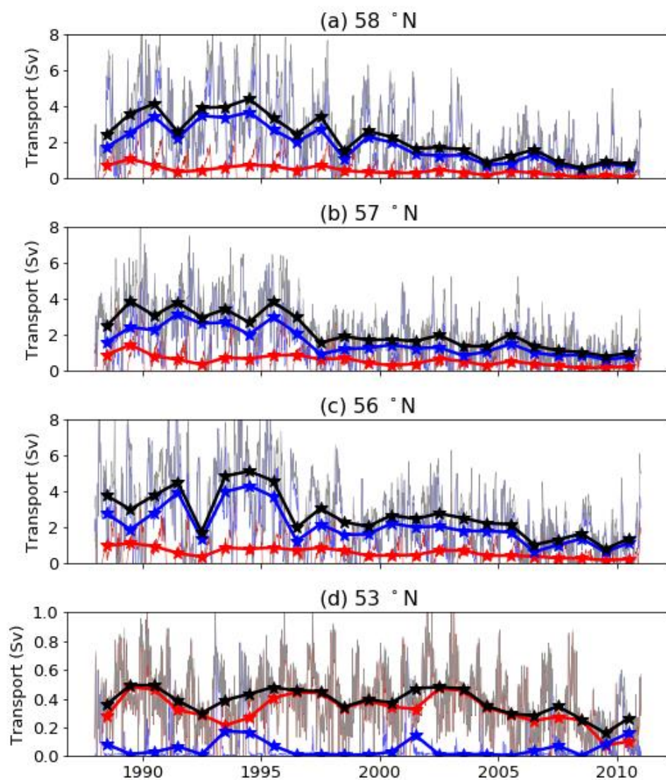
Figure 8: Northward total transport at the shelf edge from the ORCA12 hindcast, across ~400 km -zonal transects at (a) 58°N, (b) 57°N, (c) 56°N, and (d) 53°N (see Fig. 1). Transects are the following length, as constrained by the bathymetry : 53°N is 53.7 km; 56°N is 51.0 km; 57°N is 50.2 km; 58°N is 49.5 km approximately 50 km long . Total transport is indicated with black lines. Transport at temperatures above and below 11°C is indicated with red and blue lines respectively. Thin lines show 5-daily means. Thick lines and stars indicate the annual mean. Note that Y-axis scales on (d) are different from (a)-(c).
