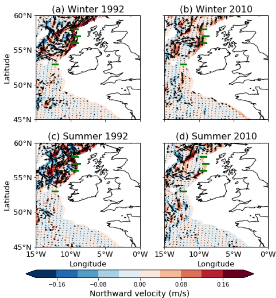
Figure 1: quiver plot, using ORCA12 data, indicating subsurface (245 m) relative-velocity magnitude and direction of the water, comparing winter (January) and summer (July) releases: (a) winter 1992; (b) winter 2010; (c) summer 1992; (d) summer 2010. Background colour highlights the magnitude of the v component of velocity, positive northwards. Green lines indicate the profiles zonal transects used for Figure 8.
