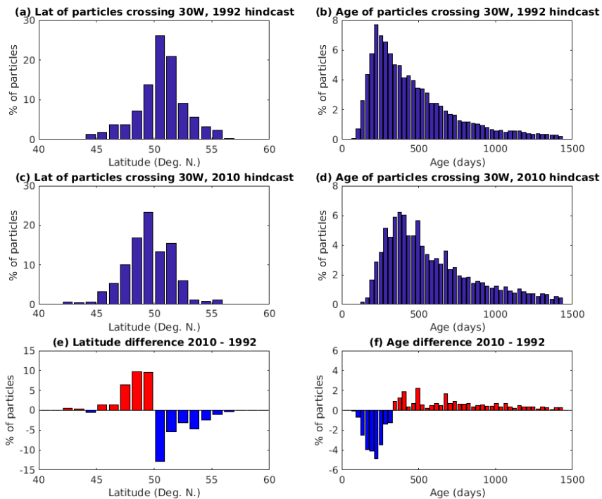
Figure 12: Histograms from the 1992 and 2010 hindcast, showing the latitude and age of unique particles crossing 30 °W for the first time (any further crossings are ignored). (a) 1992 particle latitude; (b) 1992 particle age; (c) 2010 particle latitude; (d) 2010 particle age; (e) latitude difference; (f) age difference. Positive difference = more particles in 2010. Data binned by 1° latitude and 30 days.
