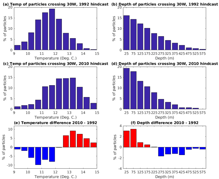
660 Figure 13: Histograms from the 1992 and 2010 hindcast, showing the temperature and depth of unique particles crossing 30 °W for the first time (any further crossings are ignored). (a) 1992 particle temperature; (b) 1992 particle depth; (c) 2010 particle temperature; (d) 2010 particle depth; (e) temperature difference; (f) depth difference. Positive difference = more particles in 2010. Data binned by 0.5 °C temperature and 50m depth.
