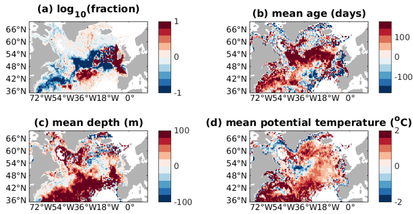
650 Figure 11: Difference between the ensemble mean statistical analyses of the ARIANE 4-year hindcasts: (a) 2010 mean – 1992 mean \log_{10} fraction of total particles; (b) 2010 mean – 1992 mean age in days; (c) 2010 mean – 1992 mean depth in metres, positive = shallower; (d) 2010 mean – 1992 mean potential temperature in ^{\circ}\text{C} .
