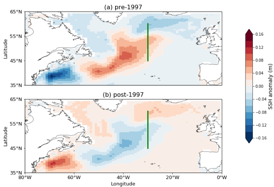
610 Figure 3: Mean anomaly maps of sea surface height (SSH): (a) pre-1997; (b) post-1997. Data from GODAS. Anomalies calculated with respect to the 1980 – 2020 climatology. Green line at 30 °W shows the meridional profile used for eastward transport calculations, between 45 °N and 60 °N.
