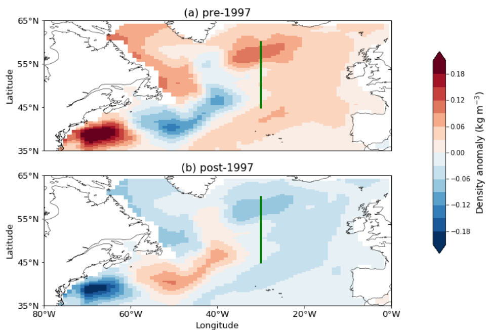
605 Figure 2: Mean anomaly maps of density at 205 m below the surface: (a) pre-1997; (b) post-1997. Data from GODAS. Anomalies calculated with respect to the 1980 – 2020 climatology. Green line at 30°W shows the meridional profile used for eastward transport calculations, between 45 °N and 60 °N
