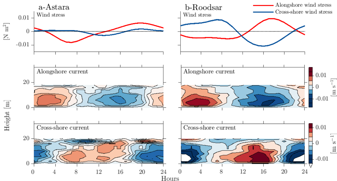
Figure 8. The 24 hours-averaged daily cycle of band-passed alongshore wind stress and cross-shore wind stress (first panel), alongshore current (second panel) and cross-shore current (third panel) at a) Astara and b) Roodsar at about 31 m (Table 1).
