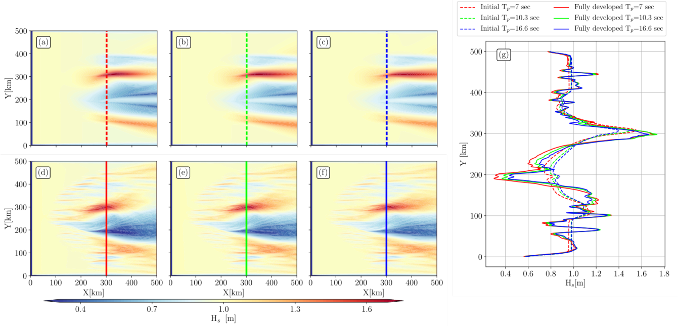
Figure 2. Significant wave height ( H_s ) fields for (a, d) T_p=7 s, (b, e) 10.3 s, and (c, f) 16.6 s incident waves. Without current forcing the entire domain is equal to the initial H_s (1 m). The first row (a, b, c) shows fields for simulations forced with the initial eddy (Fig. 1(a, c)); the second row (d, e, f) shows the same fields but for simulations forced with the fully developed eddy (Fig. 1 b, d). Panel g shows H_s along X = 300 km.
