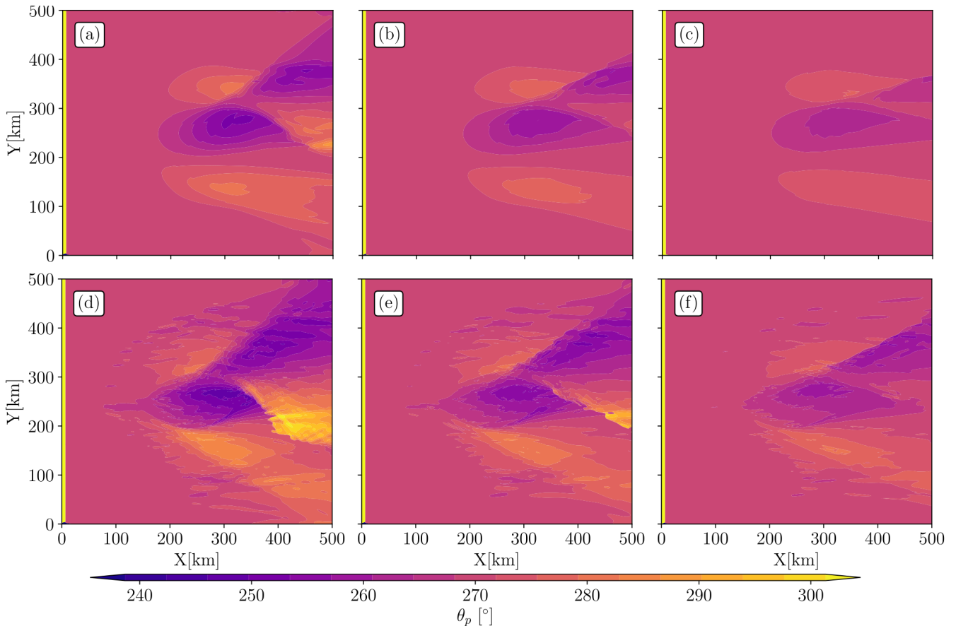
Figure 3. Peak direction ( \theta_p ) fields for (a, d) T_p=7 s, (b, e) 10.3 s, and (c, f) 16.6 s incident waves. Without current forcing, the entire domain is equal to the initial \theta_p ( 270^\circ ). The first row (a, b, c) shows \theta_p for simulations forced with the initial eddy (Fig. 1 a, c); the second row (d, e, f) shows the same fields but for simulations forced with the fully developed eddy (Fig. 1 b, d.) The narrow yellow bands in the left part of every panels are spurious, they marked the boundary where waves are generated at the left boundary.
