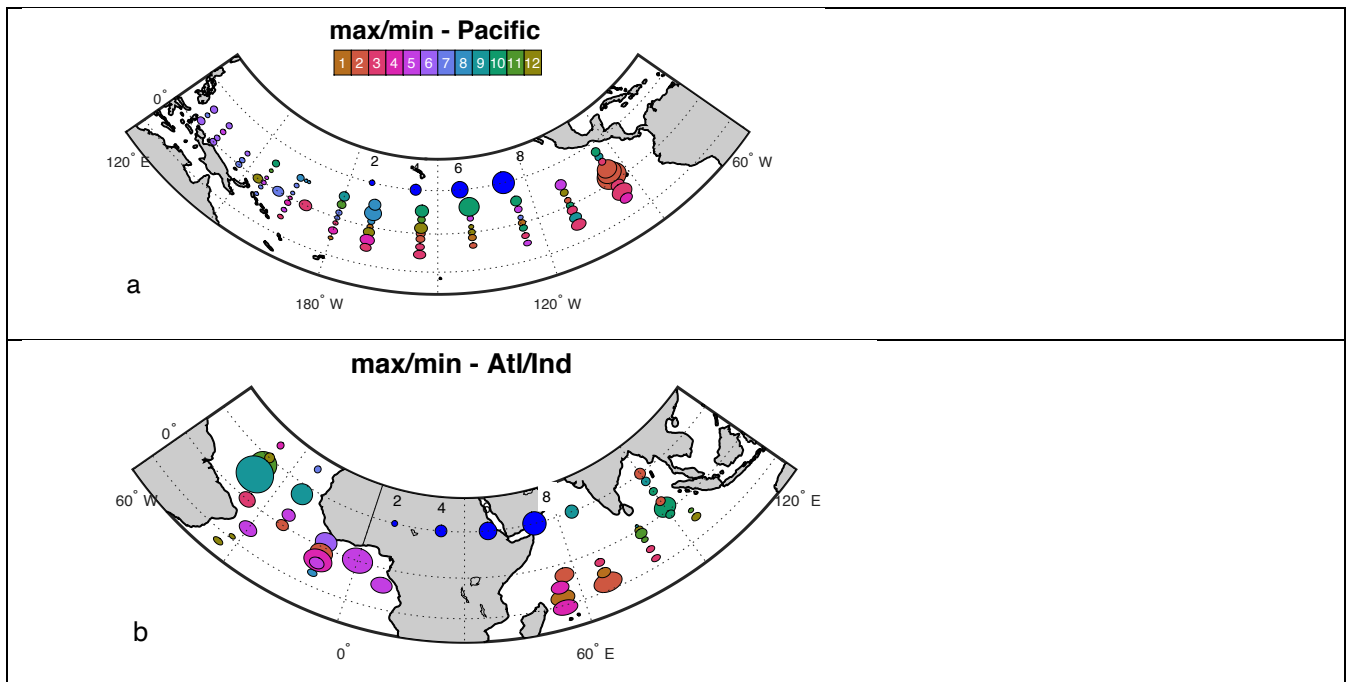
495 Figure 6: Ratio of maximum value of STV to minimum value (sizes of symbols), and month of maximum STV (symbol colors with scale in panel a in months (Jan-Dec)). a) Pacific basin and b) Atlantic and Indian basins. A size scale for the STV ratio is shown as blue circles near the middle of each panel.
