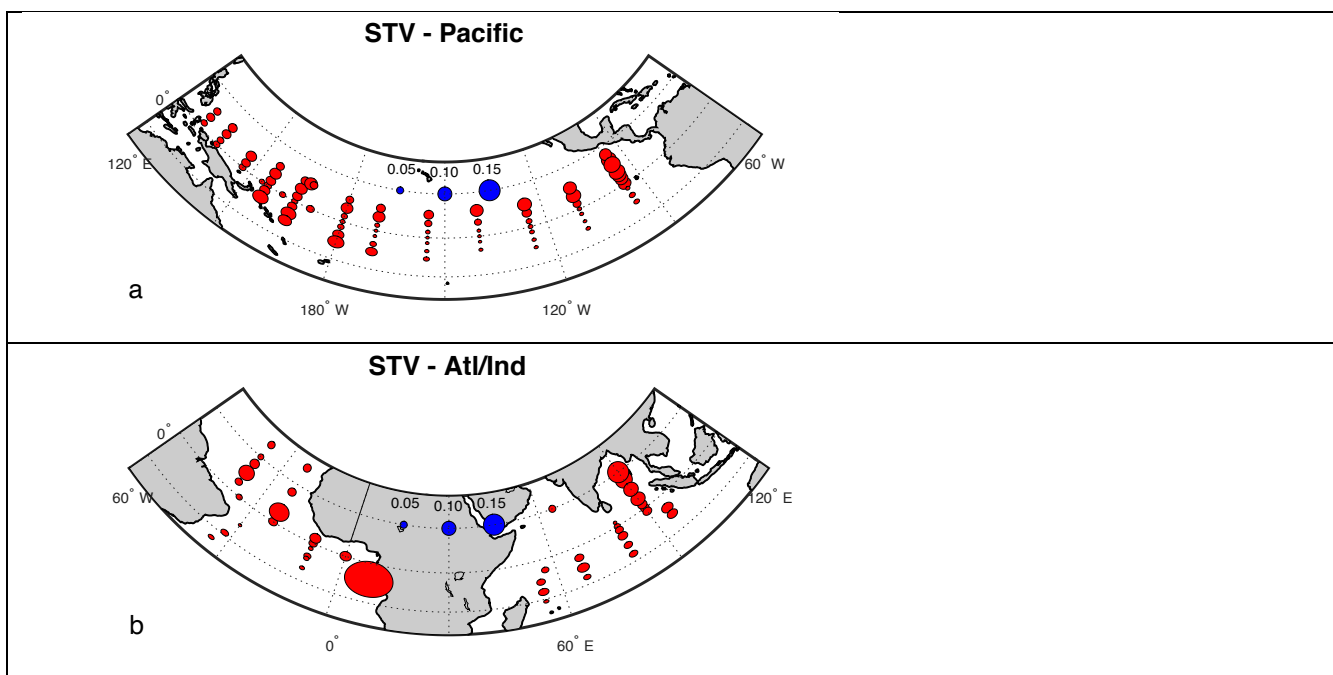
Figure 3: Median STV for each mooring for the a) Pacific basin and b) Atlantic and Indian basins. The sizes of the circles indicate the magnitude of the STV, with scale shown as blue circles near the middle of each panel.
