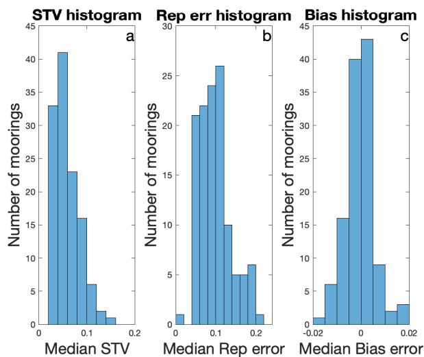
Figure 4: a) Histogram of the median STV values shown in Figure 3. One mooring is not included in this figure, an outlier with STV \approx 0.3 – the large symbol near the coast of Africa in Figure 2. b) As in panel a, but for median representation error shown in Figure 5. c) As in panel a, but for bias error. Positive bias error means instantaneous value greater than short-term mean. Note panels b) and c) rely on choosing random values from each short-term ensemble. This was done a number of times with different random values with only minor differences in results. Also note, the distributions depicted here included a small number of outliers that are not shown for clarity. Note the different x-axis limits in panel c.
