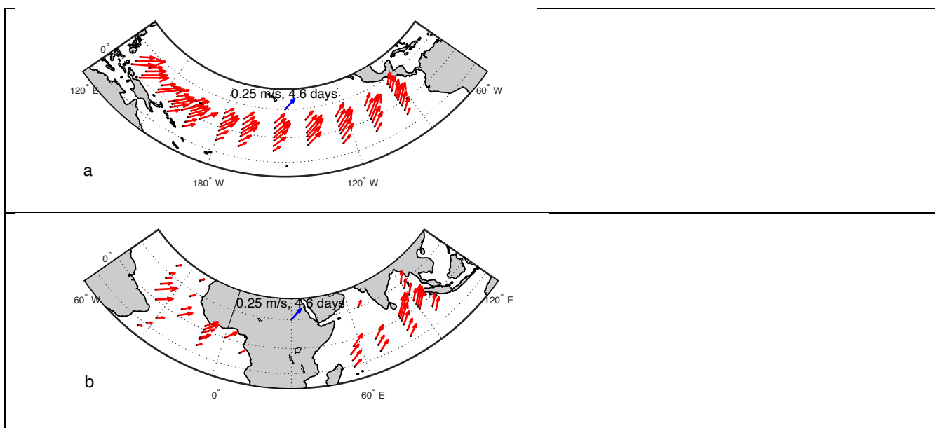
Figure 1: Small black dots: GTMBA mooring locations. Red arrows: Mean OSCAR current speed over the 1992-2020 time period at each mooring location. Arrow lengths indicate the average speed, with a scale arrow in blue at the top center. The length of the scale arrow corresponds to 25 cm/s. At that speed, it takes 4.6 days to go 100 km. Thus, the arrow length also corresponds to the time span used in computation of short-term variability discussed in the text. A shorter arrow (slower speed) means a longer time span. The directions of the arrows have no meaning. a) Pacific basin. b) Atlantic and Indian basins.
