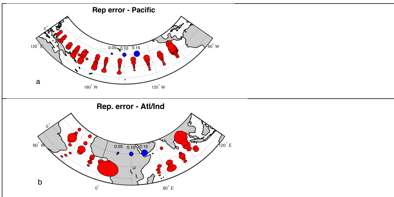
Figure 5: Representation error at each mooring. That is, RMS difference between random samples and short-term mean values. a) Pacific basin and b) Atlantic and Indian basins. The sizes of the circles indicate the magnitude of the RE, with scale shown as blue circles near the middle of each panel.
