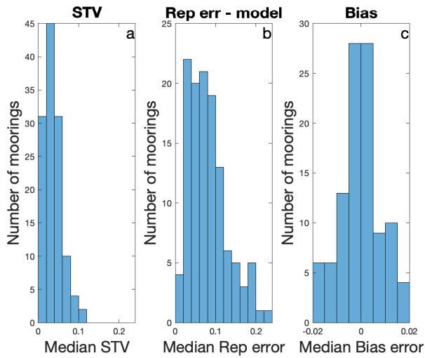
Figure 8: As in Figure 4, but for values computed from the MITgcm.
