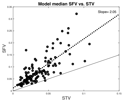
Figure 11: Median model SFV vs. model STV at each mooring location. Each symbol represents one mooring. The light line has a slope of 1. The dashed black line is a least-squares fit to the data shown, with the slope indicated at the top right.
