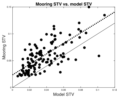
510 Figure 9: Model STV vs. mooring STV. Each symbol represents the median STV for one mooring. A couple of outlier points have been omitted for clarity. The dashed line is a least-squares fit to the data. It has a slope of about 1 and an intercept of about 0.02. The light black line has a slope of 1. This plot indicates that the mooring STV is generally larger than the model STV.
