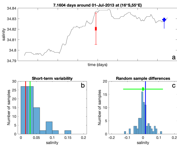
460 Figure 2: An example of how the STV is computed as explained in the text. a) A ~7-day piece of SSS record from the indicated mooring. The mean value is shown by the red “X”, with red bars being \pm 1 standard deviation. The blue “X” is a random value picked from the record. The blue line shows the difference between it and the mean value. b) The distribution of STV from the entire record at this mooring. One value is given by the standard deviation from panel a, and is the same as the red bar in panel b. The 465 median of the values in this distribution is indicated by the green bar. This is the single number from this mooring that is shown as STV in Figure 4a. c) Distribution of differences between random samples and mean values. One value is given by the blue line in panel a, and is the same as the blue bar in panel c. The RMS of this distribution is shown by the green bars, which is the mean \pm the RMS. These bars are the single value of RE that is shown for this mooring in Figure 4b.
