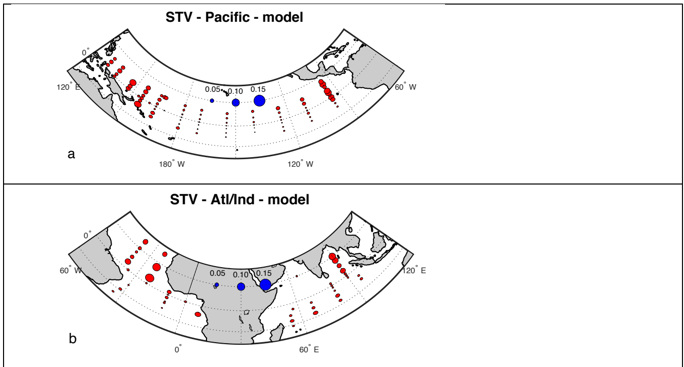
500 Figure 7: As in Figure 3, but for STV computed from the MITgcm. a) Pacific basin and b) Atlantic and Indian basins.
