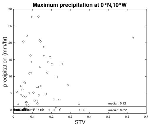
Figure 10: An example of how STV relates to precipitation at one mooring location. Maximum hourly precipitation for each short-term ensemble for the mooring at (0°N,10°W) vs. STV for the same set of ensembles. The light line indicates rain rate of 1 mm/hr separating rainy periods from non-rainy ones. Median values for all ensembles with maximum precipitation less than 1 mm/hr (below the line) and greater than or equal to 1 mm/hr (above the line) are shown at bottom right. These indicate that STV tends to be greater when there is rainfall. However, there is not a clear correlation between rainfall and STV. This pattern was consistent in most of the GTMBA moorings with precipitation records.
