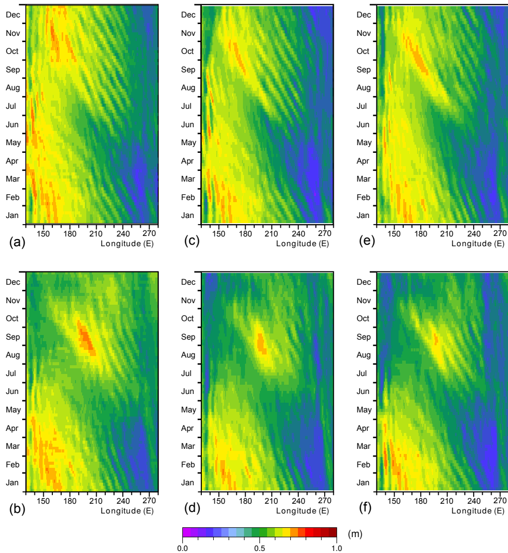
Figure 5. Hovmöller diagrams of sea level (m) at 6^{\circ}\text{N} in the Pacific for (a) Nemo model in 1981, (b) Nemo in 1982, (c) Occam starting January 1981, (d) Occam starting January 1982, (e) Occam starting January 1982 but with 1981 winds, (f) Occam starting January 1981 but with 1982 winds. The figures are based on 1^{\circ} averages of the model data.
