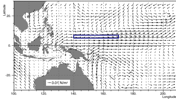
Figure 8. Wind-Mean wind stress vector anomaly ( \text{Nm}^{-2} ), for the period 16th March to the 8th August 1982 relative to the same period in 1981. The blue rectangle shows the region between 140^{\circ}\text{E} and 170^{\circ}\text{E} and between 5^{\circ}\text{N} and 7^{\circ}\text{N} .
