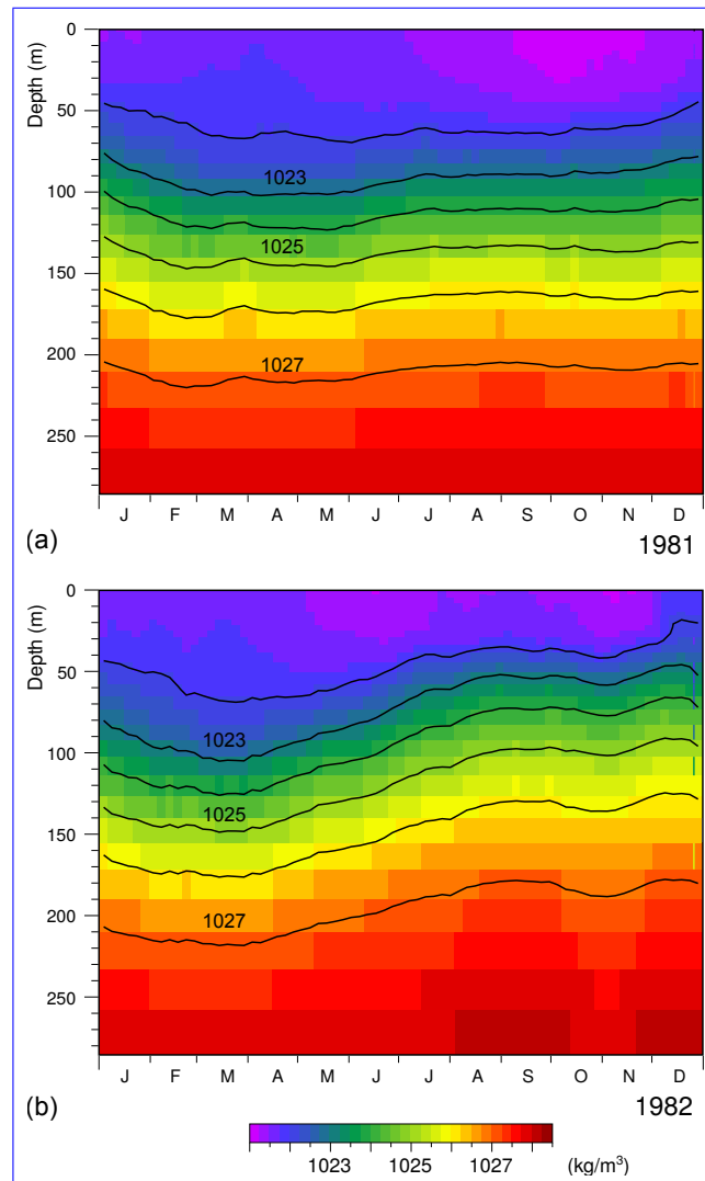
Figure 12. Nemo 1/12° model potential density averaged between 140°E and 170°E and between 5°N and 7°N, for (a) 1981 and (b) 1982. Contours at integer values of density ( \text{kg m}^{-3} ).
