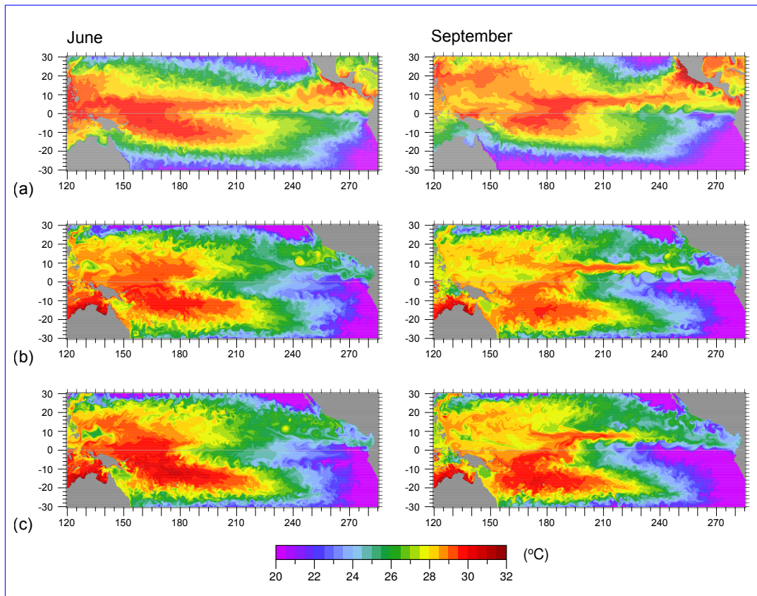
Figure 4. Surface temperature (°C) on the 6th June and 9th September for (a) Nemo in 1982, (b) Occam in 1982, started January 1982 (c) Occam in 1981, started January 1981 but with 1982 winds.
