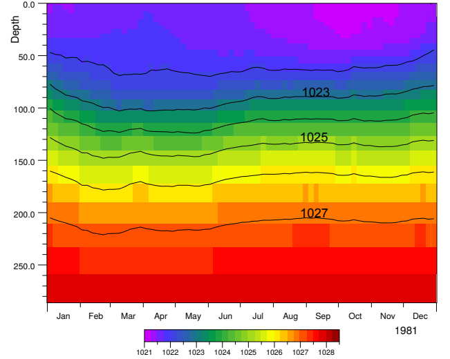
Figure 25. Nemo 1/12° model potential density during 1981, averaged between 140° E and 170° E and between 5° N and 7° N. Contours, interpolated from model layer values, at integer values of density ( \text{kg/m}^3 ).
