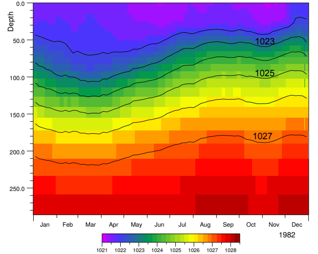
Figure 26. Nemo 1/12° model potential density during 1982, averaged between 140° E and 170° E and between 5° N and 7° N. Contours at integer values of density ( \text{kg/m}^3 ).
