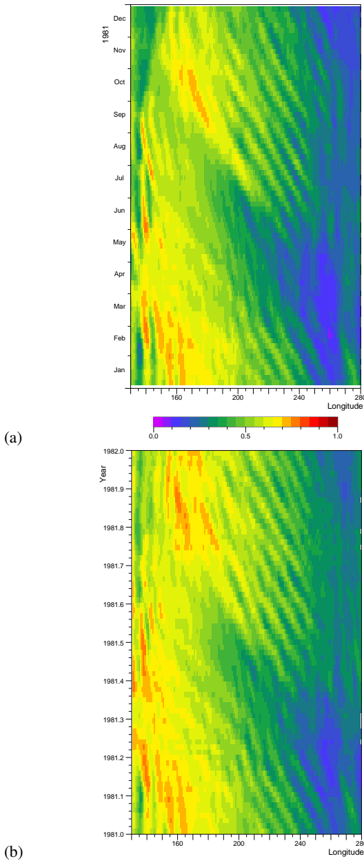
Figure 1. Hoffmuller diagram the sea level at 6° N in the Pacific for 1981, showing (a) sea level from the short Occam 1/4° model run and (b) from the Nemo 1/12° run. The figures are based on 1° averages of the model data.
