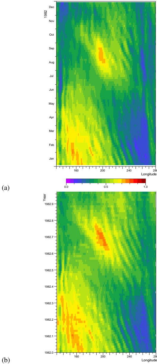
Figure 7. Hoffmuller diagram the sea level at 6° N in the Pacific for 1982, showing (a) sea level from the Occam run and (b) from the Nemo run.
