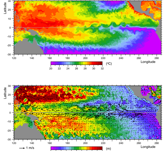
Figure 6. Plots of Nemo model SST, SSH and surface velocities from the average over the 5 days before the 2nd September 1981.
