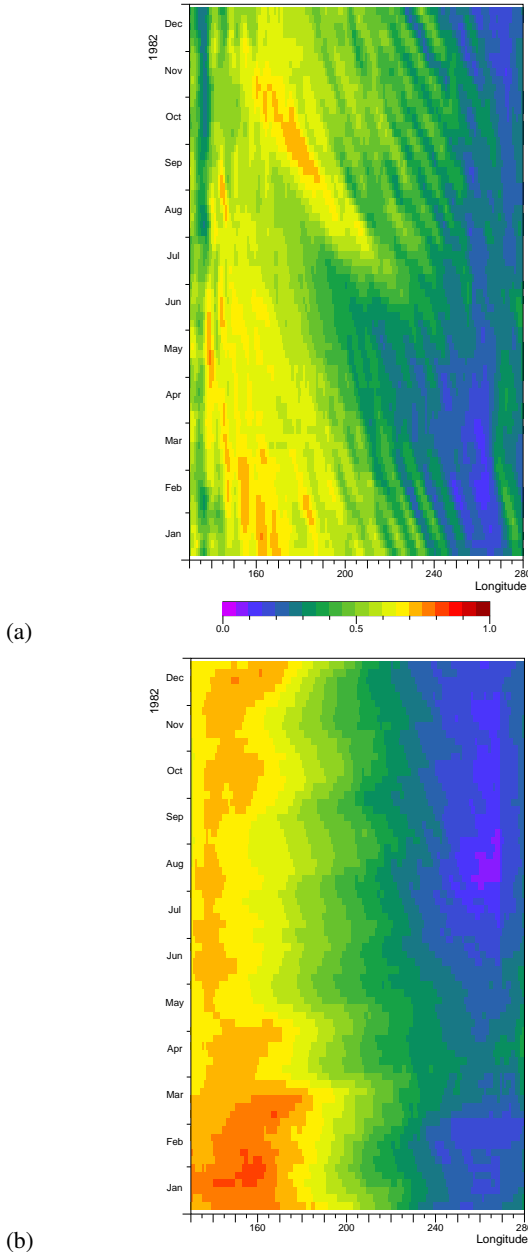
Figure 13. Hoffmuller diagram the sea level from the Occam model during 1982, when started from Nemo model archive for the 5th January 1982 but forced by 1981 winds for (above) 6° N and (below) at the Equator.
