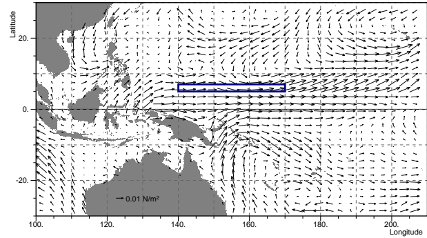
Figure 21. Wind stress vector anomaly, for the period 16th March to the 8th August 1982 relative to the same period in 1981. The blue rectangle shows the region between 140^\circ E and 170^\circ E and between 5^\circ N and 7^\circ N.
