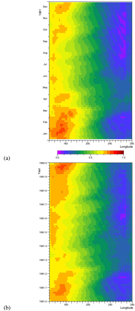
Figure 2. Hoffmuller diagram the sea level on the Equator in the Pacific for 1981, showing (a) sea level from the short Occam 1/4° model and (b) from the Nemo 1/12° run.
