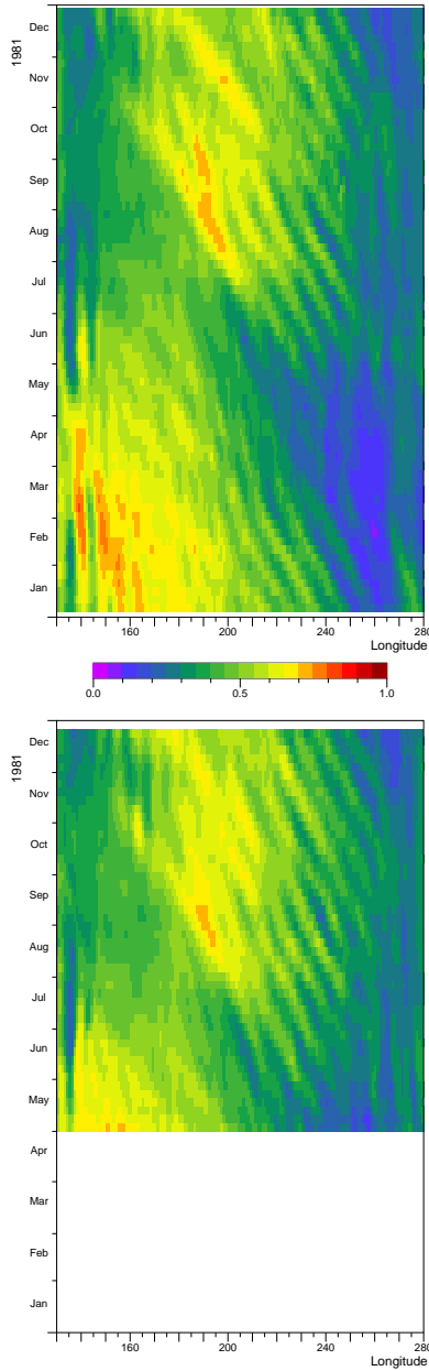
Figure 22. Hoffmuller diagram for the sea level at 6° N during 1981, forced by the combination of 1981 and 1982 winds described in the main text when started from the NEMO archive for (above) 5th January 1981, (below) 30th April 1981. [Review version: Left and right.]
