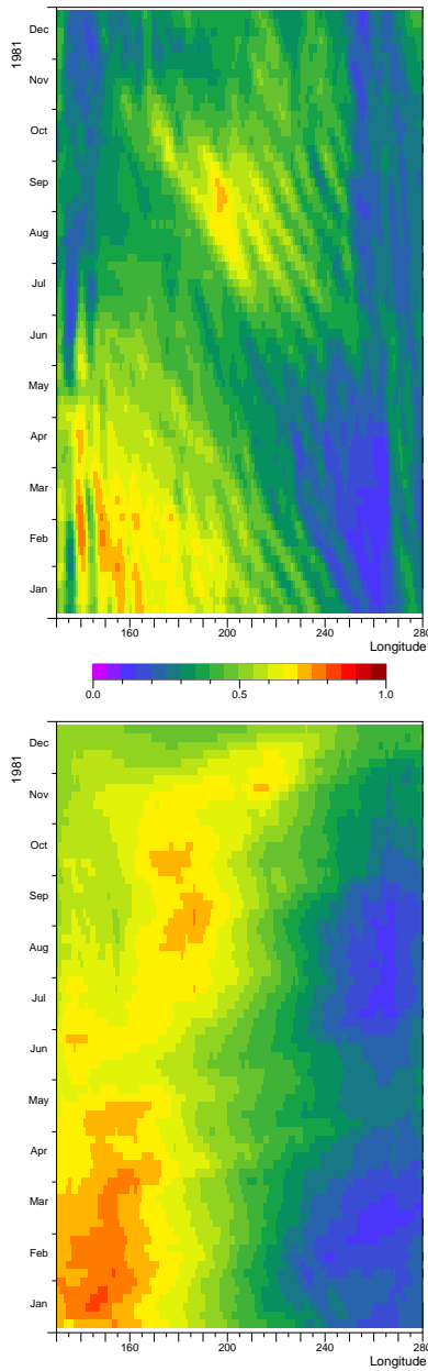
Figure 16. Hoffmuller diagram the sea level from the Occam model during 1981, when started from the Nemo model archive from the 5th January 1981 but forced by 1982 winds for (above) 6° N and (below) at the Equator. [Review version: Left and right when single column]
