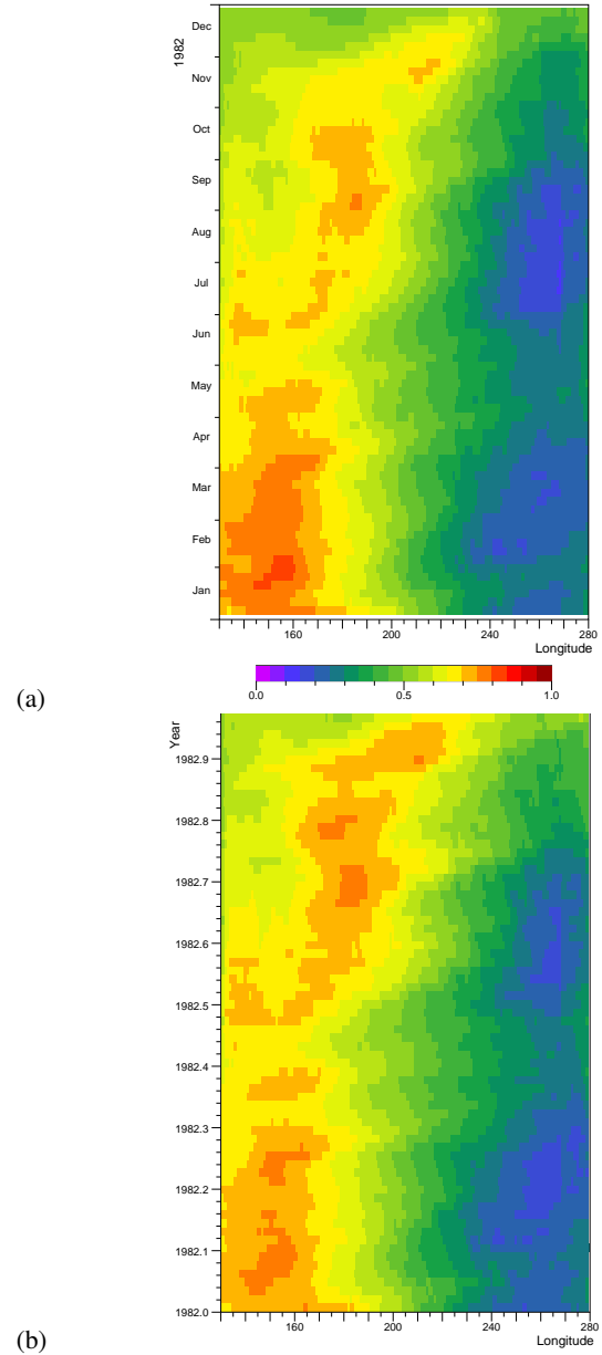
Figure 8. Hoffmuller diagram the sea level on the Equator in the Pacific for 1982, showing (a) sea level from the Occam run and (b) from the Nemo run.
