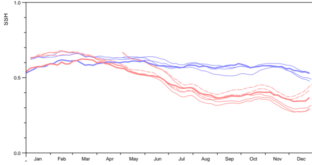
Figure 23. Sea level in the different runs averaged between 140° E and 170° E and between 5° N and 7° N. Red lines correspond to runs forced by 1982 winds, blue to 1981 winds. Thick lines are from the original Nemo run, thin lines are from the occam runs. The dashed lines corresponds to the runs started in 1981 but with 1982 winds only in the western Pacific.
