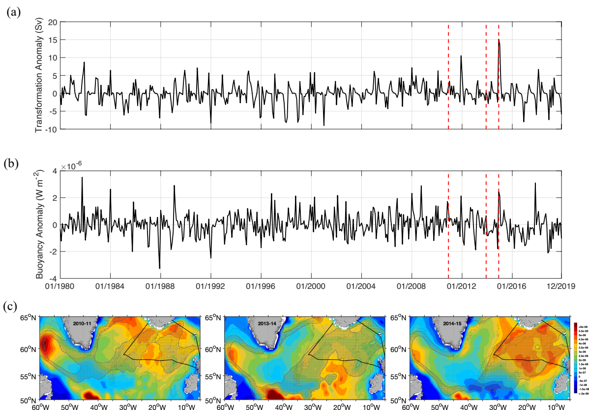
295 Figure 6. (a) Transformation anomaly at the SPMW isopycnal 27.4 \text{ kg m}^{-3} between 1980 and 2019. (b) Buoyancy anomaly over the Iceland Basin between 1980 and 2019; Dashed red lines indicate transformation and buoyancy anomalies on December 2010, 2013 and 2014. (c) Maps of buoyancy forcing superimposed by the surface density area 27.3\text{--}27.5 \text{ kg m}^{-3} in grey during winter (December to April) of three different years.
