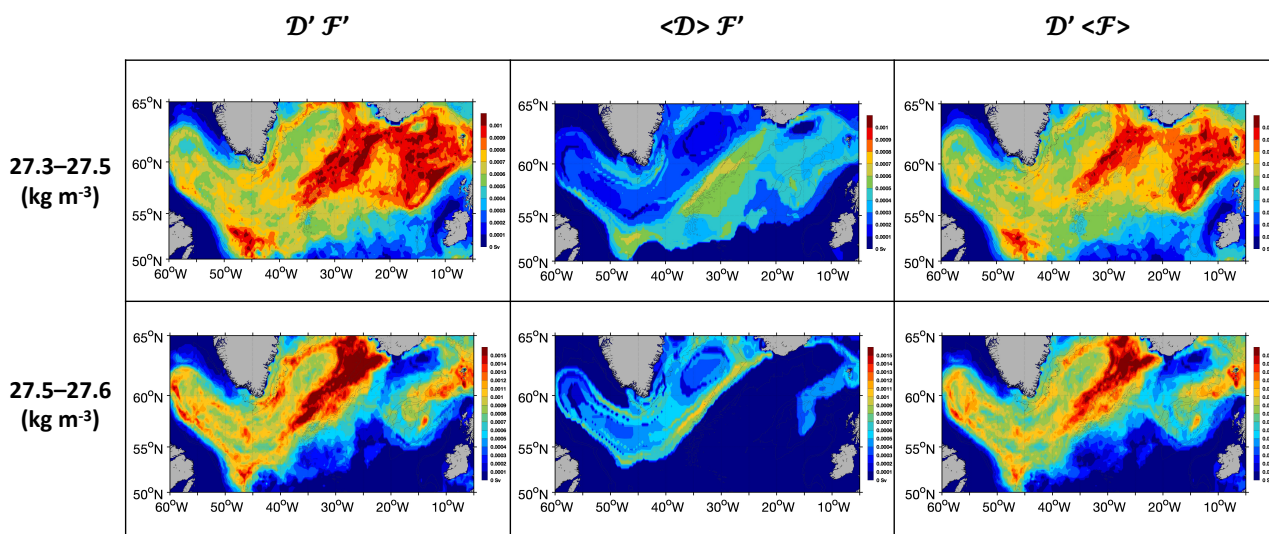
Figure 4. Sensitivity experiments of the variance in transformation estimated as the standard deviation of the yearly transformation integrated over the density range (upper row) 27.3–27.5 kg m -3 and (lower row) 27.5–27.6 kg m -3 layers during 1980–2019. The left column shows the variance in transformation estimated from monthly variable surface density ( D' ) and air-sea fluxes ( F' ); the middle column shows the variance in transformation estimated from monthly variable heat and freshwater fluxes ( F' ) and climatological surface density ( \langle D \rangle ); the right column shows the variance in transformation estimated from monthly variable surface density ( D' ) and climatological heat and freshwater fluxes ( \langle F \rangle ). Variable and climatological density at surface stand for variable and climatological salinity and temperature at surface.
