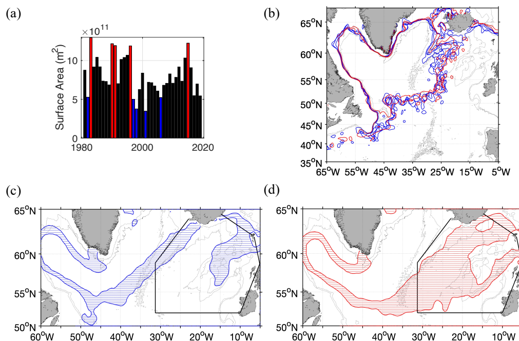
Figure 7. (a) Surface density area (m 2 ) in winter (December to April) for density higher than 27.3 kg m -3 over the black box indicated in panel (c). (b) Subpolar gyre boundaries in January during years indicated by the color code. (c)-(d) Surface density area 27.3–27.5 kg m -3 averaged during winter (December to April) of the years indicated by the color code.
