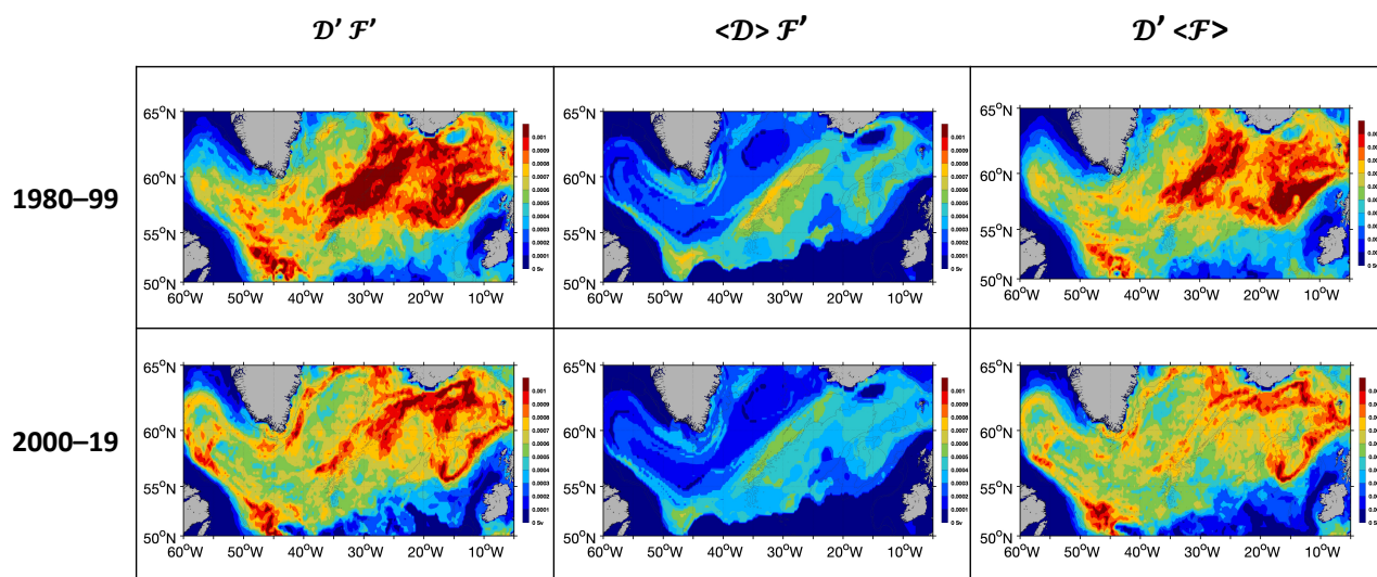
Figure 5. Same as in Fig. 4 for the density range 27.3–27.5 kg m -3 , but integrated over different periods of time.
