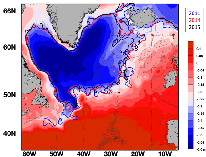
360 Figure A1. Time-mean SSH of the subpolar gyre (1993–2015) with contour interval of 5 cm. Contours in color indicate the subpolar gyre boundaries in January 2011, 2014 and 2015 defined with the 1-cm contour intervals of the monthly SSH field.
