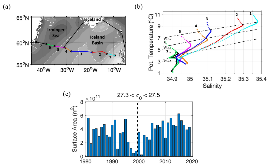
Figure 1. (a) Sea surface density ( \text{kg m}^{-3} ) averaged over winter (December to April) 1980–2019; contour interval is 0.1\text{ kg m}^{-3} . White dashed lines outline the isopycnals 27.3 and 27.5\text{ kg m}^{-3} . The OSNAP East section, divided into 7 coloured subsections, forms the southern boundary of closed domain for our study. (b) Potential temperature/salinity diagram at OSNAP East averaged over 2014–2018 for (from east to west) the three northward branches of the North Atlantic Current (NAC) in the Iceland Basin (1–3); southward East Reykjanes 95 Ridge Current (4); northward Irminger Current (5); northward Irminger Gyre (6) and southward East Greenland Current (7). Dashed black lines show the potential densities \sigma_0 = 27.3, 27.5 and 27.74\text{ kg m}^{-3} . (c) Surface area ( \text{m}^2 ) over the Iceland Basin in January.
