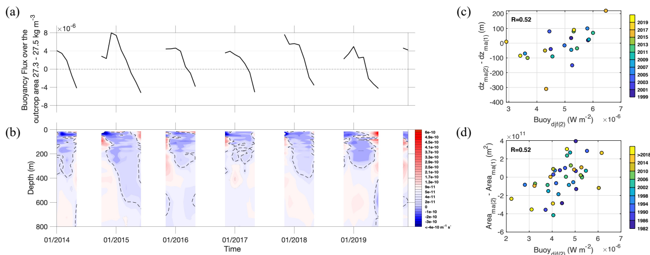
185 Figure 2. (a) Buoyancy flux ( \text{W m}^{-2} ) and (b) potential vorticity ( \text{m}^{-1} \text{ s}^{-1} ) averaged over the source density area in the Iceland Basin. The isopycnals 27.3 and 27.5 \text{kg m}^{-3} do not outcrop over the Iceland Basin during summer. The dashed black line shows the potential vorticity 4 \times 10^{-11} \text{ m}^{-1} \text{ s}^{-1} . (c) Correlations between the buoyancy flux averaged over December–January–February in the second winter ( \text{Buoy}_{\text{dj}(f(2))} ), and the difference in SPMW thickness March–April between the end of the first ( \text{dz}_{\text{ma}(1)} ) and second ( \text{dz}_{\text{ma}(2)} ) winters over 1999–2019. The SPMW thickness was estimated by the depth of the potential vorticity isoline 4 \times 10^{-11} \text{ m}^{-1} \text{ s}^{-1} over the source water area (as shown in Fig. 2b). EN4.2.1 data before 1999 are not used because of large uncertainties due to scarce observations at depth. (d) Correlation between the buoyancy flux averaged over December–January–February in the second winter ( \text{Buoy}_{\text{dj}(f(2))} ), and the difference in surface area between the end of the first ( \text{area}_{\text{ma}(1)} ) and second winters ( \text{area}_{\text{ma}(2)} ).
