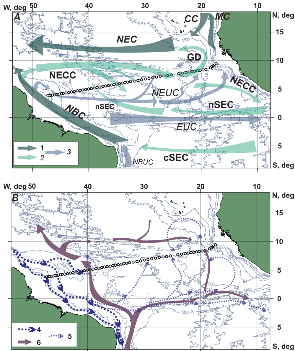
Figure 2. Generalized circulation schematics within the study area: surface and subsurface layers (A) and deep and bottom layers (B), where 1 — surface currents (from 0 up to 100 m), 2 — subsurface currents (from 100 up to 500 m), 3 — joint surface and subsurface currents (from 0 up to 500 m), 4 — the Deep Western Boundary Current (DWBC) cores, 5 — schematic Deep Western Boundary Current recirculation, 6 — Antarctic Bottom Water. The references and current abbreviations are explained in the text. White circles — Ioffe-2000 transect stations.
