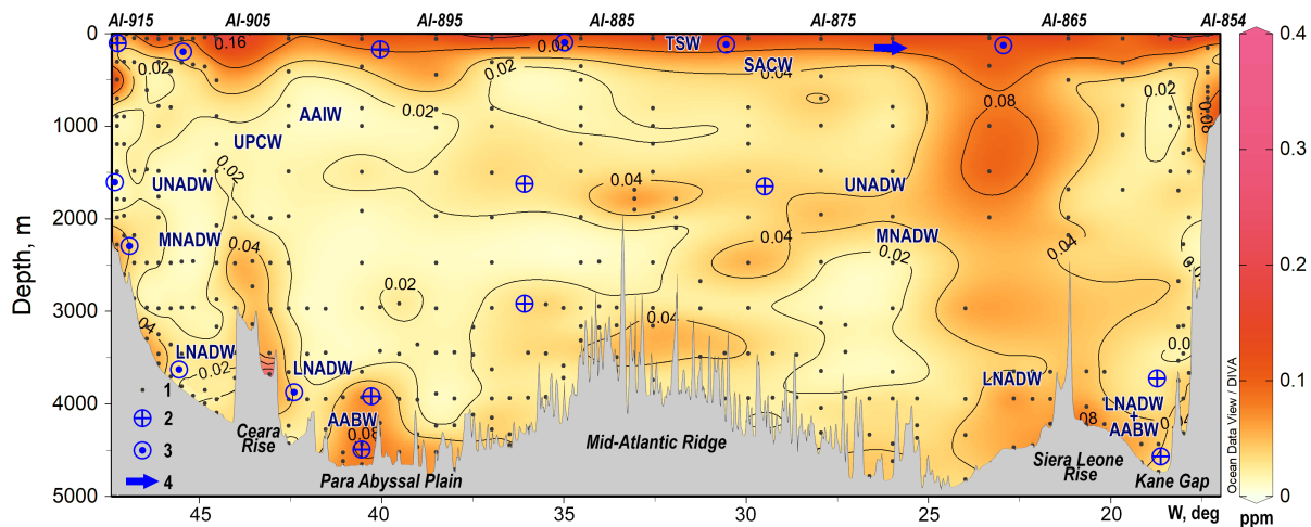
Figure 4. Distribution of the SPM volume concentration (ppm) on the Ioffe-2000 transect, done with Ocean Data View (Schlitzer, 2018). Numbers indicated in panel bottom left: 1 — sampling points, 2 — northward current, 3 — southward current, 4 — eastward current. Isolines are in geometric progression, for water mass abbreviations see text. Bottom topography from Sokov et al. (2002). The interpolation was done via the DIVA gridding (Barth et al., 2010) with 25 permille X-scale length and 65 permille Y-scale length.
