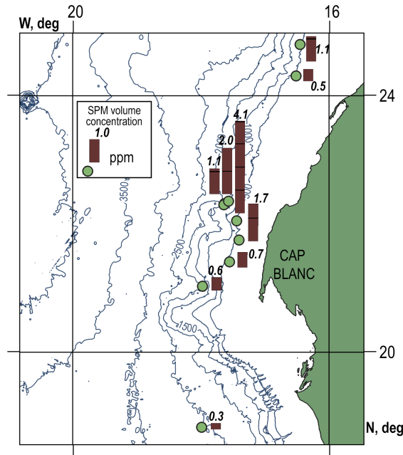
Figure 5. Schematic distribution of surface SPM concentrations (ppm) in the Northwest African upwelling area prior to the Ioffe-2000 transect. Isobaths every 500 m.
