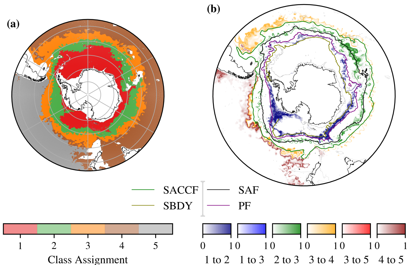
Figure 4. (a) The cluster assignments with K = 5 and (b) I-metric for specific class transitions. This view highlights the transitions between specific classes; the transitions have some similarities with respect to the altimetric fronts shown overlaid from Kim and Orsi (2014) (SBDY: Southern boundary, SACCF: Southern ACC front, PF: Polar front, SAF: Sub-Antarctic front). Data from June 2011 as a representative month.
