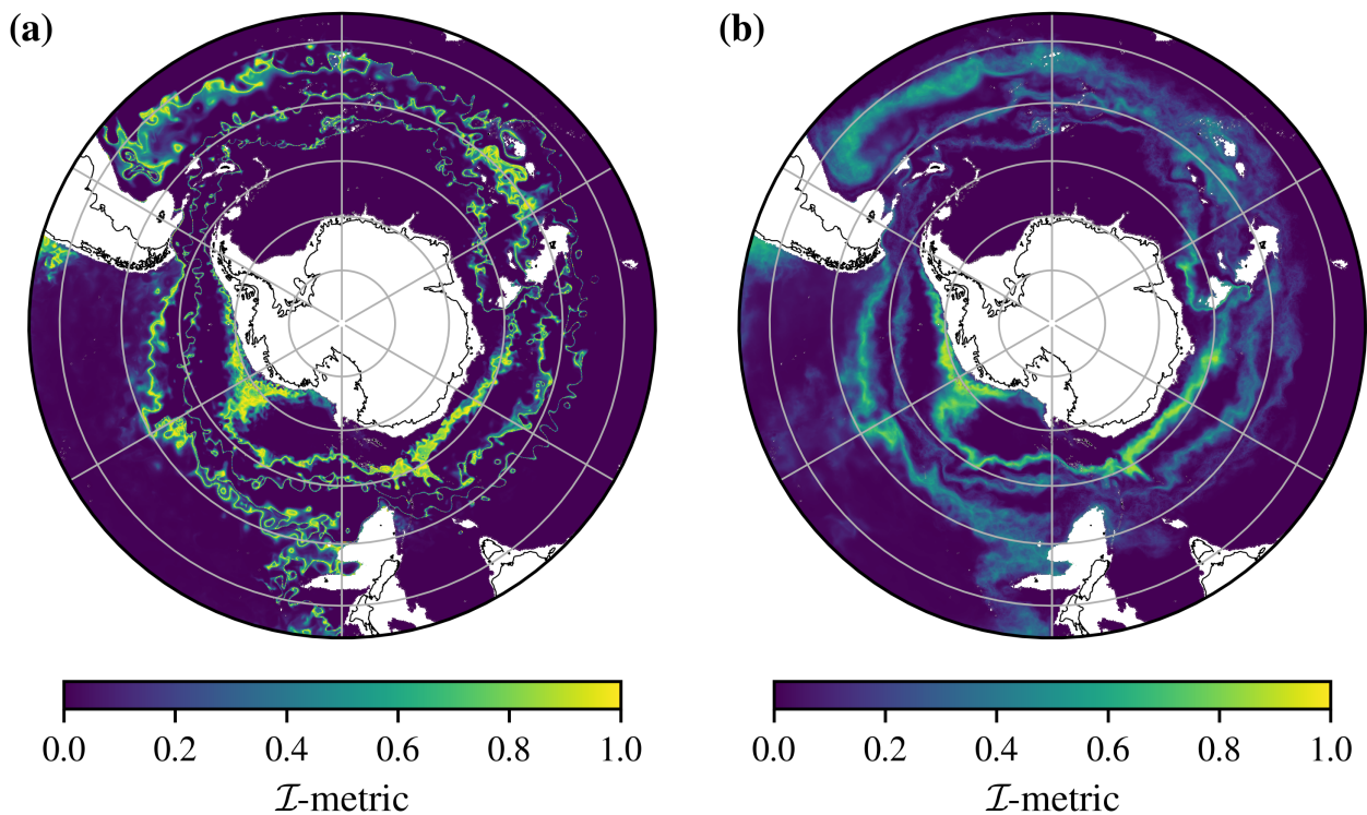
Figure 3. The I -metric highlights transitions between coherent thermohaline regimes in geographical space. (a) is the I -metric for a single month (April 2012) and (b) for the time average of the BSOSE-i106 dataset (60 months). Latitude lines are shown between 80^{\circ}\text{S} and 40^{\circ}\text{S} every 10^{\circ} , and longitude lines are shown every 60^{\circ} . Animations showing month-to-month and interannual variability are available in the software release (Thomas, 2021).
