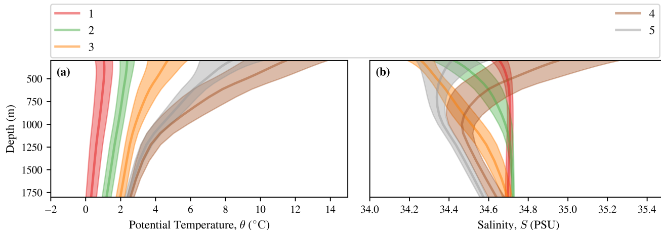
Figure 5. Profiles of the five GMM clusters between 300 m and 1800 m in (a) temperature and (b) salinity, for the training data, with one standard deviation envelope either side plotted.
