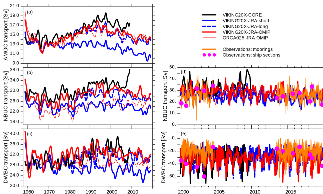
Figure 17. Time series of interannually filtered (a) AMOC, (b) NBUC and (c) DWBC transports at 11°S; monthly averages of positive (NNE-ward) NBUC and negative (SSW-ward) DWBC transports (see Table 7 for details of the definitions) are given in (d) and (e) together with mooring based (orange curves; thick monthly, thin 2.5-day averages) and ship based observations (purple dots)
