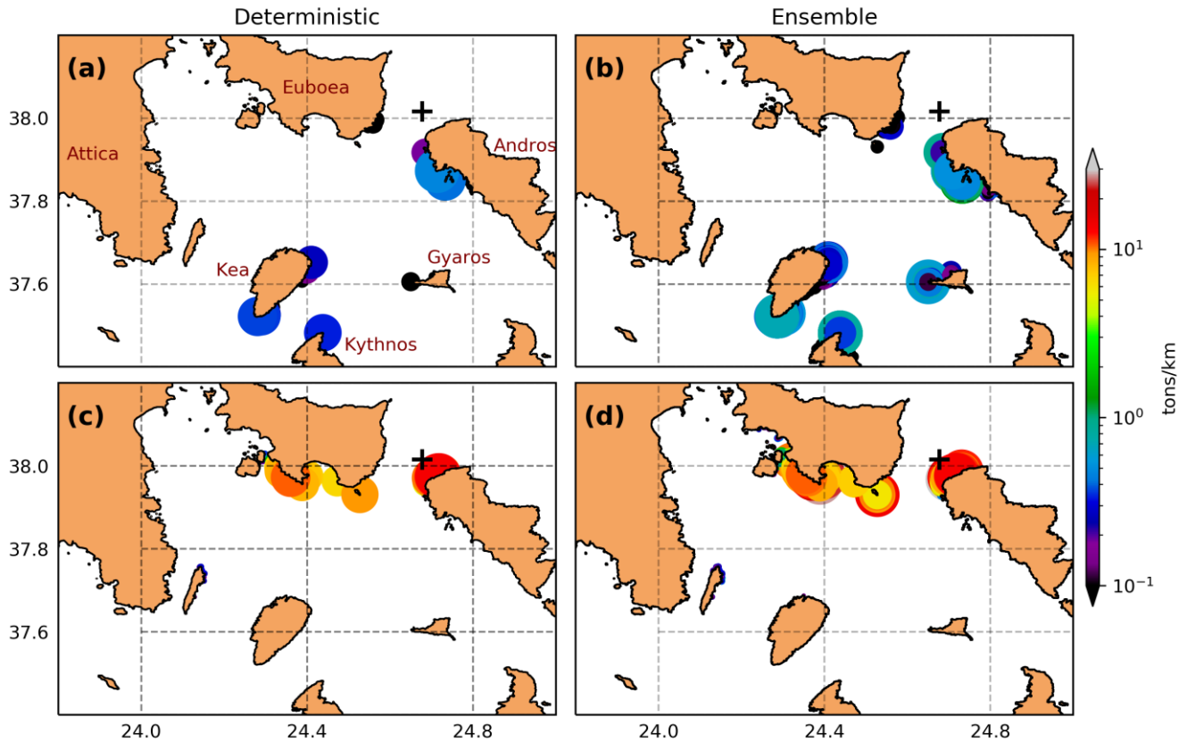
345 Figure 11: Beached oil concentrations (API 31; tons/km) at the end of the run, i.e. forecast time 168-hour, during (a-b) winter and (c-d) spring, for the (a, c) deterministic and the (b, d) ensemble considering all members.
