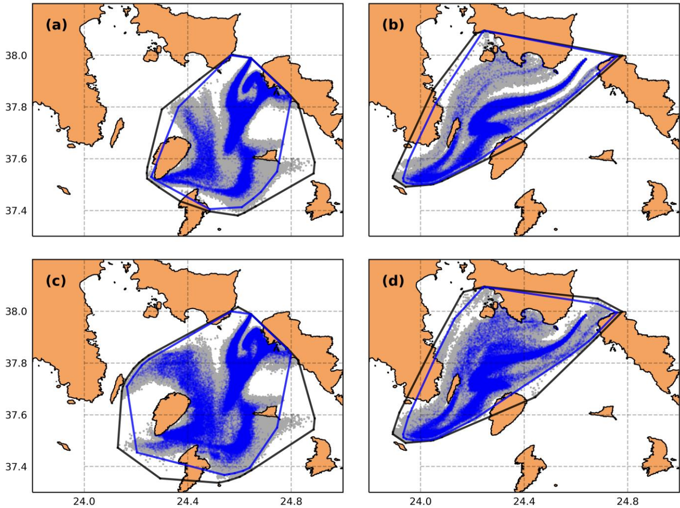
285 Figure 8: Convex hulls of the deterministic (blue dots/outer-line) and all ensemble members (grey dots/outer-line), considering only surface and oil parcels deposited at the coasts (API 31), with forecast time 168-hour in (a) winter and (b) spring; (c, d) same considering all parcels (i.e. surface, subsurface and oil parcels deposited on the seabed and at the coasts).
