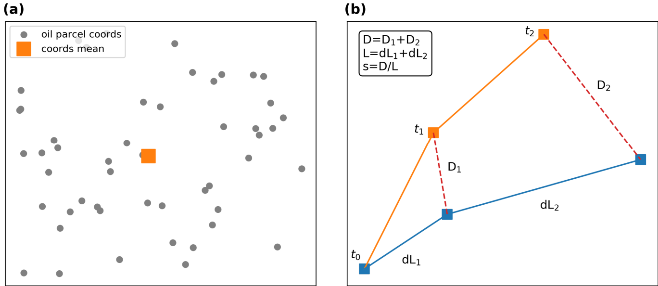
225 Figure 6: Schematic of (a) spatially weighted mean (orange square) of oil spill particles (grey dots), (b) mean oil spill trajectories (following the geographically weighted mean) between the deterministic (blue line) and an individual member of the ensemble (orange line), and their corresponding distances (red dashed lines) evolving over time.
