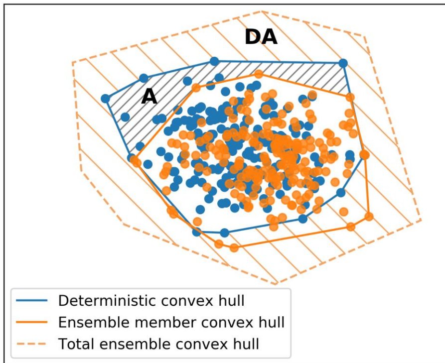
195 Figure 5: Schematic of convex hull areas (blue/orange solid outer-lines) for the deterministic oil spill particles and an individual member of the ensemble (blue/orange dots). The orange dashed outer-line shows the convex hull of the whole ensemble including all members. The orange hatched area DA shows the difference between the whole ensemble convex hull exceeding the deterministic
