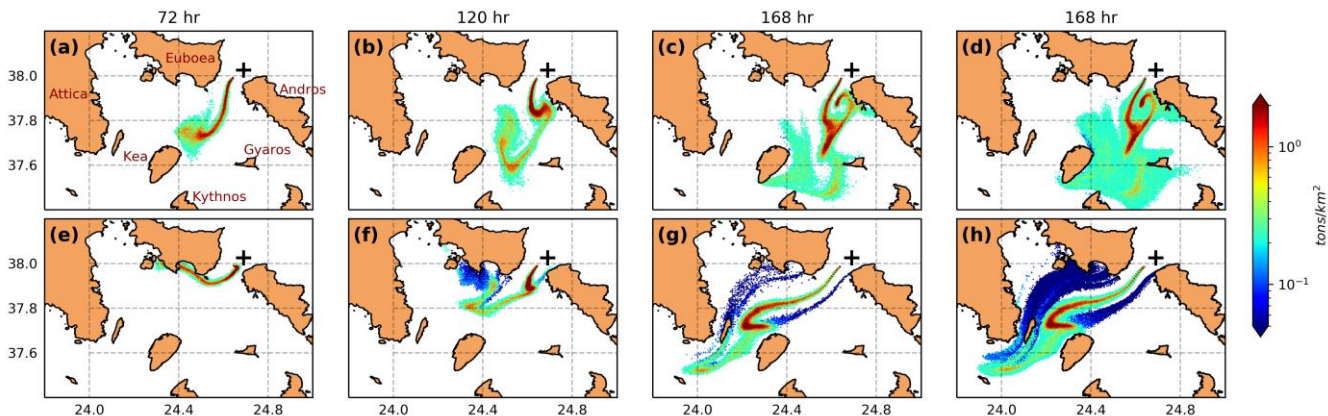
260 Figure 7: Surface oil concentrations (API 31; tons/km 2 ) of the deterministic simulation for (a-c) winter and (e-g) spring, at forecast times 72, 120 and 168 hours; (d, h) same considering all members of the ensemble at forecast time 168-hour.
