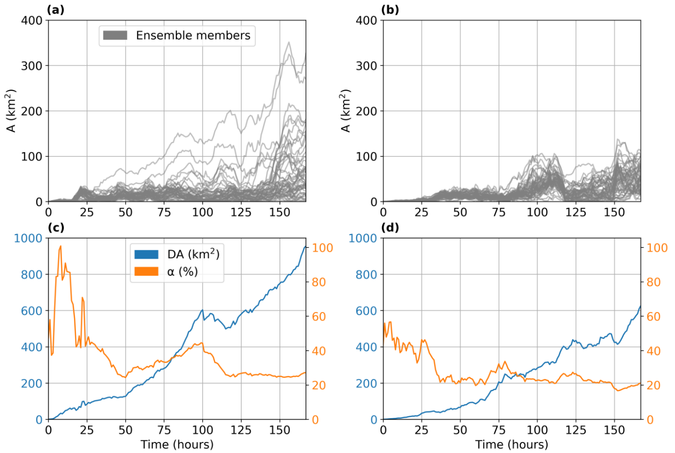
320 Figure 9: Area of the deterministic convex hull that exceeds the area of each member ( A in \text{km}^2 ; grey lines) for (a) winter and (b) spring, as a function of the forecast time. DA extent (units in \text{km}^2 ; blue line) of the ensemble convex hull area with respect to the deterministic state and percentage of change, \alpha (%; orange line), for (c) winter and (d) spring. Oil type API 31.
