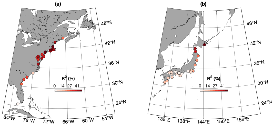
Figure S7. The adjusted coefficient of determination R_{Adj}^2 obtained for the (a) Atlantic and (b) Pacific gauges. This quantity indicates how much does the best subset regression explain of the monthly sea level.
