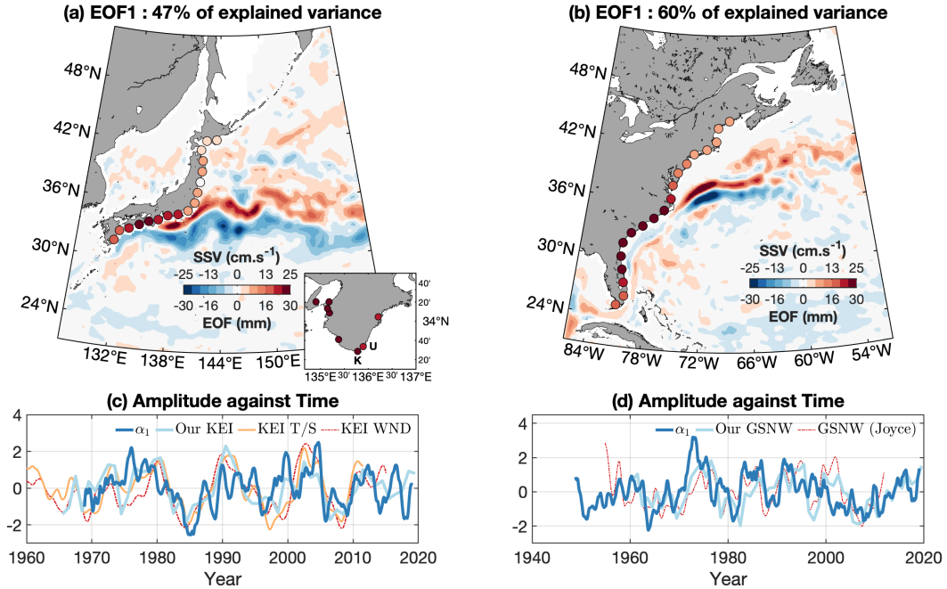
Figure 5. (a) and (b) present the leading EOF ( \phi_1 ) of the gridded, tide gauge obtained based, sea-level anomaly (circular markers) from the Pacific (a) and (b) present, for the Pacific and Atlantic respectively, the (b). The associated principal components \alpha_1 's (solid are shown as thick dark blue lines for the Pacific (c) and Atlantic (d) respectively, together with indices of WBC extension meridional location: this study and Qiu et al. (2016) T/S-based and wind-based KEIs (on (c), thick light blue line), Qiu et al. (2016) T/S-based (thin orange solid line) and wind-based (thin dot-dashed red line) KEIs, and this study and Joyce et al. (2000) GSNWs (on (d), thick light blue line and dot-dashed thin red line, respectively). All quantities timeseries on (c) and (d) are normalized. Colour shadings on (a) and (b) are, for each basin, the sea surface velocity magnitude composites difference based on the principal component \alpha_1 (period of \alpha_1 > +2/3 minus period of \alpha_1 < -2/3 ). The arbitrary threshold of \pm 2/3 was used, but taking any number between zero and one leads to akin patterns. The inset on (a) presents the regression coefficient obtained when the principal component is regressed on the original tide gauges, with a zoom in on the Kii peninsula.
