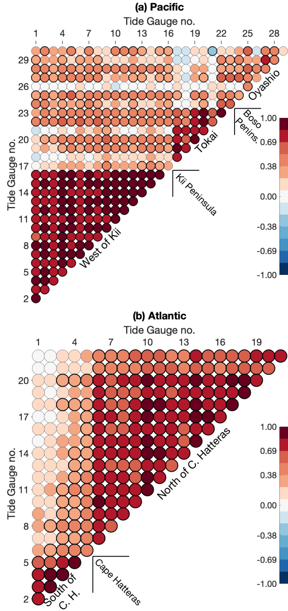
Figure 3. (a) Pacific and (b) Atlantic tide gauge cross-correlation at zero-lag. Each circular marker gives the the correlation r_{ij} , between gauge i and gauge j . Tide gauge-gauges are numbered in ascending order from south to north, following the coastline ( a list is given in Supplementary Table S1 and Supplementary Table S2 ). Bolder circular contour indicates that the correlation is above significance level of 95%.
