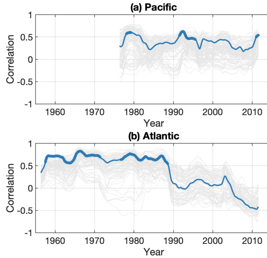
Figure 4. Moving correlation analysis between the tide gauges records with a running window of 15 years. Each individual grey line renders the moving correlation between two records. The x-axis represents the center of the moving window. (a) Cross correlation between the Oyashio group and West-west of Kii groupings (grey lines). (b) Cross-correlation between gauges on either side of the Cape Hatteras, the separation point of the Gulf Stream (again, grey lines). On each panel, the solid blue line is the moving correlation between the group averages of sea-level anomalies. Significant correlations above 95% level are indicated by thicker blue line.
