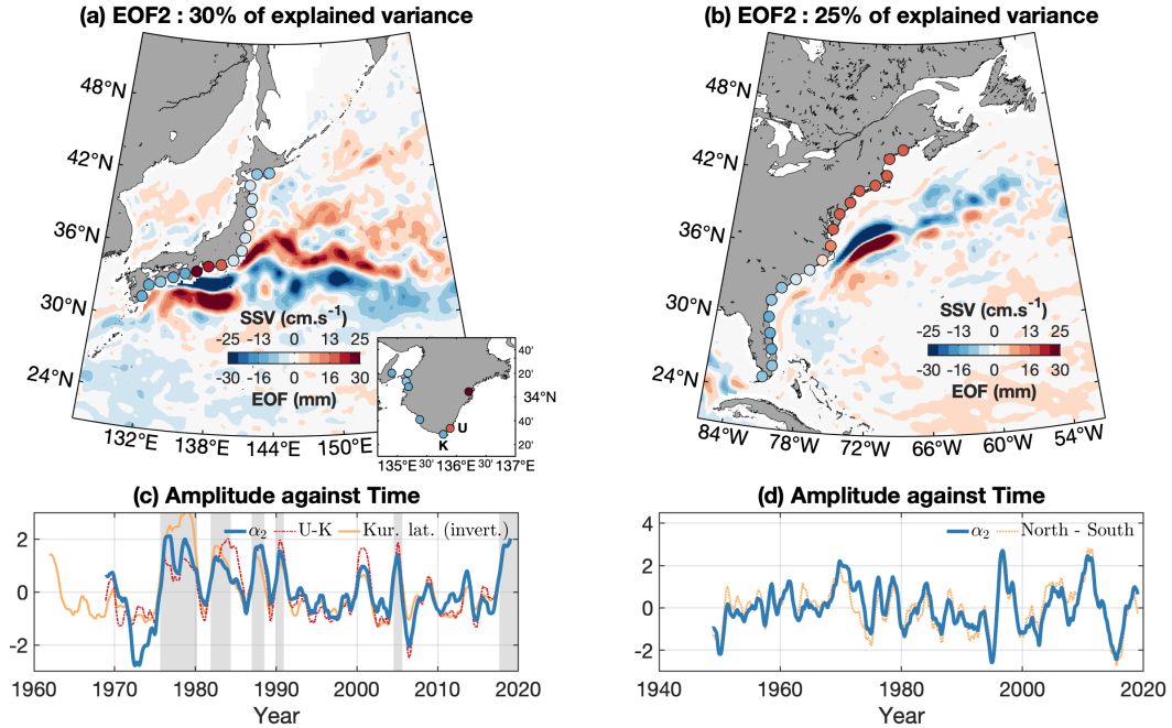
Figure 6. (a) and (b) present the The second EOF ( \phi_2 ) of the gridded, tide gauge obtained based, sea-level anomaly (circular markers) -from the Pacific (ea) and (d) present, for the Pacific and Atlantic respectively, the (b). The associated principal components \alpha_2 's (solid are shown as thick dark blue lines for the Pacific (c) and Atlantic (d) respectively). Also on (c), the Kuroshio southernmost latitude South-south of Tōkai is represented with the solid orange line (positive values indicate Kuroshio further to the south), the difference between sea level at Uragami and Kushimoto with the dot-dashed red line, and grey shadings represent periods of typical large meander (JMA, 2018). On (d), the dashed yellow line is the sea-level difference between the averages of northern and southern groupings of tide gauges, as in McCarthy et al. (2015). All timeseries on (c) and (d) are normalized. Colour shadings on (a) and (b) are, for each basin, the sea surface velocity magnitude composite difference based on the principal component \alpha_2 (period of \alpha_2 > +2/3 minus period of \alpha_2 < -2/3 ). The arbitrary threshold of \pm 2/3 was used, but taking any number between zero and one leads to akin patterns. The inset on (a) present-presents the regression coefficient obtained when the principal component is regressed on the original tide gauges, with a zoom in on the Kii peninsula.
