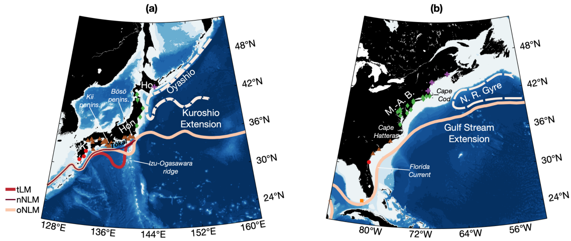
Figure 1. (a) Kuroshio region circulation: The three Kuroshio paths — the typical Large Meander (tLM), the near-shore nearshore Non-Large Meander (nNLM) and the offshore Non-Large Meander (oNLM) are indicated upstream of the Izu-Ogasawara Ridge. The mean location of the KE is indicated offshore of this point showing the location of the quasi-stationary meanders. The Oyashio current is shown in blue dashed pink . On land, K indicates Kyūshū, Hon stands for Honshū and Ho indicates Hokkaidō. (b) Gulf Stream region circulation from the Florida Current to the Gulf Stream Extension. The Northern Recirculation Gyre is also indicated. On land, M.-A. B. stands for Mid-Atlantic Bight and N.S. indicates Nova Scotia. Markers in (a) and (b) indicate the location of the tide gauges used in this study. The colour and shape of the markers in (a) and (b) indicate the angle used to rotate the wind stress in an alongshore/across-shore coordinate system for the removal of sea-level variability driven by local atmospheric effect (See Supplementary Table S1 and Supplementary Table S2). Shadings in (a) and (b) indicate bathymetry.
