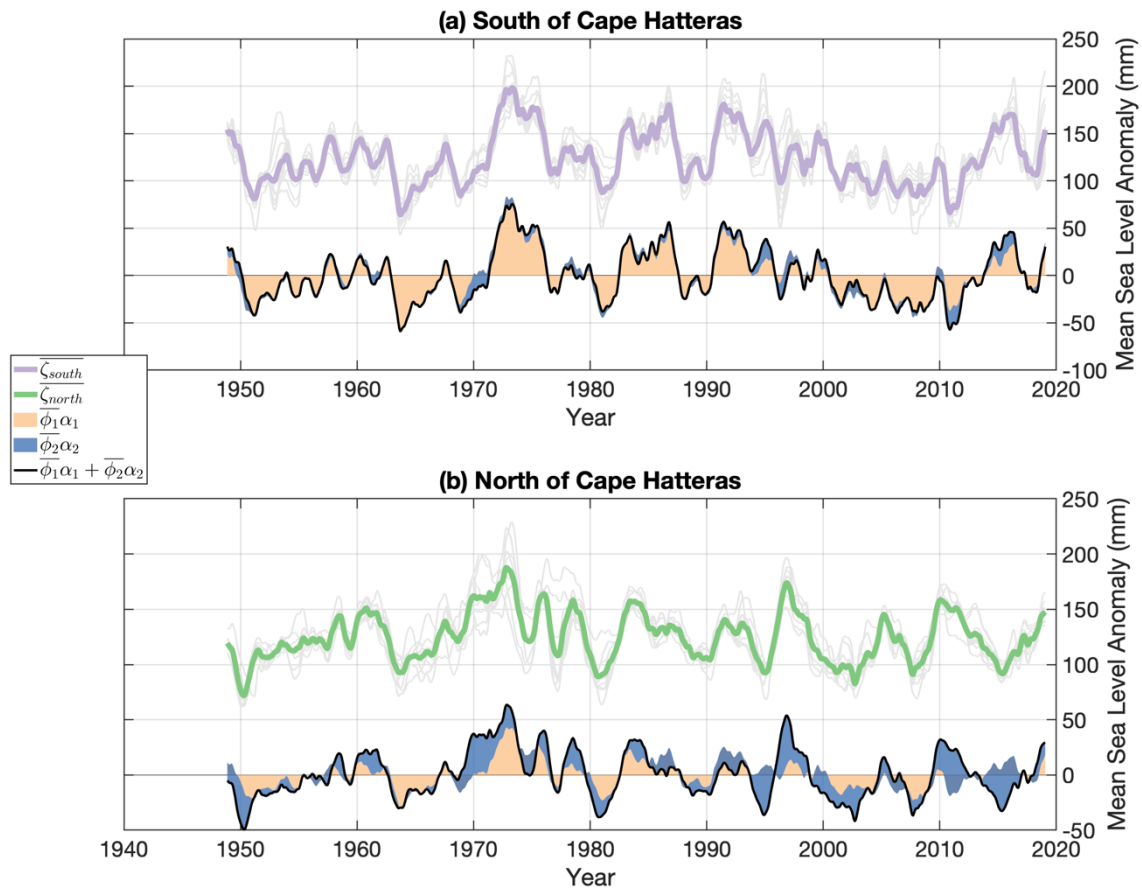
Figure 2 – (a) Mean of the sea level south of Cape Hatteras (thick violet line), together with reconstructed sea-level from the EOF modes 1 and 2 (orange and blue shades). (b) As for (a), but with the sea level north of Cape Hatteras. Mean of the sea level north of Cape Hatteras is in green.
