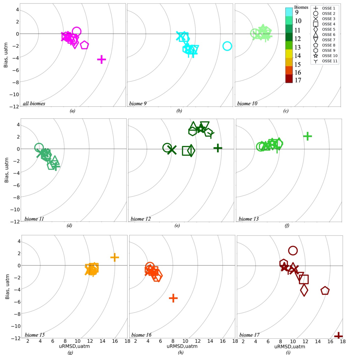
Figure 4: Target Diagram per biome for 11 OSSEs, the colour code corresponds to Fig. 2, the purple colour represents the whole of the 8 biomes: (a) - all 8 biomes, (b) - biome 9 (Subpolar seasonally stratified North Atlantic), (c) - biome 10 (Subtropical seasonally stratified North Atlantic), (d) - biome 11 (Subtropical permanently stratified North Atlantic), (e) - biome 12 (Equatorial Atlantic), (f) - biome 13 (Subtropical permanently stratified South Atlantic), (g) - biome 15 (Subtropical seasonally stratified Southern Ocean), (h) - biome 16 (Subpolar seasonally stratified Southern Ocean), (i) - biome 17 (Southern Ocean ice). OSSE 1: SOCAT data only; OSSE 2: synthetic Argo data only; OSSE 3: SOCAT and synthetic Argo data; OSSE 4: SOCAT data and 25% of original synthetic Argo data; OSSE 5: SOCAT data and 10% of original synthetic Argo data; OSSE 6: SOCAT data and synthetic Argo data in the Southern Hemisphere; OSSE 7: SOCAT data and 25% of original synthetic Argo data in the Southern Hemisphere; OSSE 8: SOCAT data and 10% of original synthetic Argo data in the Southern Hemisphere; OSSE 9: SOCAT data, synthetic Argo data in the Southern Hemisphere and data from mooring stations; OSSE 10: SOCAT data, 25% of original synthetic Argo data in the Southern Hemisphere and data from mooring stations; OSSE 11: SOCAT data, 10% of original synthetic Argo data in the Southern Hemisphere and data from mooring stations. OSSEs 1, 3 and 10 are in bold as we focus our detailed comparison on these three OSSEs.
