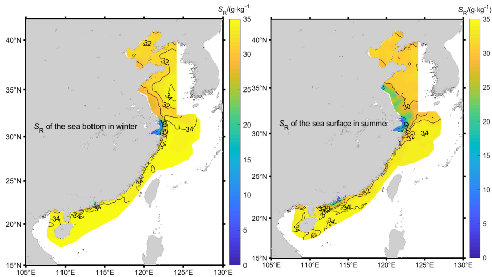
Fig. 2 S_R isoclines of China offshore seawater
