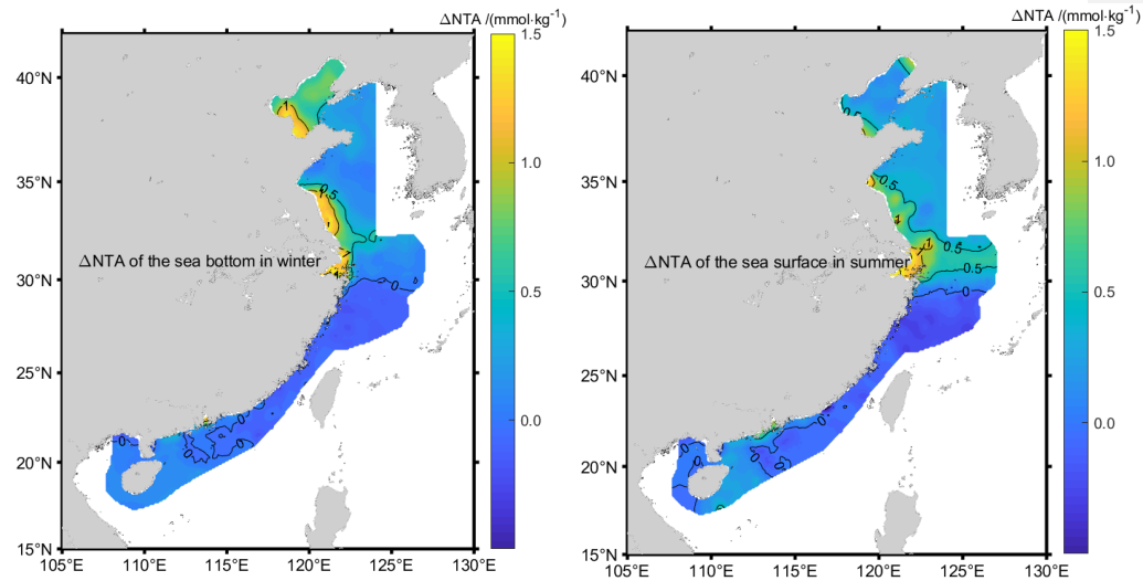
Fig.4 \Delta[\text{NTA}] isoclines of China offshore seawater
