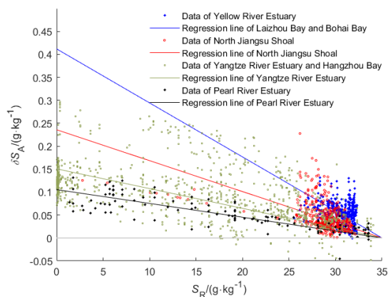
Fig.5 The Absolute Salinity Anomaly of the four regions of China offshore as a function of their Reference Salinity
