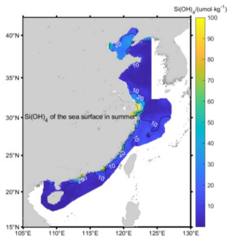
Fig.6 \text{Si(OH)}_4 isoclines of sea surface in summer
