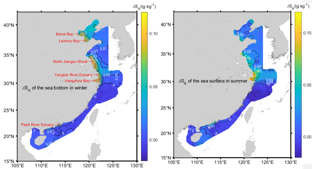
Fig.3 \delta S_A isoclines of Chinese offshore seawater. Hatched areas at left represent Salinity Anomalies more than 0.05 \text{ g} \cdot \text{kg}^{-1} .
