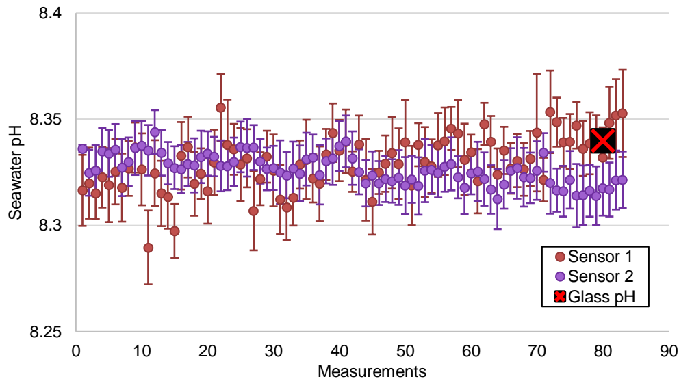
Figure 5: Representation of pH values obtained by two sensors in synthetic seawater at a constant temperature, compared with the pH measured by a glass pH probe. Each measurement corresponds to the average of twelve pH measurements over five minutes testing.
