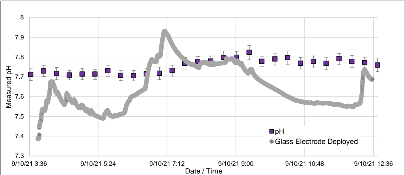
Figure 9: A plot of pH as a function of time for the sensors deployed in Ardmucknish Bay for both the calibration free pH sensor and an oceanographic glass-based pH sensor.
