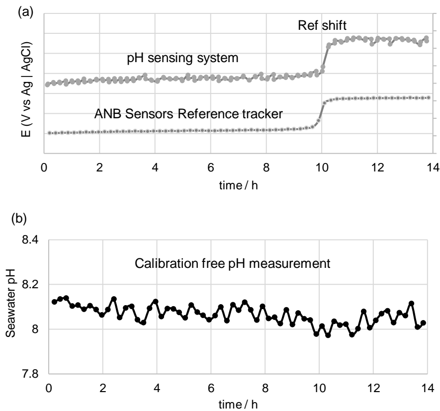
145 Figure 4: (a) The plot of peak potential for the reference tracking and pH sensing elements as a function of time. (b) The final calibration free pH sensor output as a function of time.
