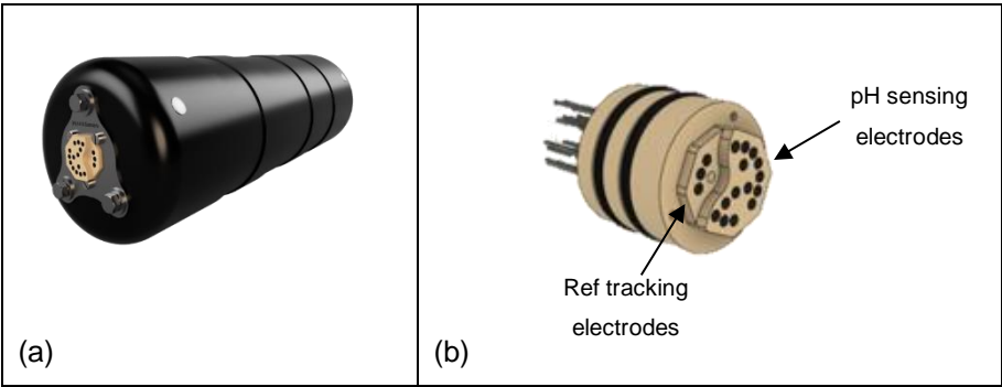
95 Figure 2: (a) The mechanical housing of the sensor including the transducer. (b) An image of the transducer depicting the recessed reference tracking electrodes and the pH sensing electrodes on the front face.
