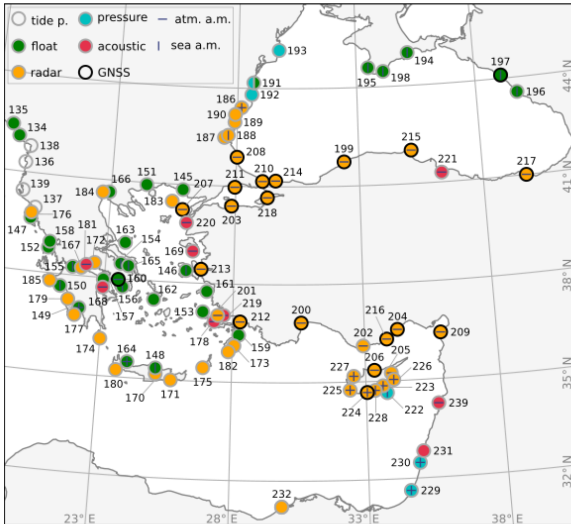
720 Figure 6: Same as in Figure 4, but for the Eastern Mediterranean Sea and for the Black Sea. Station names are listed in the Appendix tables: Tables A13 -- A14, Tables A16 -- A25, and Table A27. Stations 137, 152, 156, 165, 168, 170, 172, 178, 205 and 222 are slightly shifted to assure better visibility.
