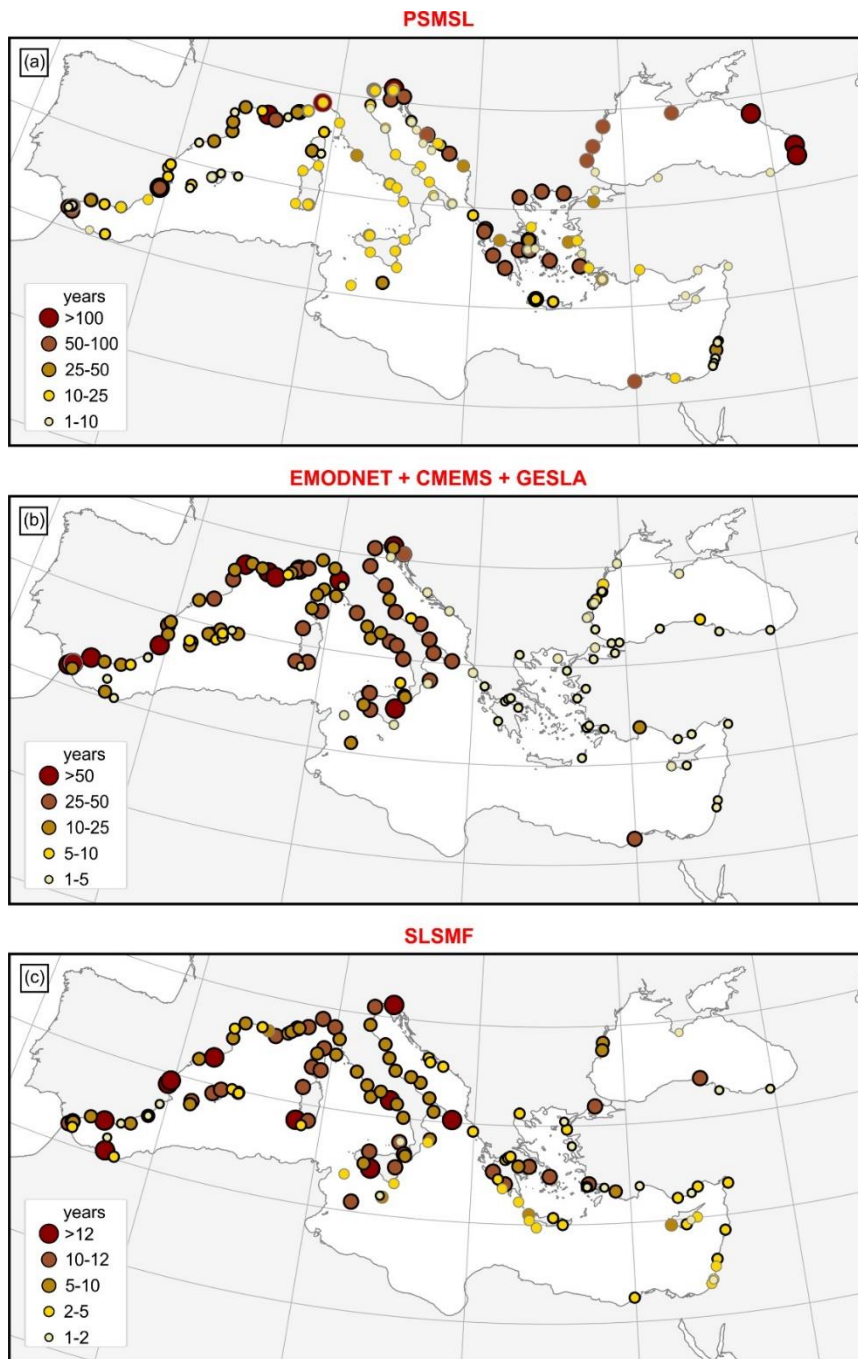
835 Figure 8. The Mediterranean and Black Sea data accessible as: (a) monthly sea level averages in the PSMSL (the length of series is indicated by the size and colour of the circle; thick border lines denote the series that end in 2018 or later, and grey the series that end earlier), (b) hourly sea level data in either EMODnet Physics, Copernicus Marine Service and GESLA (the length of series is indicated by the size and colour of the circle; thick and grey lines denote the series that do or do not, contain the data in 2021, respectively), and (c) minute series in the IOC-SLSMF (the length of the operability period is indicated by the size and the colour of the circle; thick and grey border lines denote the stations that were or were not, operational on 15 November 2021, respectively).
