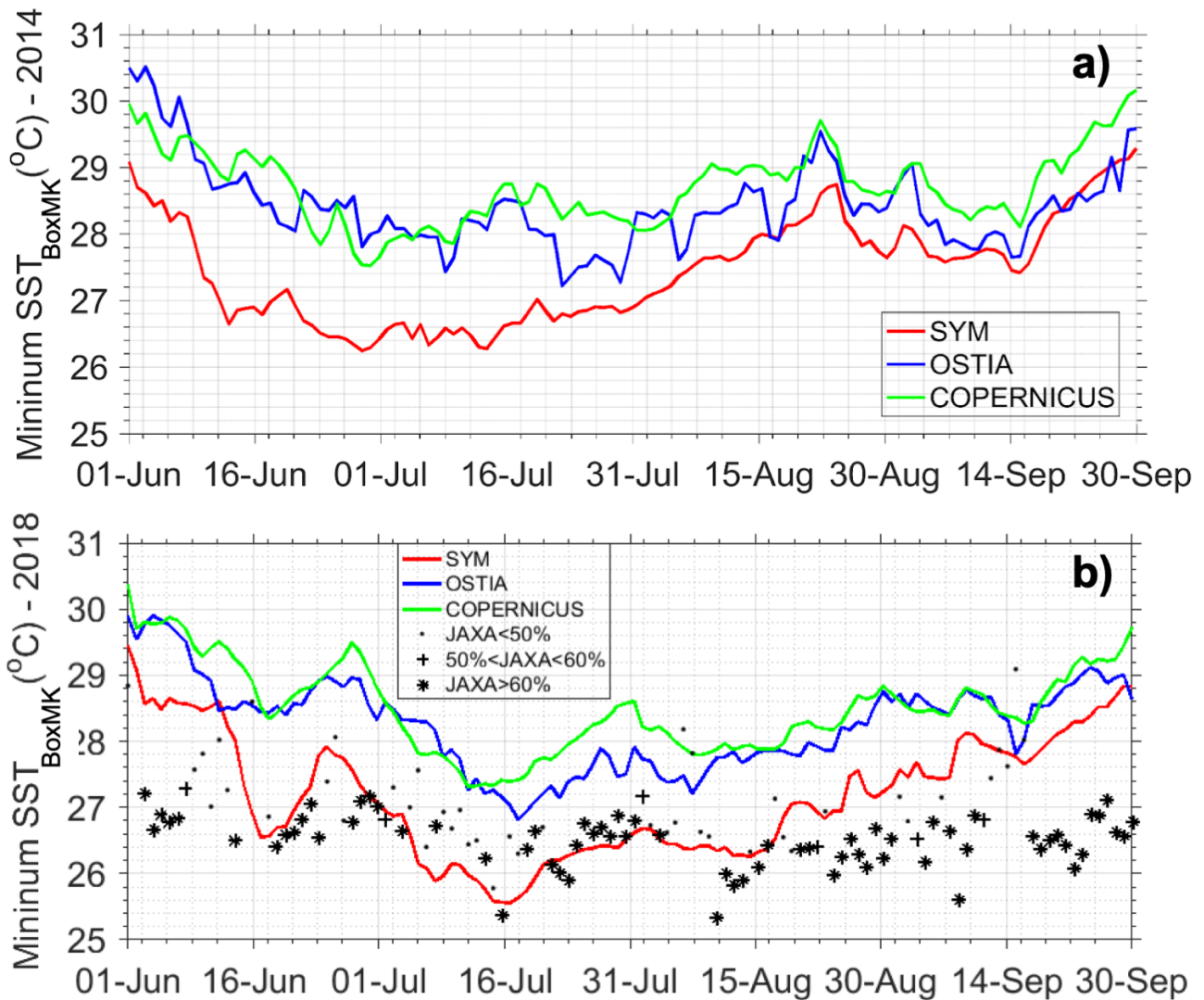
1165 Figure 5: Daily time series of minimum SST ( ^{\circ}\text{C} ) over BoxMK (a) during summer 2014 in SYMPHONIE, OSTIA, COPERNICUS, and (b) during summer 2018 in SYMPHONIE, OSTIA, COPERNICUS and JAXA. Dots, crosses and stars correspond respectively to a spatial coverage of BoxMK lower than 50%, higher than 50%, and higher 60% for JAXA. We only consider JAXA pixels of quality levels \geq 4 .
