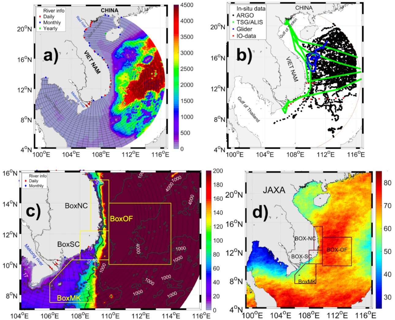
1110 Figure 1. (a) Characteristics of the orthogonal curvilinear computational grid (black lines, not all points are shown for 1111 visibility purposes) and bathymetry (colors, m, GEBCO_2014 ) used for the VNC configuration of the SYMPHONIE model. Dots show the location of rivers for which we used daily (red), monthly (blue) and yearly climatology (green) discharge values. (b) Location of in-situ data available over the VNC domain: ARGO buoys (black), ALIS R/V campaign (TSG: green), IO-18 data (red), and glider data (blue). (c) Bathymetry (m) over the SVU region. Yellow boxes show the 1115 location of the 4 boxes used for the study of SVU. (d) Percentage of days during which JAXA data are available during summer 2018.
