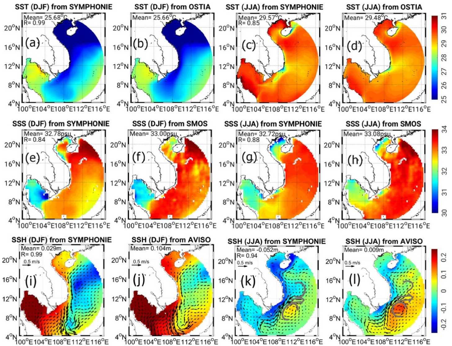
1130 Figure 2: Spatial distribution of simulated and observed winter (DJF) and summer (JJA) climatological averages of SST (a,b,c,d, °C), SSS (e, f, g, h), SSH (i,j,k,l, m) and total surface geostrophic current ( \text{m}\cdot\text{s}^{-1} ), and spatial correlation coefficient R (here the p-value is always smaller than 0.01). Grey arrows on panels k-l highlight the summer AC/C dipole and eastward jetmet.
