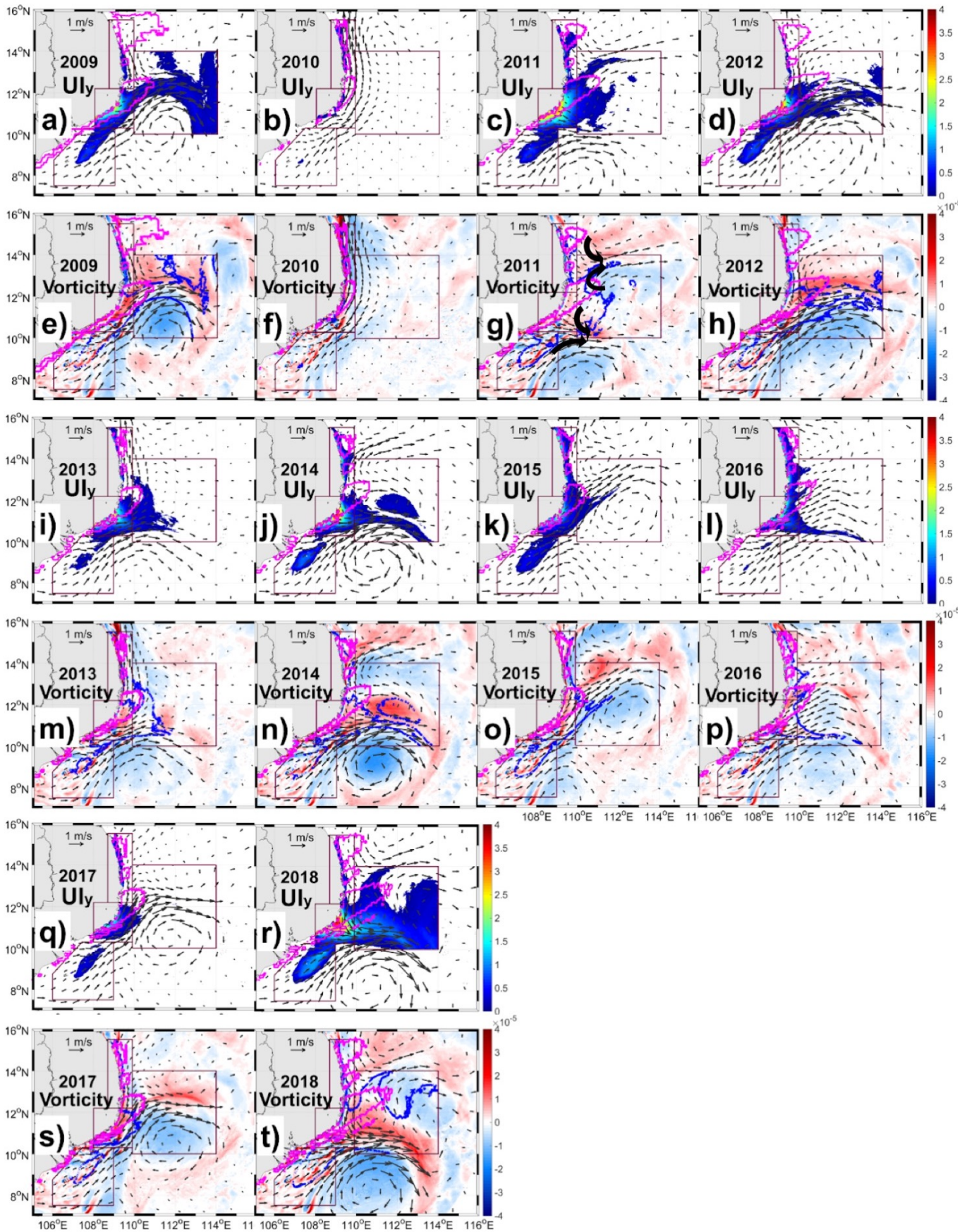
1225 Figure 12: Maps of spatial yearly upwelling index UI_y ( ^{\circ}C , a,b,c,d,i,j,k,l,q,r) and of speed and direction (arrows, m \cdot s^{-1} ) and vorticity (colors, s^{-1} ) of JJAS averaged surface current (e,f,g,h,m,n,o,p,s,t) for each year of the simulation. Pink contours show the +3 \cdot 10^{-7} N \cdot m^{-3} isoline of JJAS average positive wind stress curl. Blue contours show the 0.1^{\circ}C isoline of UI_y .
