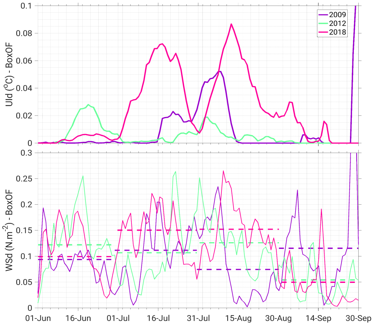
1260 Figure 15: Same as Figure 9 for BoxOF and years 2009 (purple), 2012 (green) and 2018 (magenta). For the sake of readability, the y-axis is cut off for the last extreme value of September 2009, which corresponds to the passage of storm KETSANA over the SVU region (see the NOAA storm track website on https://coast.noaa.gov/hurricanes ).
