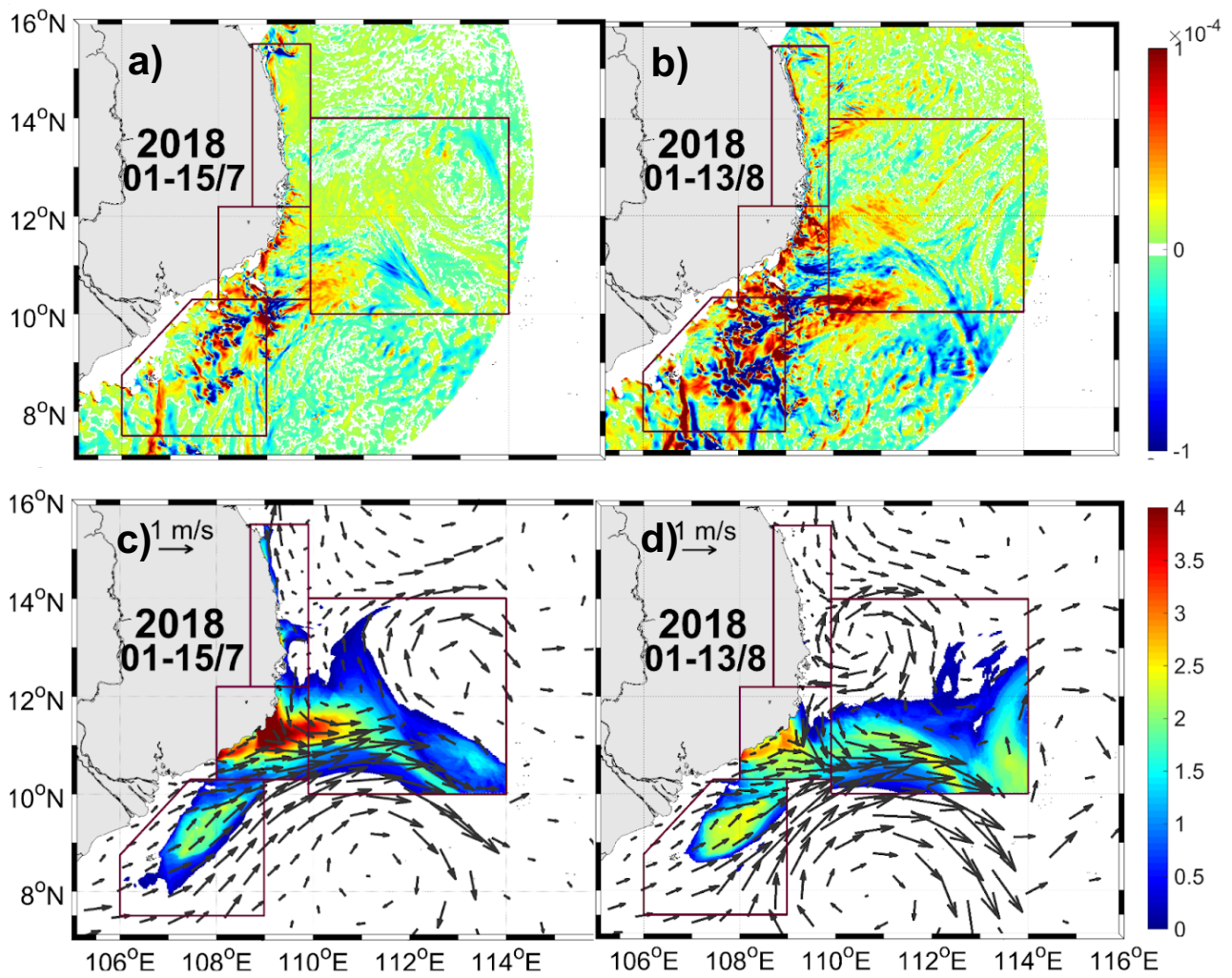
Figure 18 : Vertical velocity ( \text{m}\cdot\text{s}^{-1} , 1 st row) and daily upwelling index ( ^{\circ}\text{C} , 2 nd row) and surface currents ( \text{m}\cdot\text{s}^{-1} ) averaged over the July (a,c) and August (b,d) periods of upwelling development in summer 2018.
