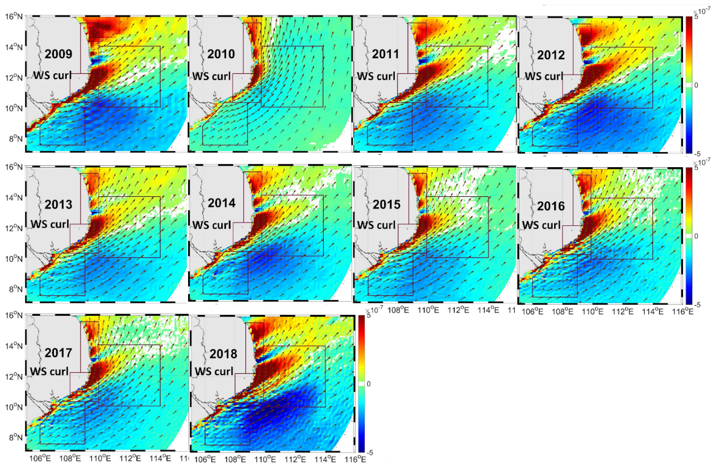
Figure 11: Maps of JJAS averaged wind stress (arrows, \text{N}\cdot\text{m}^{-2} ) and wind stress curl (colors, \text{N}\cdot\text{m}^{-3} ) for each year of the 1220 simulation.
