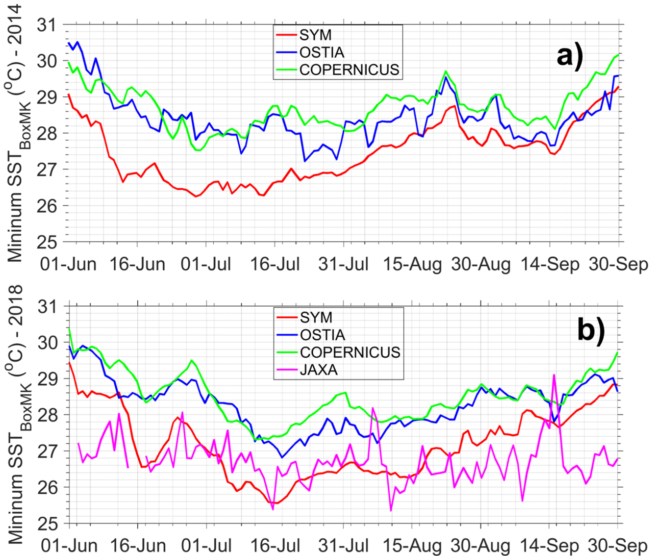
1080 Figure 5: Daily time series of minimum SST (°C) over BoxMK (a) during summer 2014 in SYMPHONIE, OSTIA, COPERNICUS, and (b) during summer 2018 in SYMPHONIE, OSTIA, COPERNICUS and JAXA.
