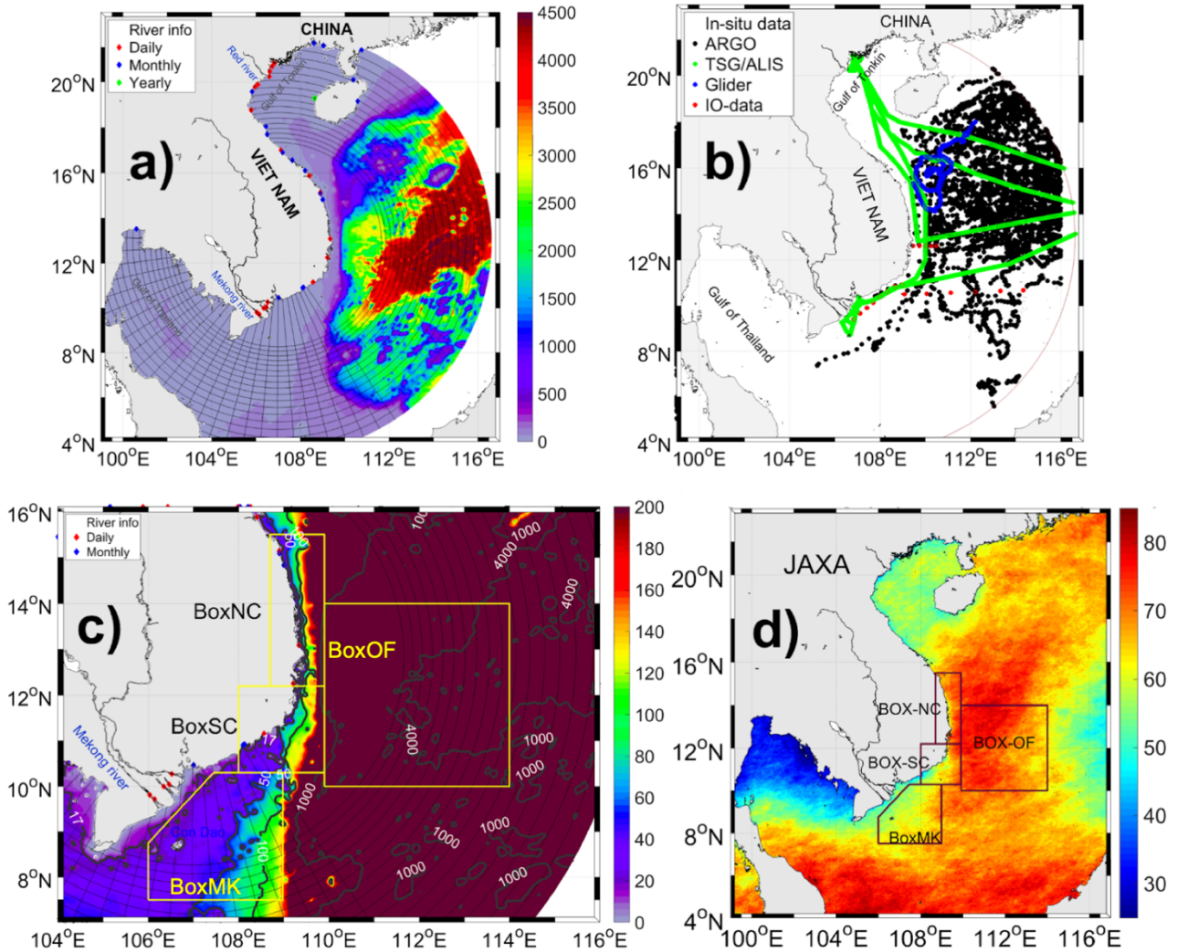
1025 Figure 1. (a) Characteristics of the orthogonal curvilinear computational grid (black lines, not all points are shown for visibility purposes) and bathymetry (colors, m, GEBCO_2014 ) used for the VNC configuration of the SYMPHONIE model. Dots show the location of rivers for which we used daily (red), monthly (blue) and yearly climatology (green) discharge values. (b) Location of in-situ data available over the VNC domain: ARGO buoys (black), ALIS R/V campaign (TSG: green), IO-18 data (red), and glider data (blue). (c) Bathymetry (m) over the SVU region. Yellow boxes show the location of the 4 boxes used for the study of SVU. (d) Percentage of days during 1030 which JAXA data are available during summer 2018.
