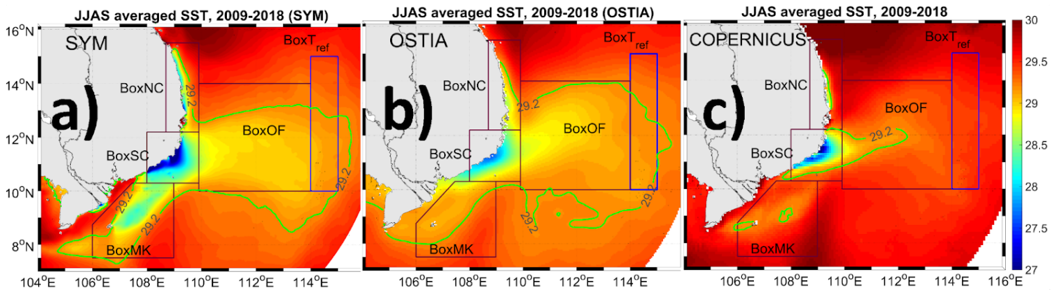
1055 Figure 3: JJAS average over 2009-2018 of SST (°C) from (a) SYMPHONIE, (b) OSTIA and (c) COPENICUS over the SVU region. Black boxes show the 4 upwelling areas, and the blue rectangles shows the reference box. Coordinates of the boxes : BoxNC (12.2-15.5°N; 108.7-109.9°E), BoxSC (10.3-12.2°N; 108-109.9°E), BoxOF (10-14°N; 109.9-114°E), BoxMK (at depth > 17m, 7.5-10.3°N; 106-109°E). BoxT Ref (10-15°N; 114-115°E)
