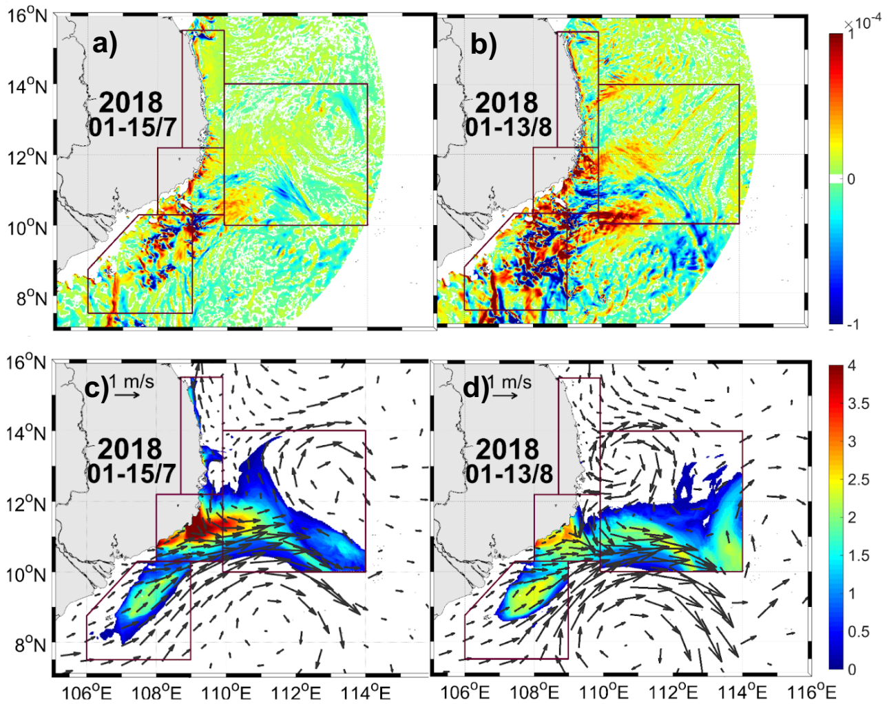
1195 Figure 17 : Vertical velocity ( \text{m}\cdot\text{s}^{-1} , 1 st row) and daily upwelling index ( ^{\circ}\text{C} , 2 nd row) and surface currents ( \text{m}\cdot\text{s}^{-1} ) averaged over the July (a,c) and August (b,d) periods of upwelling development in summer 2018.
