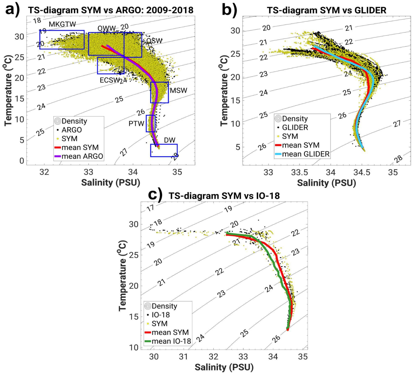
1105 Figure 8: TS-diagram built from observations from (a) ARGO (black dots and purple line for dots average), (b) GLIDER (black dots, cyan line), (c) IO-18 (black dots, green line), and from SYMPHONIE colocalized outputs (yellow dots, red line). Blue rectangles represent water masses in the SCS (Uu and Brankard 1997, Dippner et al. 2011) : MKGTW (Mekong & Gulf of Thailand Water), OWW (Offshore Warm Water), OSW (Offshore Salty Water), ECSW (East China Sea Water), MSW (Maximum Salinity Water), PTW (Permanent 1110 Thermocline Water), DW (Deep Water).
