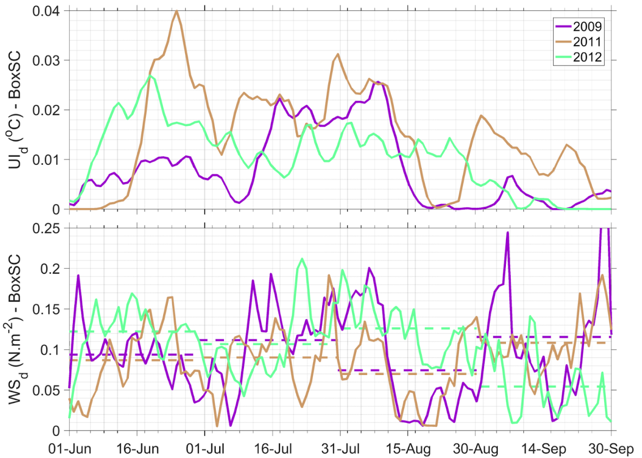
1160 Figure 14: Time series of daily upwelling index (top) and average daily (plain line) and monthly (dashed line) wind stress (bottom) over BoxSC between June and September for years 2009 (purple), 2011 (orange) and 2012 (green). For the sake of readability, the y-axis is cut off for the last extreme value of September 2009, which corresponds to the passage of storm KETSANA over the SVU region (see the NOAA storm track website on https://coast.noaa.gov/hurricanes ).
