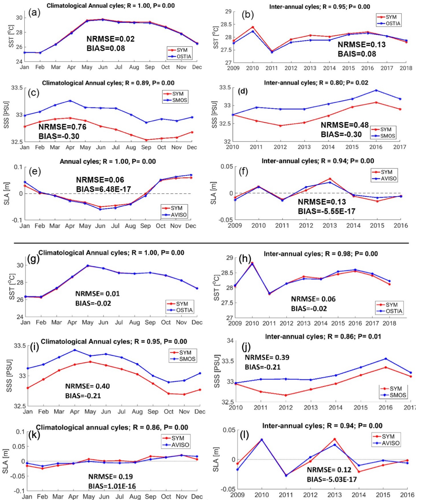
1095 Figure 7: Climatological monthly time series (left) and interannual yearly time series (right) of simulated (red) and observed (blue) SST (°C), SSS and SLA (m) averaged over (a to f) the VNC domain and over (g to l) the SVU area (104-116°E; 7-16°N). Correlation (correlation coefficient R and p-value P), NRMSE and bias of simulated vs. observed values are indicated.
