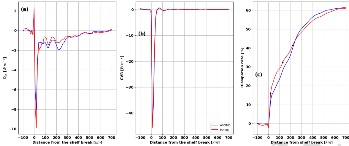
Figure 8. (a) D_{bc} (units: W m^{-2} ), (b) CVR (units: W m^{-2} ), and (c) dissipation rate (%) as a function of distance from the continental shelf break. CVR and D_{bc} are integrated every 10 km from the shelf break. The dissipation rate is the ratio between the cumulative sum of D_{bc} and the sum of CVR within the first 50 km from the shelf break. ASOND is in blue and MAMJJ is in red. The black stars are the locations of the three peaks of maximum dissipation.
