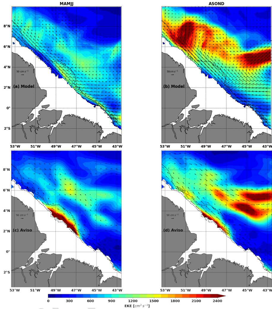
Figure 3. (a, b) Model mean surface EKE (colours, units: \text{cm}^2 \text{s}^{-2} ) and current (arrows, units: \text{cm s}^{-1} ) during (a) MAMJJ and (b) ASOND. (c, d) AVISO mean surface EKE during (c) MAMJJ and (d) ASOND. Dashed black contours are 100 and 2000 m isobaths. Bathymetry less than 100 m is masked.
