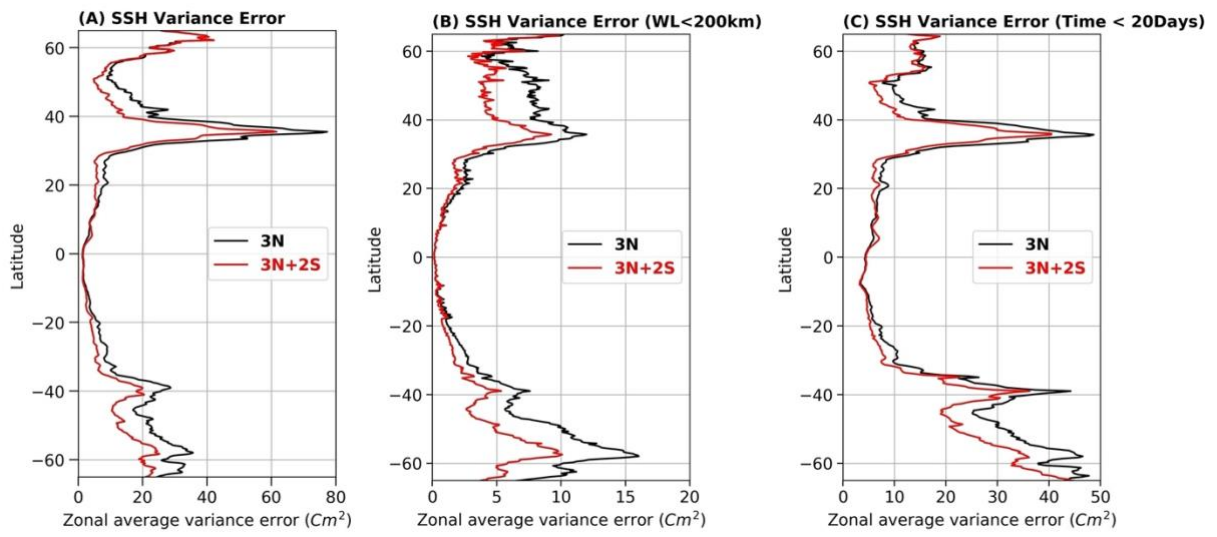
3 Figure 9: The zonal SSH averaged error variance: (A) for full scales, (B) for scales less than 200 km and (C) for time scales 4 less than 20 days; assimilation of 3N (black lines) and assimilation of 3N+2S (red lines). Units are \text{cm}^2
