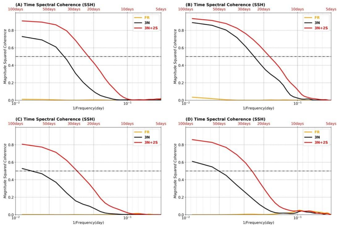
2 Figure 12: Time spectral coherence with respect to the NR (Wavelengths < 500km), (A) low-latitude region (red box), (B) 3 Agulhas current (orange box), (C) North Atlantic (high-latitude, green box) and (D) North Atlantic Drift current (black box).
