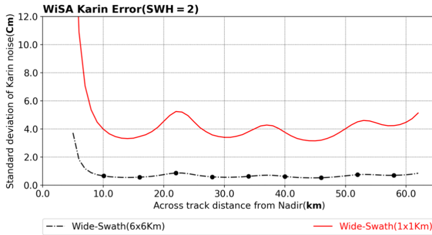
3 Figure 1: The curves displayed show the wide-swath instrumental error with SWH=2m (wave height), considering 4 across-swath horizontal resolution of 1 km (solid red line) and 6 km (dash black line).
