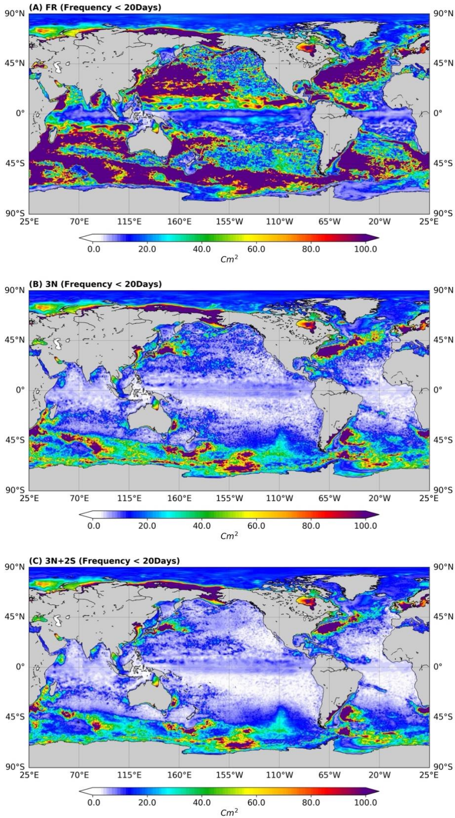
2 Figure 8: Global maps of SSH analysis error (NR – Model Analysis; Time scales < 20Days) variance (in cm^2 , 2015). (A) Free 3 Run (FR); (B) With 3 nadir (3N); (C) with 3 nadir and two Wide-Swath (3N+2S).
