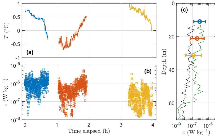
Figure 8. Overview of dissipation rates. Time series of a) temperature and b) final estimate of the dissipation rate. c) Vertical profiles (black and green) of \epsilon measured by the vertical microstructure profiler at two co-located stations marked by stars in Fig. 1b. Mean value and the lower and upper limits (95% confidence intervals) of the natural logarithm of the AUV-MR measurement are shown at their corresponding average depth in (c). Blue, red and yellow corresponds to 11, 21 and 31 m depth respectively.
