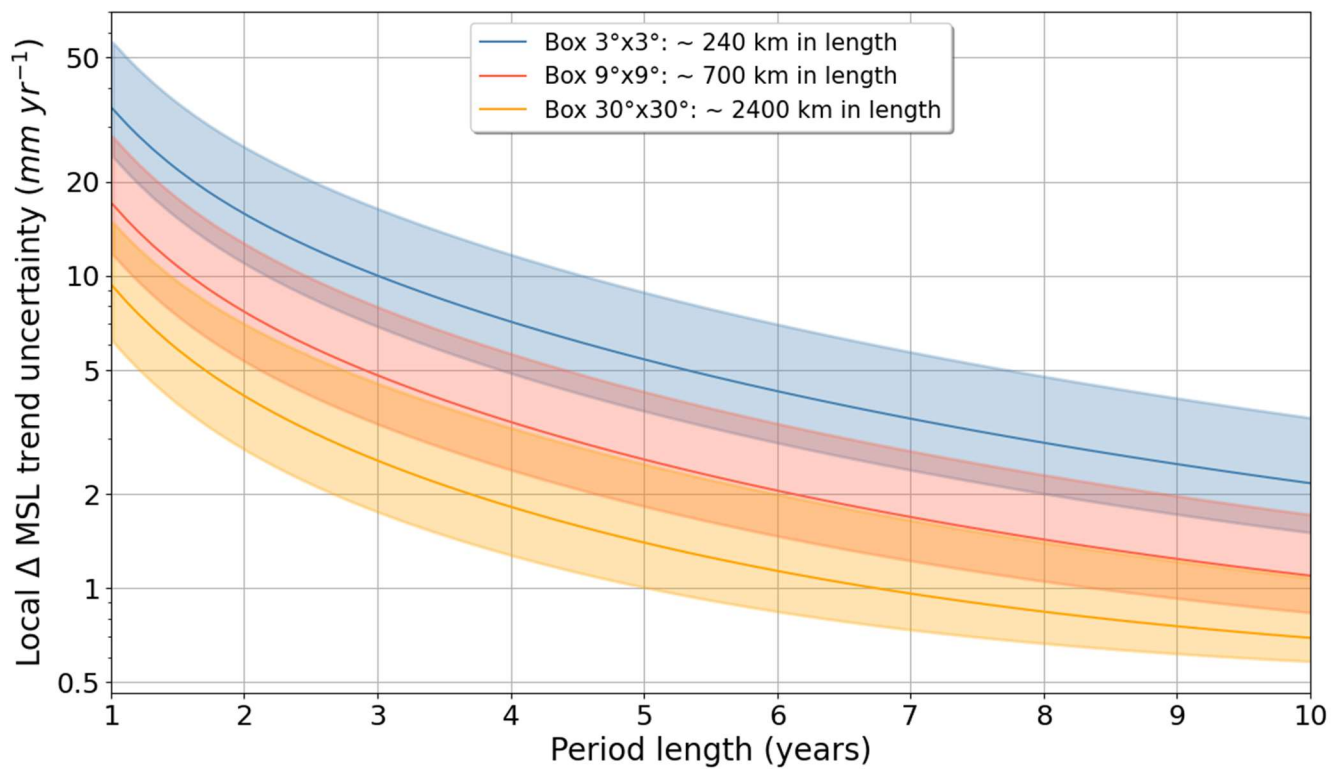
Figure 6: Evolution of the S3A - Jason-3 regional \Delta MSL trend uncertainties as a function of period length for different box sizes. The solid line is the global median of regional \Delta MSL trend uncertainties. The envelope represents the spatial distribution of uncertainties at between the 16th and 84th percentile (i.e. 1-sigma) values. Y-axis scale is logarithmic.
