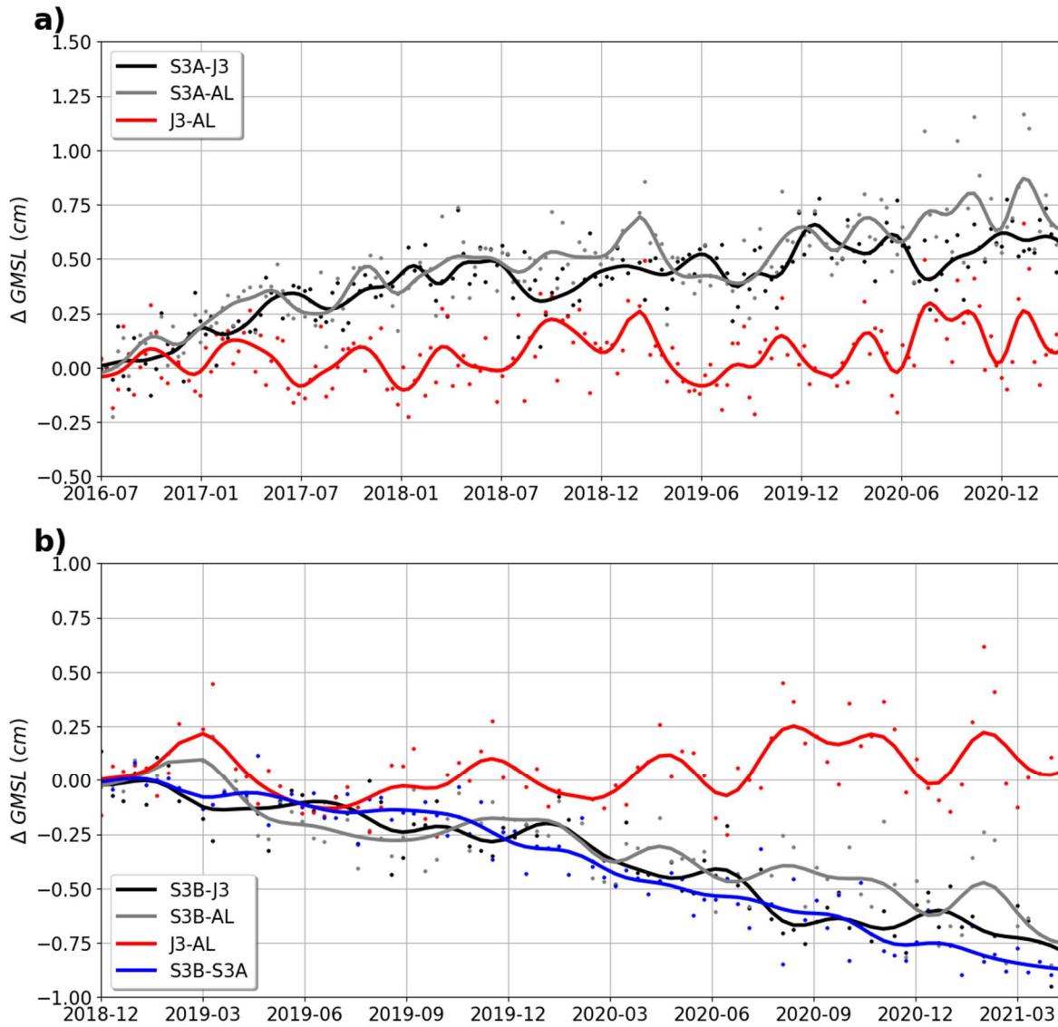
Figure 1: Evolution of \Delta GMSL: a) over the S3A period between S3A and Jason-3, S3A and SARAL/AltiKa, Jason-3 and SARAL/AltiKa; b) over the S3B period between S3B and S3A, S3B and Jason-3, S3B and SARAL/AltiKa, Jason-3 and SARAL/AltiKa. The dotted curves are the raw time series sampled at 10-days. The solid lines are time series filtered at 3 months with a low pass filter. Each time series is artificially set to 0 at its origin.
