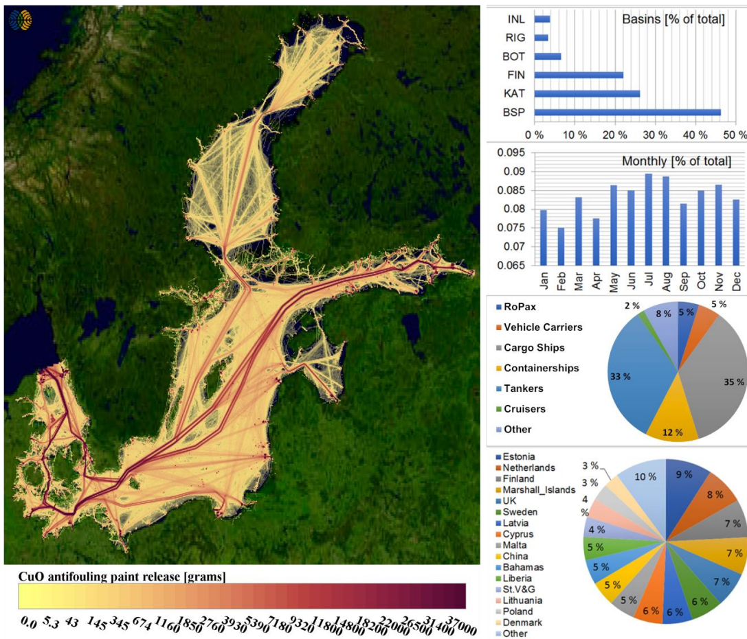
Figure 9 Geographical distribution of the emissions of Cu(I)O from ship hull antifouling paints. The values reported by the colour scale indicate CuO releases in unit of grams per map grid cell of 5 km 2 . Top right bar chart indicates the share of Cu(I)O releases by sea area (INL=Inland areas, RIG=Gulf of Riga, BOT=Bothnian Sea and Bothnian Bay, FIN=Gulf of Finland, KAT=Kattegat, BSP=Baltic Proper). Lower bar chart describes the monthly variation of CuO releases. Upper pie chart illustrates the estimated share various ship types and the lower pie chart the flag state contributions to CuO releases. Map background Landsat-8 image courtesy of the U.S. Geological Survey.
