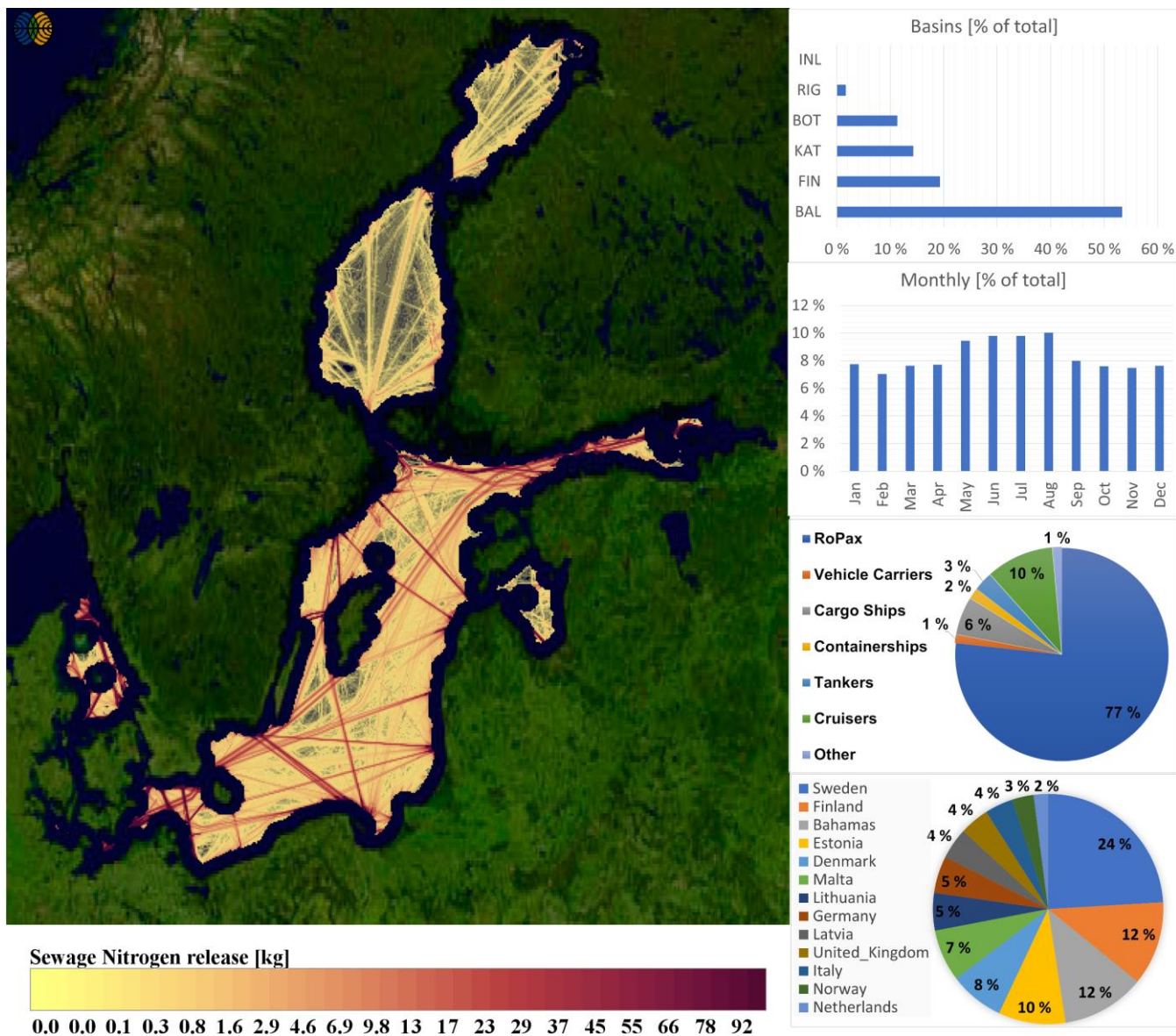
735 Figure 11 Sewage nitrogen discharges from ships during 2012 in unit of kilograms per map grid cell area of 5 km 2 . According to IMO rules, no discharge is allowed closer than 12 nm distance from the coastline. Upper bar chart describes the contributions by sub-basin, lower bar chart the monthly variation. Upper pie chart depicts the ship type and lower pie chart the flag state contributions to sewage nitrogen releases. Map background Landsat-8 image courtesy of the U.S. Geological Survey.
