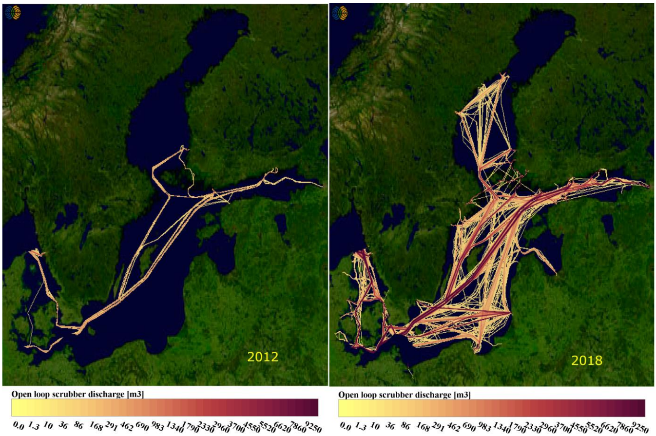
575 Figure 5 Annual discharge of effluent from open loop scrubbers during 2012 (left) and 2018 (right). Both images describe the discharge in units of cubic metres per map grid cell of 5 km 2 . A significant increase in open loop scrubber effluent release was predicted based on the activity of scrubber-enabled vessels. Map background Landsat-8 image courtesy of the U.S. Geological Survey.
