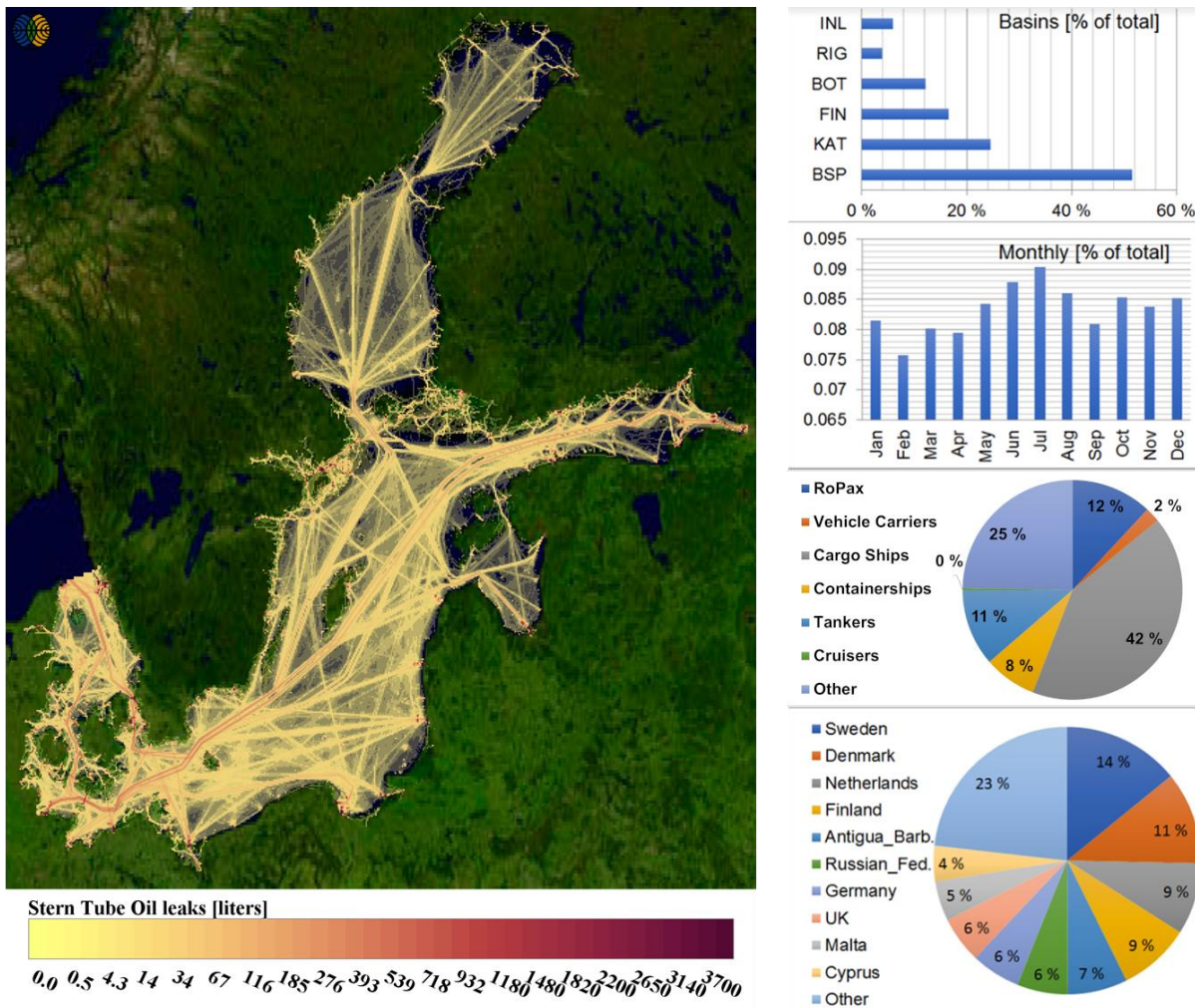
550 Figure 4 Distribution of the annual stern tube oil releases for year 2012 from the Baltic Sea shipping. Discharge volumes are indicated in litres per map grid area of 5 km 2 . Top right: Share of stern tube oil released in various sub-basins of the Baltic Sea (INL=Inland areas, RIG=Gulf of Riga, BOT=Bothnian Bay and Bothnian Sea, FIN=Gulf of Finland, KAT=Kattegat, BSP=Baltic Sea Proper). Lower bar chart depicts the monthly variation of stern tube oil discharges. Upper pie chart summarizes the contribution of various ship types to stern tube oil releases and the lower pie chart the flag state shares of stern tube oil releases. Map background Landsat-8 image courtesy of the U.S. Geological Survey.
