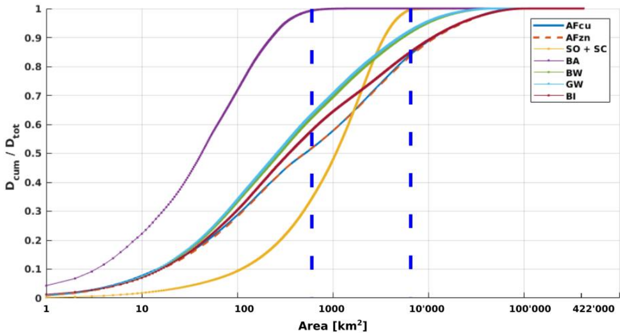
755 Figure 12: The cumulative discharges over the area of the Baltic Sea divided by the total discharges for the year 2012. Vertical blue dashed lines correspond to the areas of total load of the ballast water and scrubber water discharges. AFCu=Antifouling paint release CuO, AFzn=Antifouling paint release ZnO, SO+SC=Scrubber effluent release both from open and closed loop systems, BA=Ballast water discharge, BW=Sewage release, GW=Grey water discharge, BI=Bilge water release.
