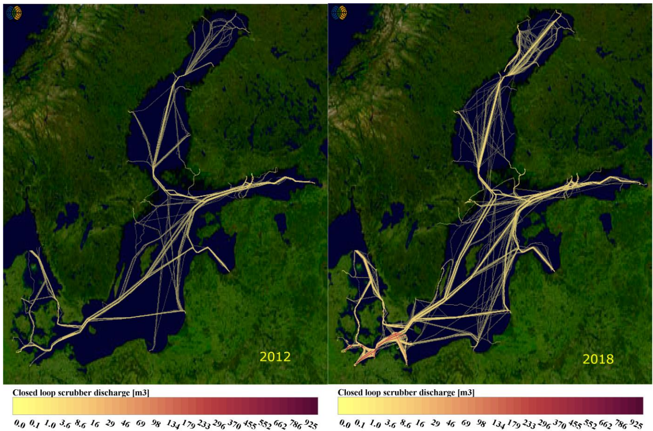
580 Figure 6 Discharge of scrubber effluent from closed loop systems during 2012 (left) and 2018 (right). The values for discharges are reported in units of cubic meters for each map grid cell of 5 km 2 . Map background Landsat-8 image courtesy of the U.S. Geological Survey.
