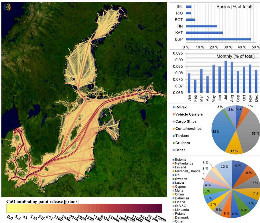
680 Figure 9 Geographical distribution of the emissions of Cu(I)O from ship hull antifouling paints. The values reported by the color scale indicate CuO releases in unit of grams per map grid cell of 5 km 2 . Top right bar chart indicates the share of Cu(I)O releases by sea area (INL=Inland areas, RIG=Gulf of Riga, BOT=Bothnian Sea and Bothnian Bay, FIN=Gulf of Finland, KAT=Kattegat, BSP=Baltic Proper). Lower bar chart describes the monthly variation of CuO releases. Upper pie chart illustrates the estimated share various ship types and the lower pie chart the flag state contributions to CuO releases. Map background Landsat-8 image courtesy of the U.S. Geological Survey.
