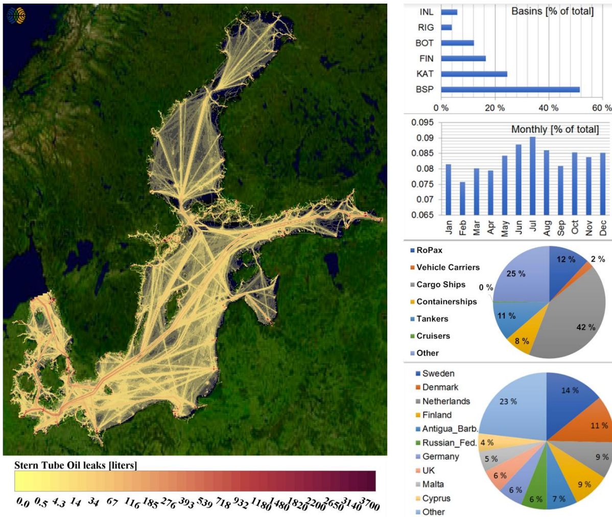
550 Figure 4 Distribution of the annual stern tube oil releases for year 2012 from the Baltic Sea shipping. Discharge volumes are indicated in liters per map grid area of 5 km 2 . Top right: Share of stern tube oil released in various sub-basins of the Baltic Sea (INL=Inland areas, RIG=Gulf of Riga, BOT=Bothnian Bay and Bothnian Sea, FIN=Gulf of Finland, KAT=Kattegat, BSP=Baltic Sea Proper). Lower bar chart depicts the monthly variation of stern tube oil discharges. Upper pie chart summarizes the contribution of various ship types to stern tube oil releases and the lower pie chart the flag state shares of stern tube oil releases. Map background Landsat-8 image courtesy of the U.S. Geological Survey.
