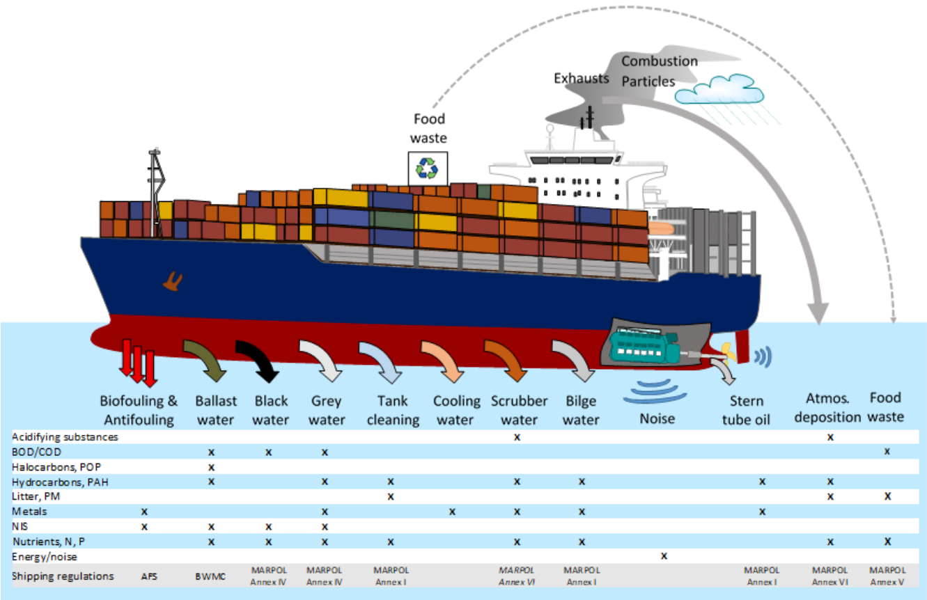
65 Figure 1: Waste streams from ships and the constituents in terms of stressors on the marine environment. These releases are regulated through several international conventions, like the IMO MARPOL, Antifouling (AFS) and Ballast Water Management Conventions (BWMC). Releases of excess energy (noise, heat, light) to the sea are not currently regulated.
