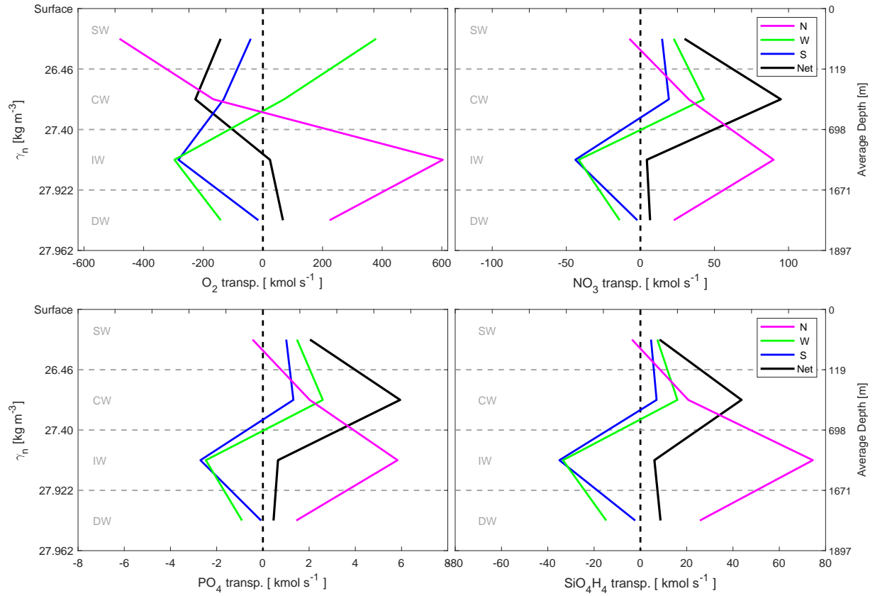
Figure A14. Mass ( \gamma_n ), O_2 , NO_3 , PO_4 and SiO_4H_4 transports ( kmol\ s^{-1} ) integrated per water types levels (SW, CW, IW and DW) at transects north (N, pink line), west (W, green line) and south (S, blue line) during FLUXES-I cruise and including WOA stations. Black line represents the net transport of each biochemical variable. See Tab. A2 to check O_2 , NO_3 , PO_4 and SiO_4H_4 transports values at each layer per transect. Negative/positive values indicate inward/outward transports as in Fig. A11.
