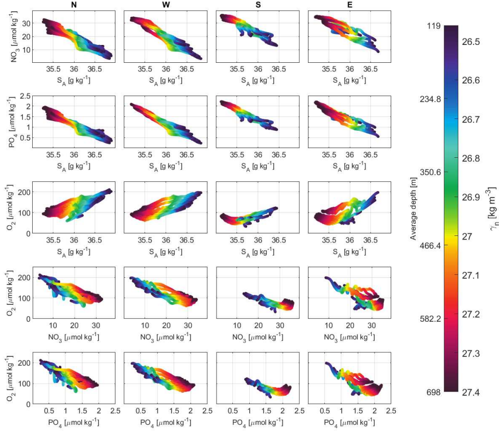
Figure A8. Scatter plots of in situ observations of \text{NO}_3 , \text{PO}_4 and \text{O}_2 ( \mu\text{mol kg}^{-1} ) with respect to S_A and \gamma_n (in colour with an approximate scale of the average depths) in transects north (N, first column), west (W, second column), south (S, third column) and east (E, fourth column) for CW layers in first, second and third line. In fourth and fifth lines, scatter plots of \text{NO}_3 - \text{O}_2 and \text{PO}_4 - \text{O}_2 in 4 transects and also for CW layers.
