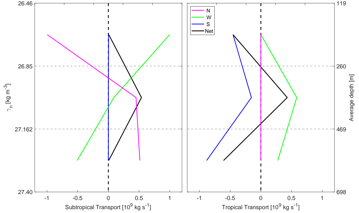
Figure A16. Mass transports ( 10^9 \text{ kg s}^{-1} ) integrated per transect at north (N, pink line), west (W, green line) and south (S, blue line) of the subtropical (left) and tropical (right) areas separated by the CVF at the three CW layers and considering transports between WOA stations. Black line represents the net transport. Negative/positive values indicate inward/outward transports as in Fig. A11.
