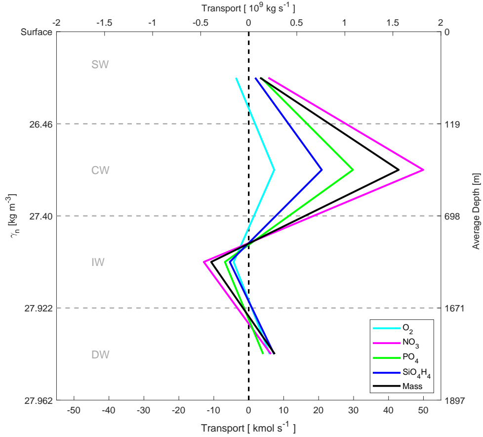
Figure A15. Mass ( 10^9 \text{ kg s}^{-1} ), \text{O}_2 , \text{NO}_3 , \text{PO}_4 and \text{SiO}_4\text{H}_4 transports ( \text{kmol s}^{-1} ) integrated per water types levels (SW, CW, IW and DW) through transect E during FLUXES-I cruise. Eastward transports were defined positive. The \text{O}_2/\text{PO}_4 transport is represented divided/multiplied by 10.
