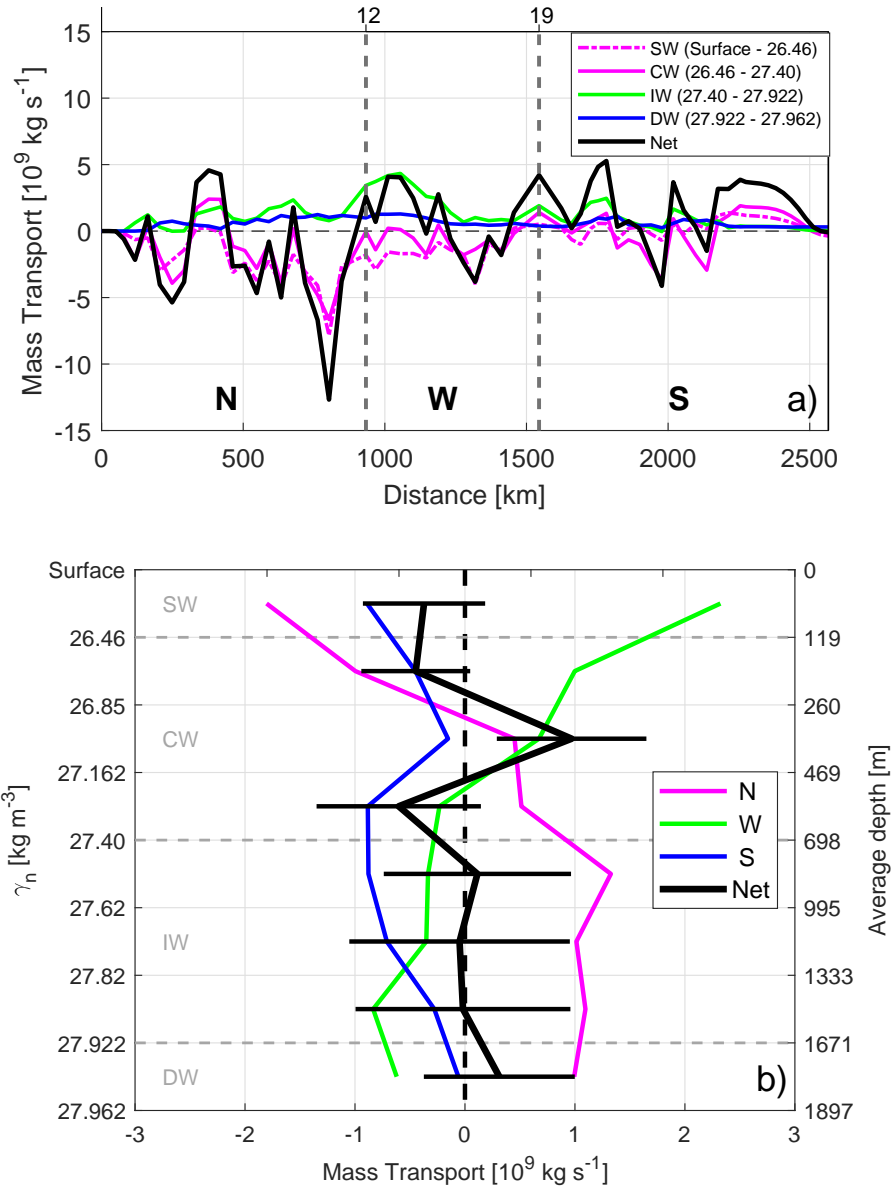
Figure A11. a) Accumulated mass transports per SW, CW, IW and DW levels and b) mass transports integrated per transect at north, west, and south, estimated by the inverse model during FLUXES-I cruise (including WOA stations in transects N and S). Negative/positive values indicate inward/outward transports in both plots. Mass conservation in the whole domain closed to coast is shown by the black line. The N/W and W/S corners are indicated with vertical dashed lines at stations 12 and 19 in the accumulated mass transports (a). The horizontal bars in each layer represented in the net mass transport are the errors estimated by the inverse model (b).
