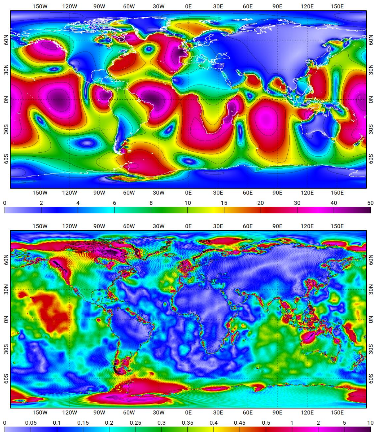
Figure 21: upper panel, M2 tidal loading, vertical displacement (cm); lower panel, M2 tidal loading vector difference between FES2014b and GOT4.10 (cm). Wave-like patterns visible in some regions are likely due to differences between Green's functions based computation of LSA (as in FES2014-derived atlas) and spherical harmonics based computation (GOT).
