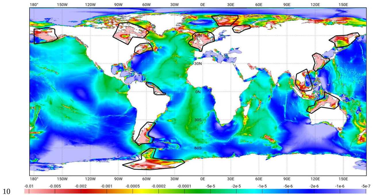
Figure 6: Energy ( \text{W/m}^2 ) dissipated by bottom friction in the FES2014 hydrodynamic model, for the M2 wave, and polygons used for the perturbations of the bottom friction coefficient.
