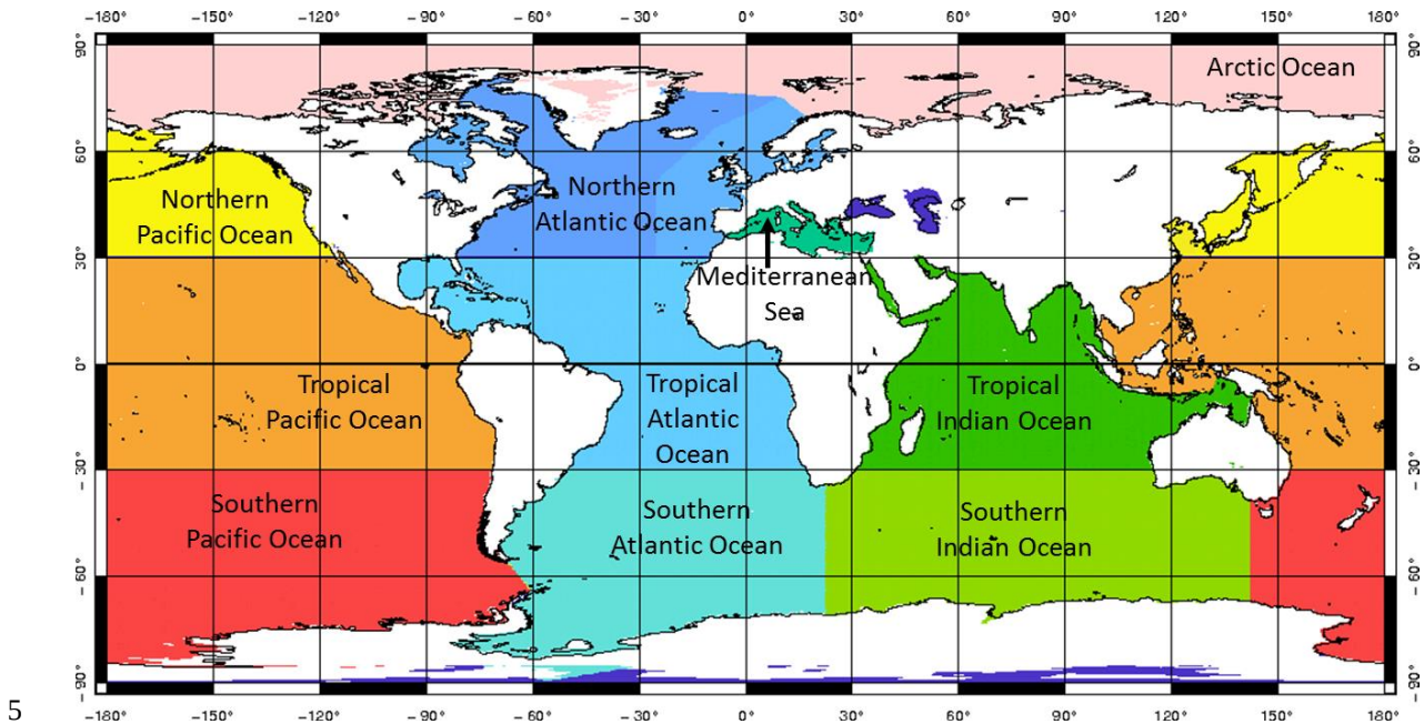
Figure 7: Divisions used for the perturbations of the wave drag coefficient.
